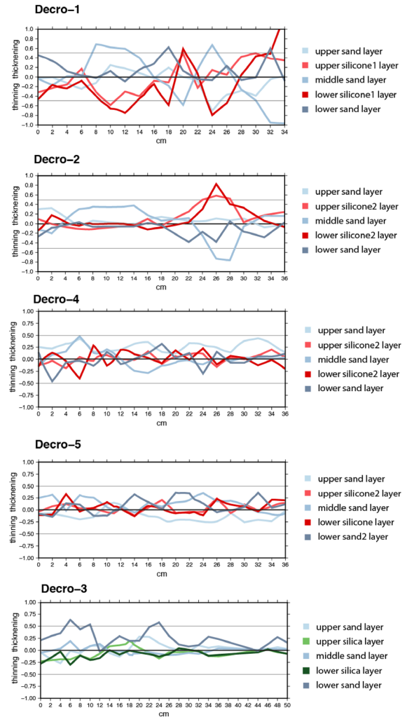
Figure 4. Variations in thicknesses of the five layers along the velocity discontinuity in each experiment. Note the wavelength for the thickness that is in opposite shift.
