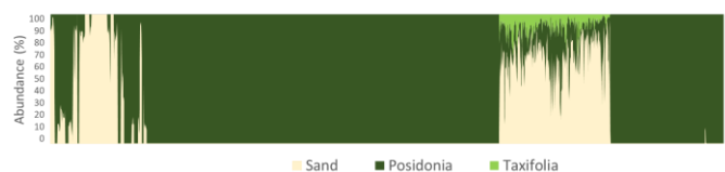
Fig. 5. Proportion of each class composing the seabed, namely Sand, Posidonia and Caulerpa taxifolia within a 1-meter square resolution on the transect between the sampling stations 1 and 4.
