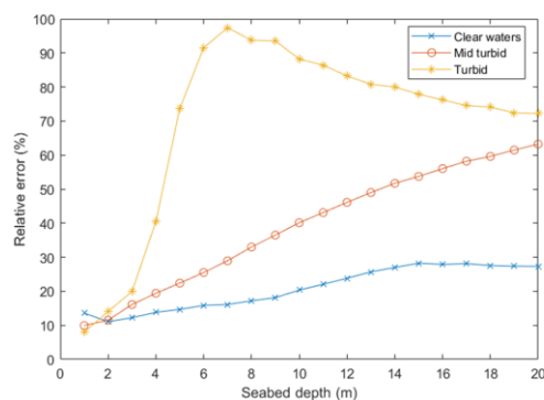
Fig. 10. Variation of the relative errors of the estimated seabed depth with bathymetry and water turbidity when a BIODIVERSITY-like sensor configuration is used.
