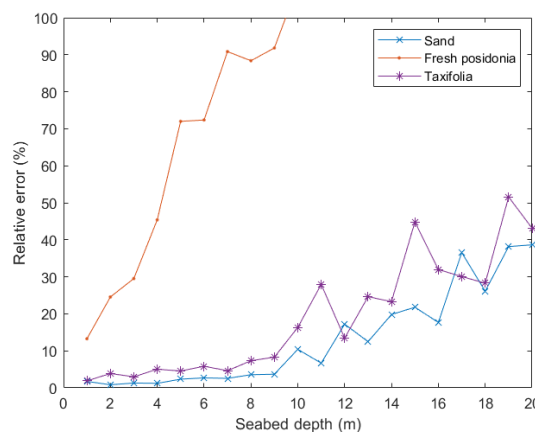
Fig. 13. Variation of the relative errors of the estimated seabed material abundance (in %) with bathymetry for seabed composed of mixed materials, namely 1/3 of Sand, 1/3 of fresh Posidonia , 1/3 of Caulerpa taxifolia species for BIODIVERSITY-like sensor configuration.
