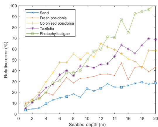
Fig. 12. Variation of the relative errors of the estimated seabed material abundance (in %) with bathymetry for seabed composed of pure materials in clear water, when a BIODIVERSITY-like sensor configuration is used.
