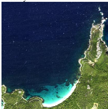
Fig. 2. Hyperspectral image acquired by the HYSPEX sensor above the study area on Sept, 13, 2017.
