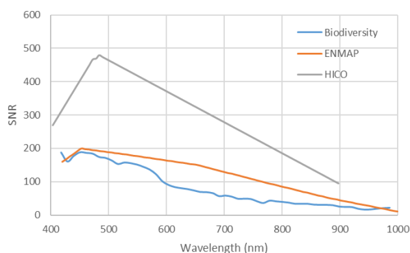
Fig. 8. Signal-to-Noise Ratio (SNR) values used for the 3 sensors
