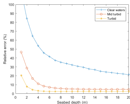
Fig. 9. Variation of the relative errors of the estimated SPM concentration with the seabed depth and water turbidity when a BIODIVERSITY-like sensor configuration is used.
