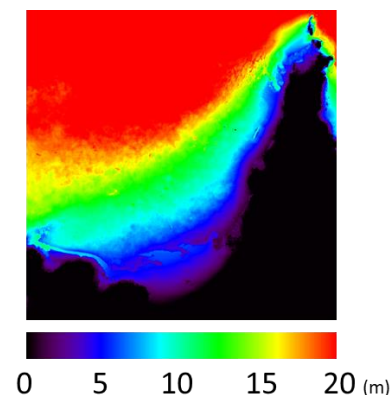
Fig. 3. Litto3D modelled bathymetry for the study area.
