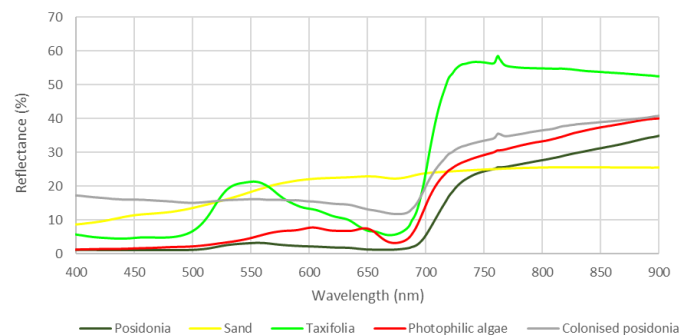
Fig. 4. In-situ measurements of the hyperspectral reflectance of the various components of the seabed, namely the seagrass, sand and algae.
