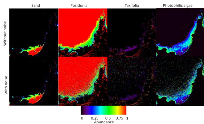
Fig. 16. Retrieved abundance of seabed materials, namely Sand, Posidonia , Caulerpa taxifolia and photophilic algae, from the inversion of satellite data simulated for the BIODIVERSITY-like sensor configuration.
