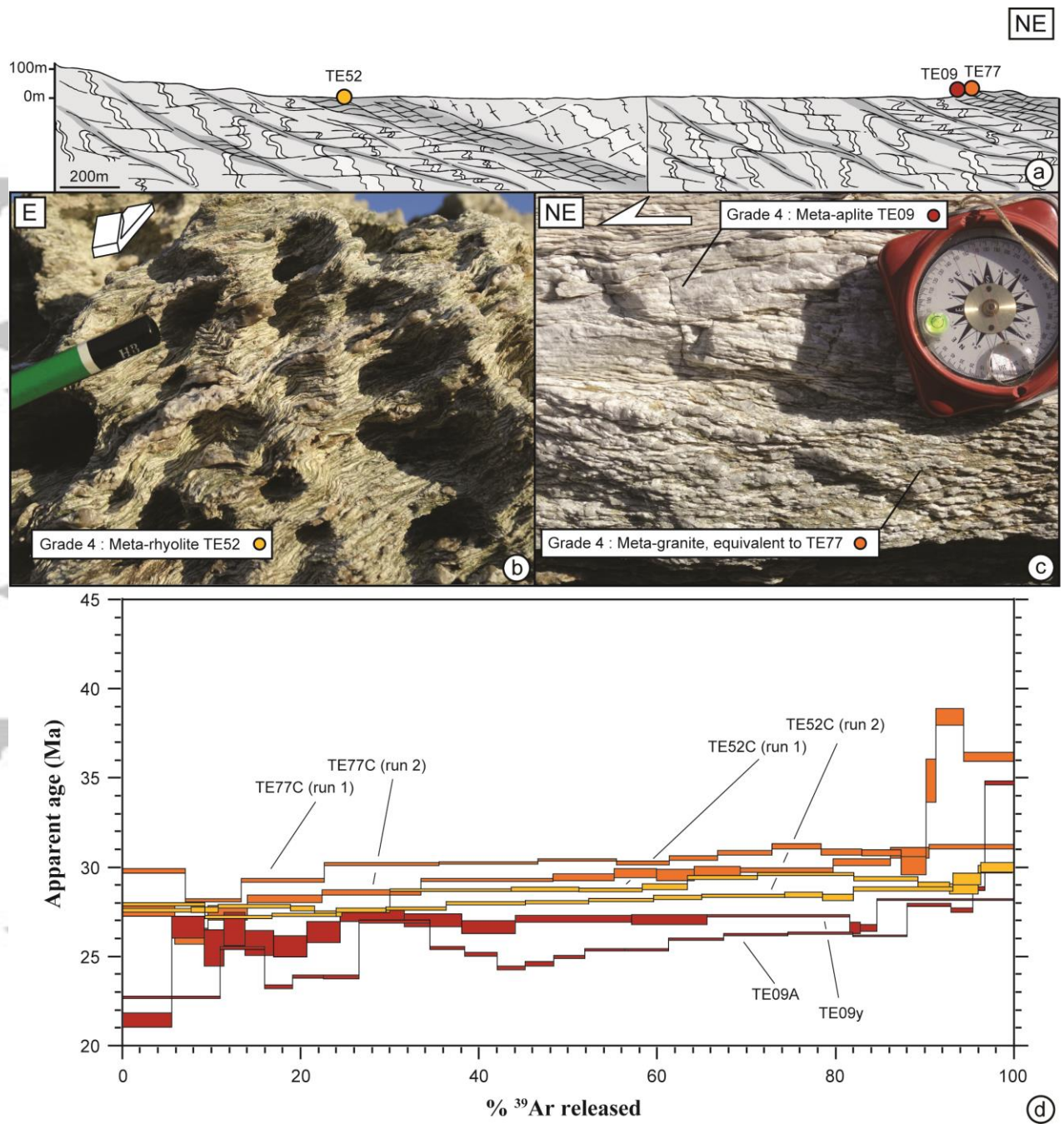
Figure 11: Step-heating analyses from cross section 3 (see Fig. 2). (a) Cross section showing deformation features and samples location. (b) Outcrop picture of sample TE52 (Grade 4), deformed rhyolite from the Saleccia shear zone. (c) Outcrop picture of sample TE09 (ultramylonitic aplite) and an equivalent of sample TE77 (meta-granite mylonite; Grade 4), sampled few meters away, showing S_2/C_2 structures. (d) Step-heating spectra.
