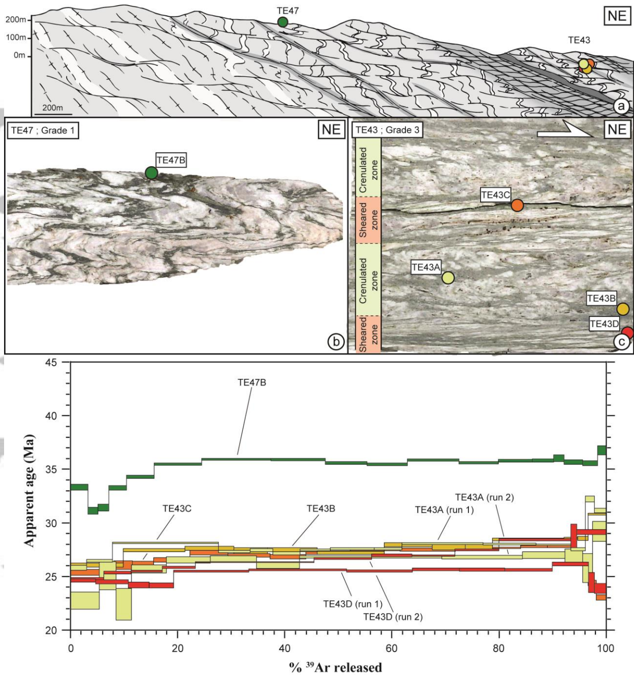
Figure 10: Step-heating analyses from cross section 2 (see Fig. 2). (a) Cross section showing deformation features and samples location. (b) Hand-sample picture of sample TE47 (Grade 1) showing a strong crenulation structure. (c) Hand-sample picture of sample TE43 (Grade 3) showing crenulated structures preserved between highly sheared zones where C_2 shear bands and S_2 tend to parallelize. In situ location of analyzed aggregates are indicated. (d) Step-heating spectra.
