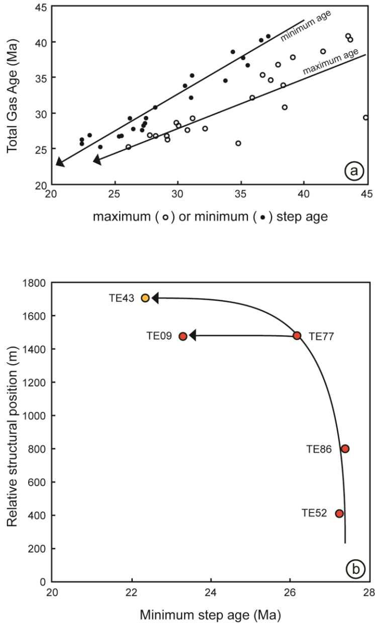
Figure 17: Global age trends. (a) Maximum/minimum recorded age vs. total gas age. (b) minimum recorded ages vs. structural position. Note that for minimum ages, the first step is not considered.
