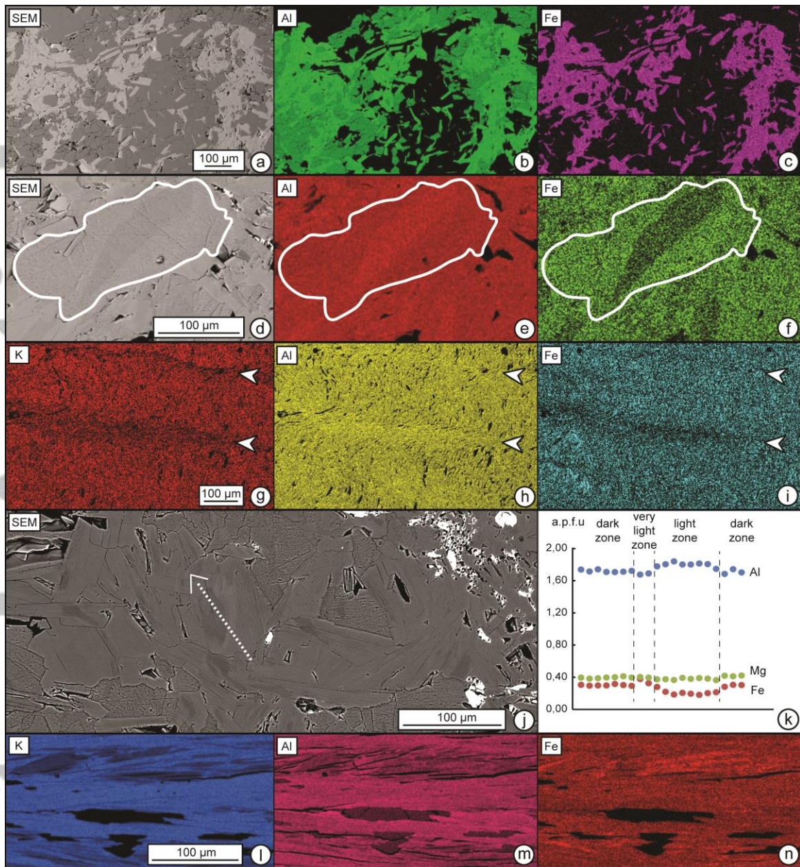
Figure 7: SEM and XRD compositional maps in phengite aggregates. (a), (b) and (c) illustrate homogeneous Al and Fe concentration in some samples (XY sections). (d), (e) and (f) Core (Al-rich)-rim (Fe-rich) zoning in a grain from Grade 0W. (g), (h) and (i) Relative enrichment in Al and depletion in K and Fe in S 2 -phengite (arrows) compared to S 1 -phengite in Grade 1. (j) and (k) Al, Mg and Fe zoning that is not associated with core-rim textures anymore (XY section). (l) Heterogeneous distribution of K interfering with other zonations involving Al (m) and Fe (n) in samples with pyrophyllite-rich phengite.
