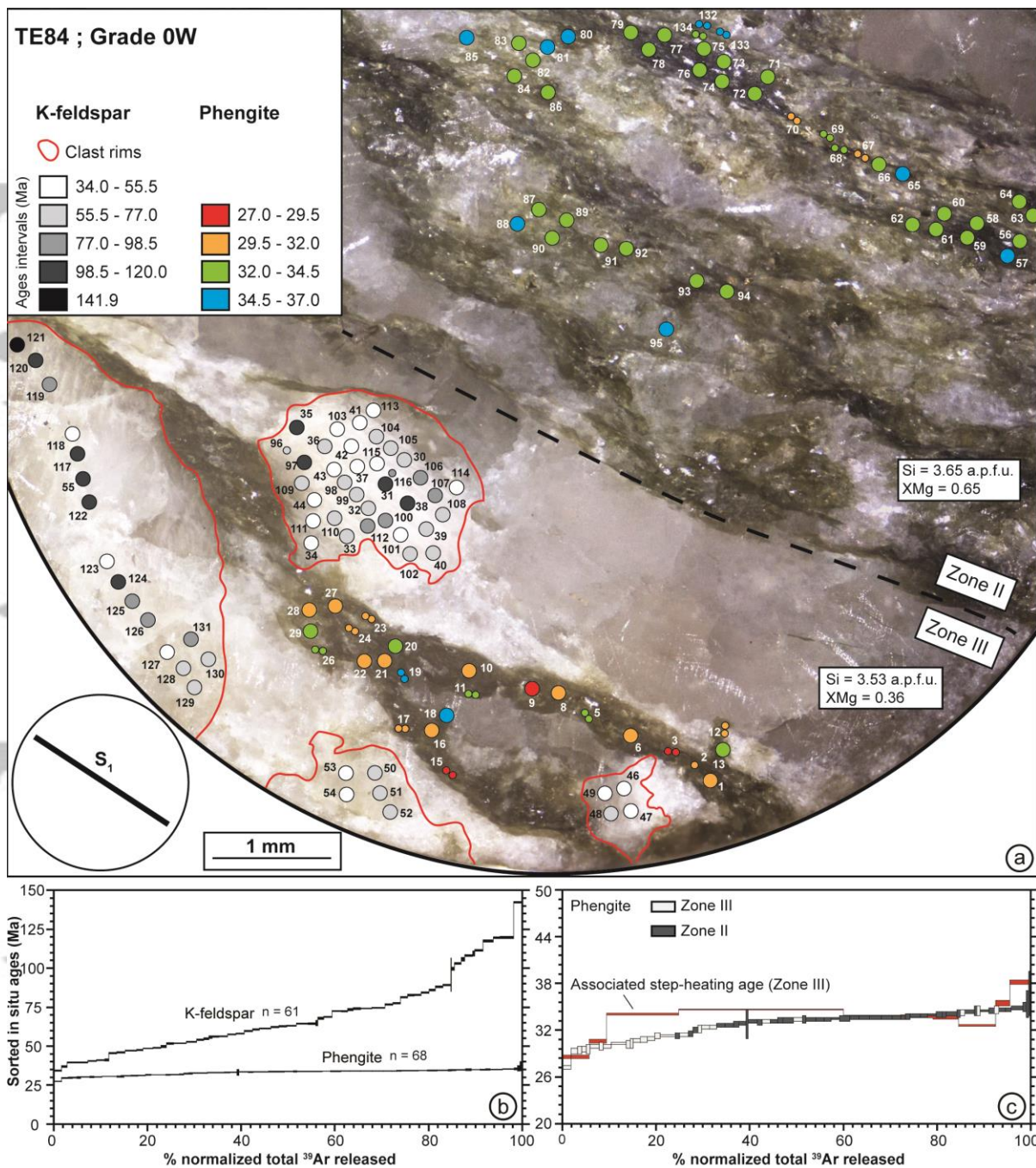
Figure 12: in situ ^{40}\text{Ar}/^{39}\text{Ar} dating of phengite and K-feldspar on section TE84, Grade 0W. (a) Distribution of in situ ages, color scaled for phengite and grey scaled for K-feldspar (grains are contoured in red). In situ ages in phengite are older (~32-37 Ma) in zone II, characterized by the highest mean X_{\text{Mg}} than in zone III (~27-32 Ma), characterized by the lowest mean X_{\text{Mg}} . Besides, they are randomly distributed in each zone. In situ ages in K-feldspar are randomly distributed but older (~35-150 Ma) than ages in phengite. (b) Spectra of sorted in situ ages for K-feldspar and phengite. (c) Close-up of the phengite spectrum. In red, the step-heating spectrum of TE84Y (zone III) for comparison.
