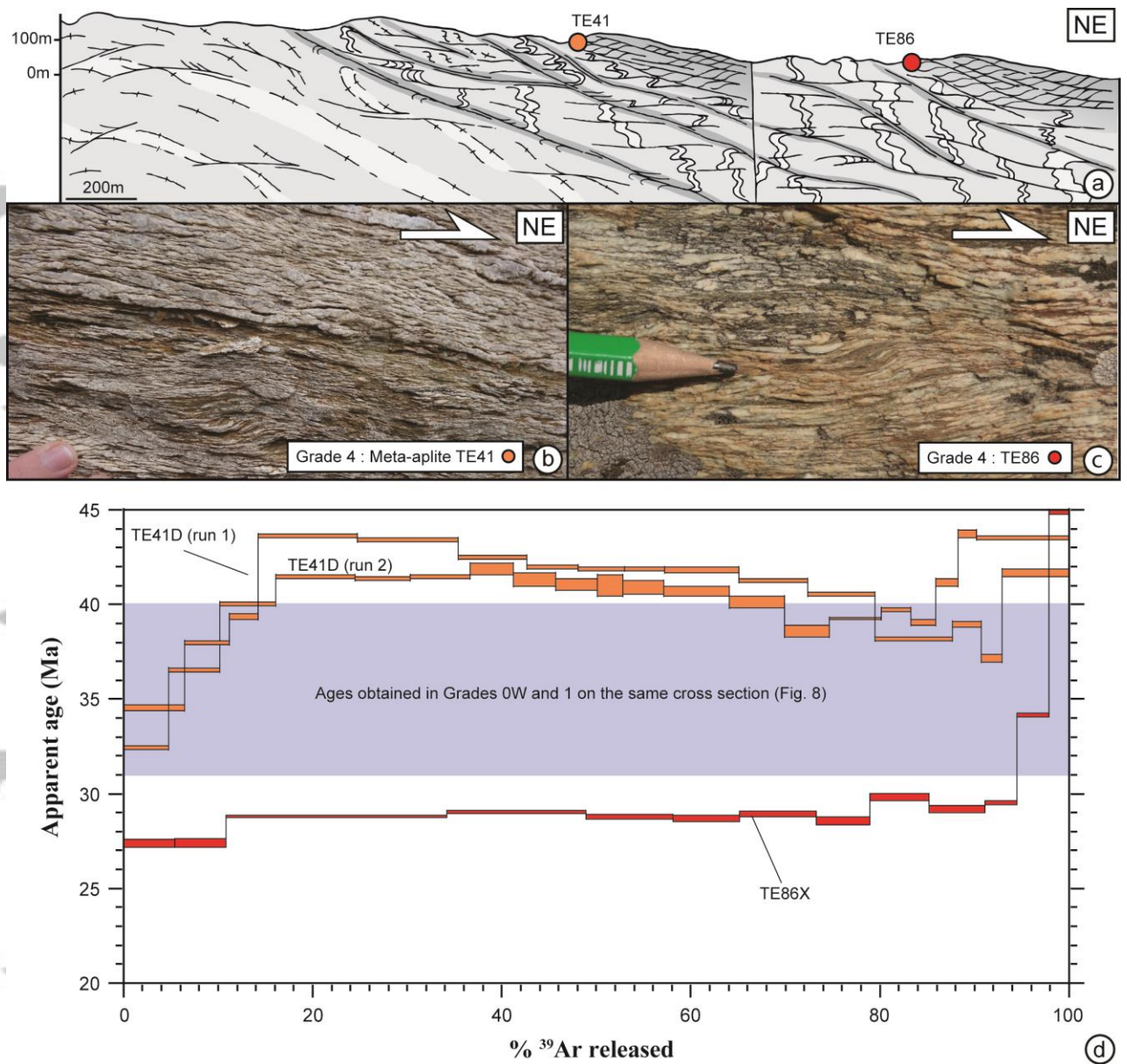
Figure 9: Step-heating analyses from Grade 4 from cross section 1 (see Fig. 2). (a) Cross section showing deformation features and samples location. (b) and (c) Outcrop pictures of meta-aplite TE41 and meta-granite TE86 showing parallelization of S_2 and C_2 shear bands. Few top-to-the-NE indicators remain. (d) Step-heating spectra.
