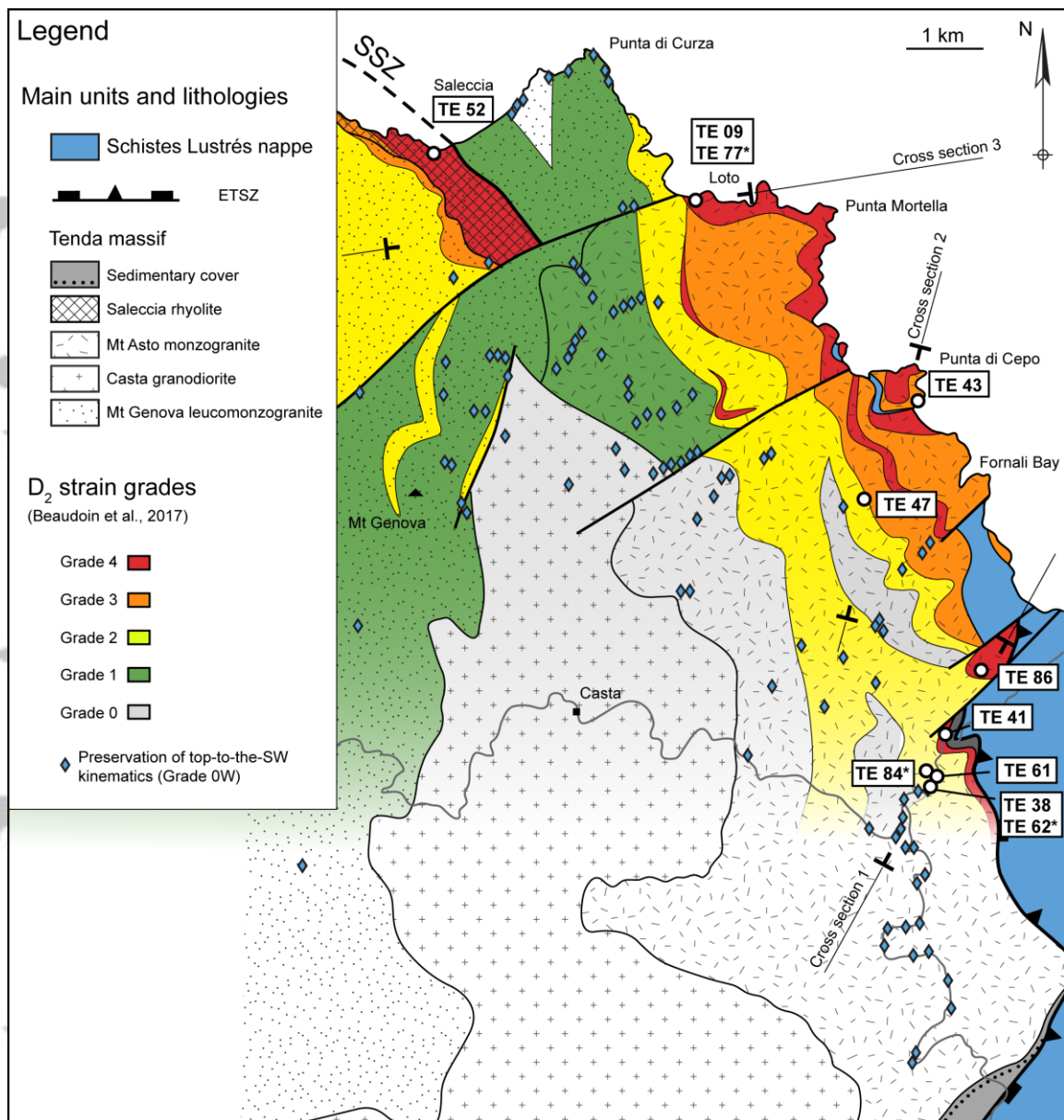
Figure 2: Deformation intensity map and samples location (modified after Beaudoin et al., 2017). The geological outlines in the background are from Rossi et al. (1994a; 2001) and Beaudoin et al. (2017). Cross sections presented in figures 8, 9, 10 and 11 (step-heating results) are indicated. The asterisks indicate samples also dated by the in situ approach.
