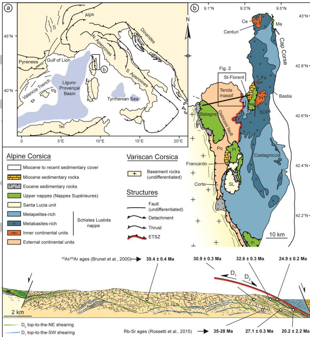
Figure 1: Geological context of the studied area. (a) Tectonic map of the western Mediterranean region. (b) Geological map of Alpine Corsica (modified after Vitale Brovarone et al., 2013) associated with a representative cross-section of the Tenda massif (modified after Beaudoin et al., 2017). Previous ^{40}\text{Ar}/^{39}\text{Ar} and Rb-Sr ages are projected on the cross section. Ce: Centuri continental unit; Fa: Farinole continental unit; In: Inzecca unit; Ma: Macinaggio unit; Ne: Nebbio unit; Sa: Sampolo unit; SDP: Serra di Pigno continental unit; SL: Santa Lucia; Pi: Pineto ophiolitic unit; Po: Popolasca unit.
