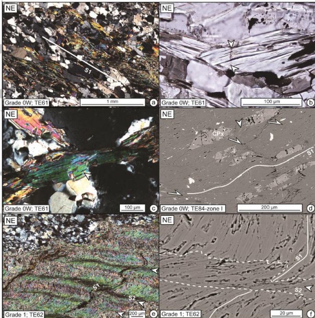
Figure 5: Microstructural observations of white mica aggregates. Strain grade is indicated for each picture. (a) Lattice preferred orientation with (001) parallel to S_1 in Grade 0W. (b) Bending and kinking of (001) associated (top arrow) or not (bottom arrow) with cracking normal to (001). (c) Grain segmentation. (d) C_1/S_1 structures in clinopyroxene/white mica aggregate in TE84-zone I. (e) Folded S_1 between S_2 cleavage (arrows) in Grade 1. (f) Recrystallized grains in S_2 . Note that folding in S_1 is achieved through different strain free grains that are progressively misoriented from each other.
