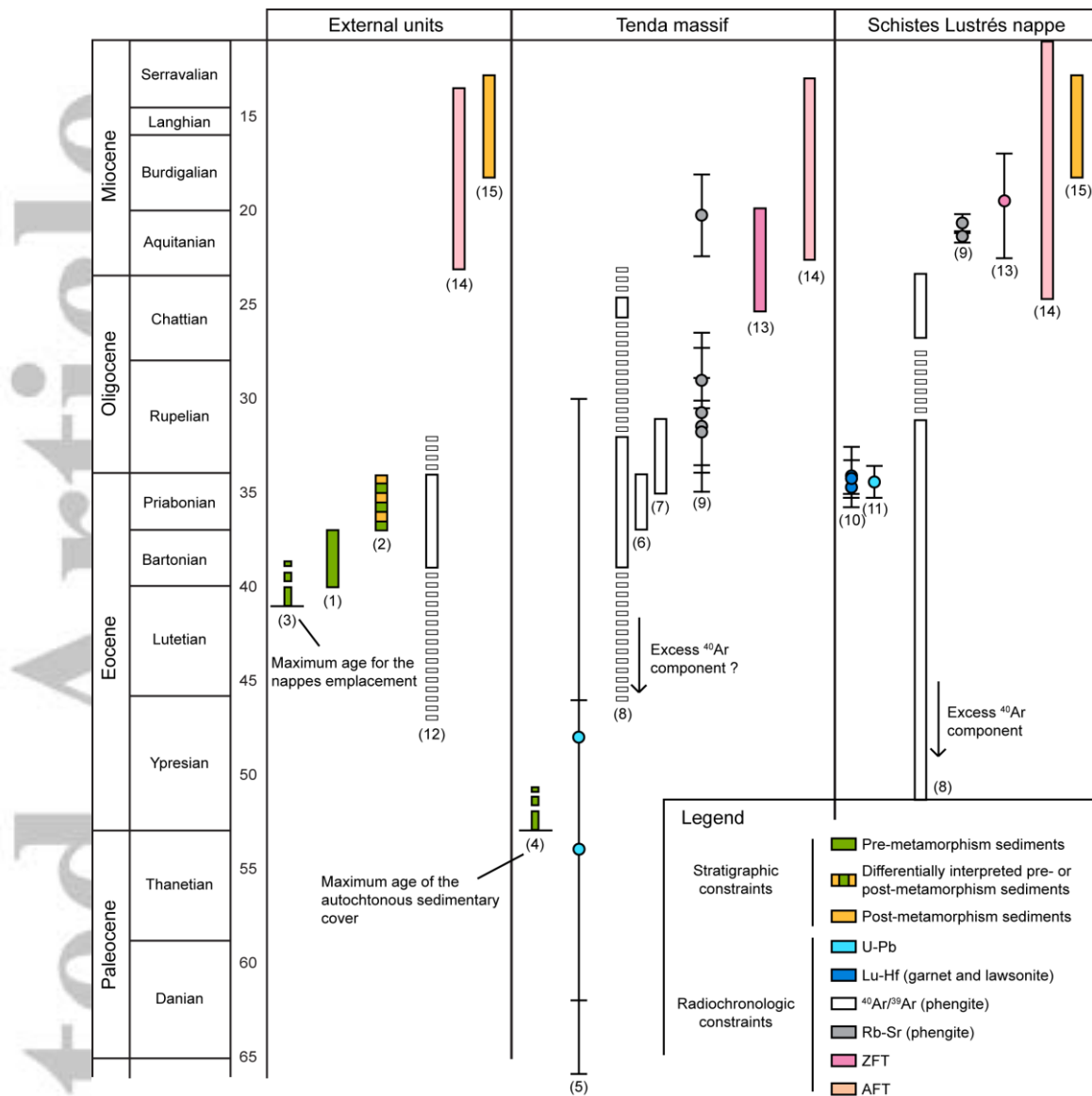
Figure 3: Biostratigraphic and radiometric constraints on tectonic and metamorphic events in Alpine Corsica. See text for further explanations. 1) Bézert and Caby, 1988; 2) Bézert and Caby, 1989; Ferrandini et al., 2010; 3) Nardi et al., 1978; Rossi et al., 1994b; Ferrandini et al., 2010; 4) Rossi et al., 2001; 5) Maggi et al., 2012; 6) Mailhé, 1982; 7) Jourdan, 1988; 8) Brunet et al., 2000; 9) Rossetti et al., 2015; 10) Vitale Brovarone and Herwartz, 2013 ; 11) Martin et al., 2011; 12) Di Vincenzo et al., 2016; 13) Fellin et al., 2006; 14) Cavazza et al., 2001; Zarkni-Jakni et al., 2004; Danisik et al., 2007 ; 15) Ferrandini et al., 2003; Cavazza et al., 2007.
