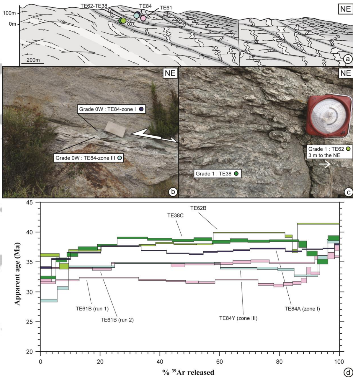
Figure 8: Step-heating analyses from Grades 0W and 1 from cross section 1 (see Fig. 2). (a) Cross section showing deformation features and samples location. (b) Outcrop picture of sample TE84 (Grade 0W). Top-to-the-NE indicators show a weak reworking of this thick shear band localized in a meta-basite, but the thin section shows pervasive top-to-the-SW shear bands (see Fig. 5d). (c) Outcrop picture of sample TE38 (Grade 1) showing crenulated structures. (d) Step-heating spectra.
