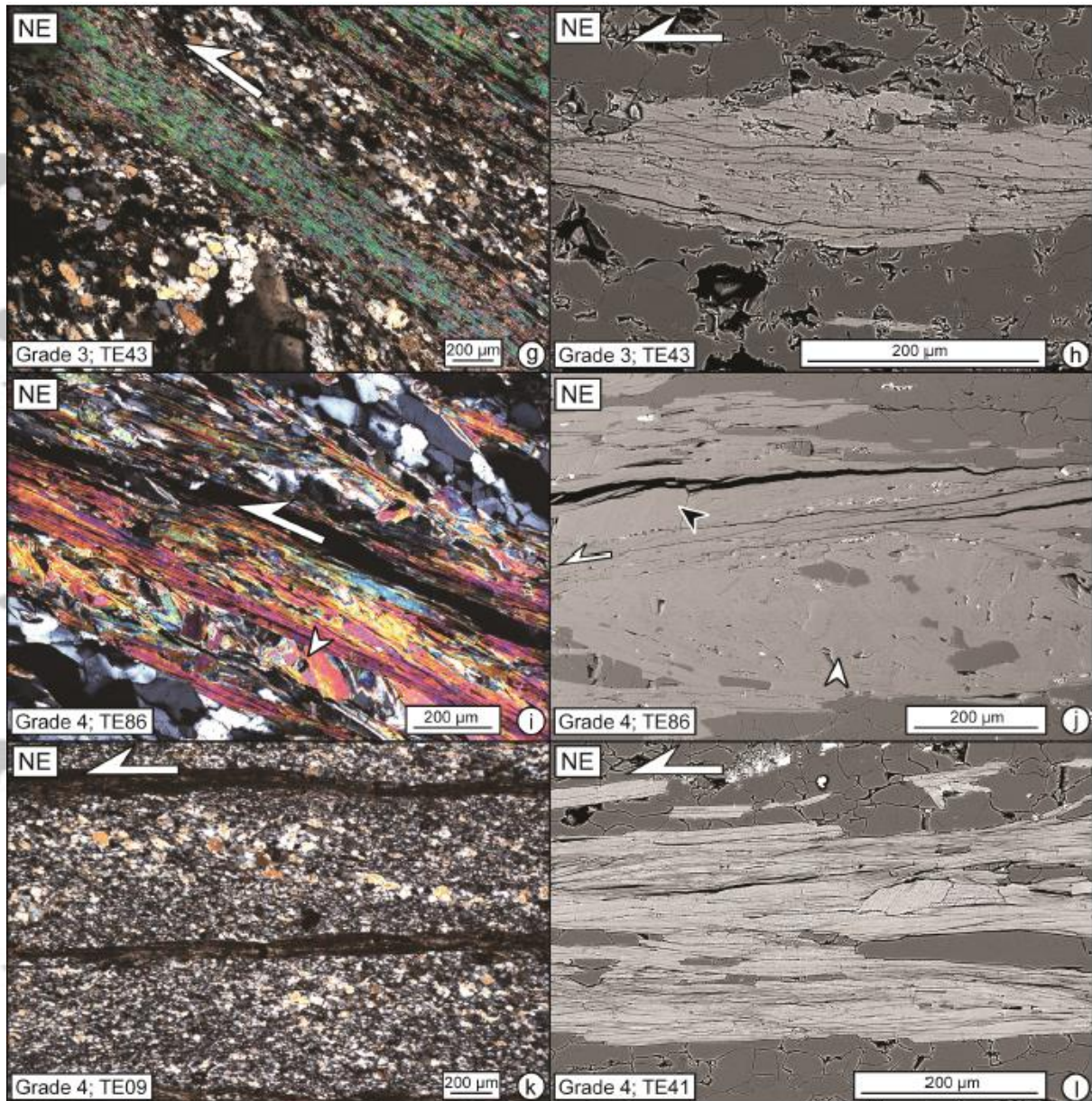
Figure 5: Microstructural observations of white mica aggregates (continued). (g and h) Transposition of grains in C_2 shear zones in Grade 3. (i and j) Coarse grains aligned in C_2 shear bands between microlithons domains with oblique grains (white arrow) in Grade 4. (k and l) Almost total transposition of grains in discrete layers in meta-aplites of Grade 4.
