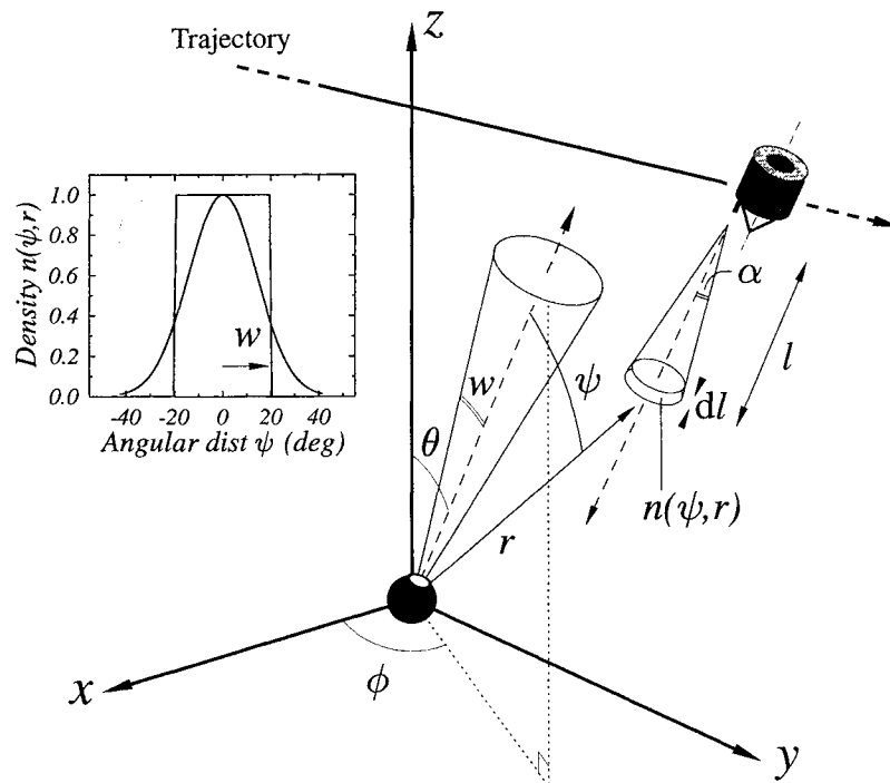
Figure 8. Schematic of the jet model. Particles in jets are assumed to be emitted radially. A jet is defined by parameters f , the fraction of total dust emission from the comet emitted in the jet, and \omega , the angular half-width of the jet (see text). The dust spatial density n(\psi, r) at cometocentric distance r at an angular distance \psi from a jet goes to contribute to the observed brightness seen in the OPE conic field of view.
