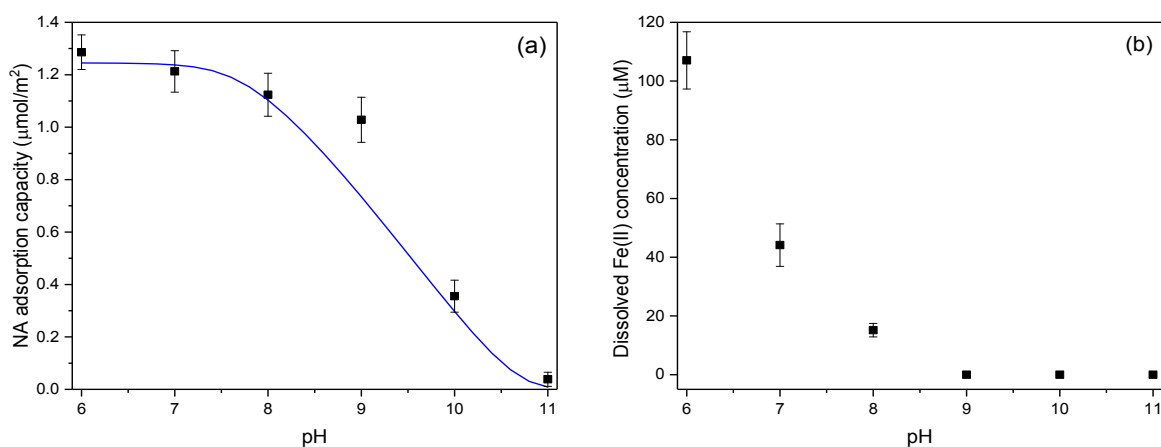
Figure 5. pH-dependency of (a) NA adsorption and (b) dissolved Fe(II) concentration in NZVI suspension after oxidation (5mM H 2 O 2 ). Lines are modeling results. Experimental conditions: [NZVI]=0.2 g·L -1 , [NA]=10 μM, 20 ± 1 °C. The BET surface area used here is that measured for the oxidized particles (using 5 mM of H 2 O 2 ) (28.2 ± 1.5 m 2 /g).
