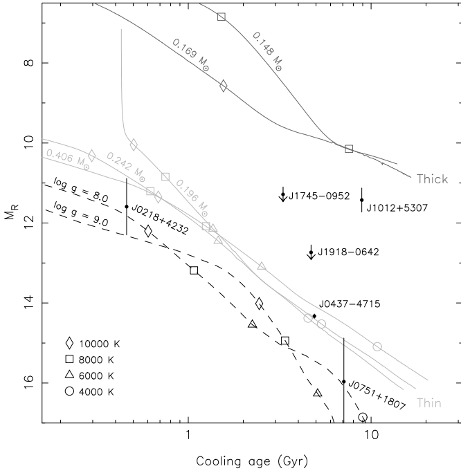
Fig. 5. Absolute R -band magnitude and cooling age predictions. Shown are helium-core white dwarf cooling tracks by Rohrmann et al. (2002) and carbon-oxygen white dwarf cooling tracks with hydrogen-rich atmospheres by Bergeron et al. (1995) ( \log g = 8 corresponds to M_c \approx 0.6 M_\odot while \log g = 9 corresponds to M_c \approx 1.2 M_\odot ). Helium-core models with masses below approximately 0.18\text{--}0.20 M_\odot have thick hydrogen envelopes and continue to residually burn hydrogen, keeping the white dwarf hot and slowing the cooling. Heavier models have thin hydrogen envelopes and cool much faster, creating a dichotomy in the cooling properties of white dwarf companions to millisecond pulsars. White dwarfs with carbon-oxygen cores cool even faster. Shown with error bars are PSR J0218+4232 (Bassa et al. 2003), PSR J0437-4715 (Danziger et al. 1993), PSR J0751+1807 (Bassa et al. 2006) and PSR J1012+5307 (Lorimer et al. 1995), where the white dwarf cooling age is assumed to be equal to the characteristic age of the pulsar (using braking indices of n = 3 ). Shown with upper limits on the absolute R -band magnitude are the values for PSR J1745-0952 and PSR J1918-0642. For these two pulsars, thick hydrogen envelopes are excluded, indicating the white dwarf companions in these systems are heavier than about 0.2 M_\odot .
