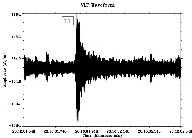
Fig. 5. VLF wave form from the electric field experiment onboard the DEMETER satellite gathered at the time of L1 (see Table 1).
