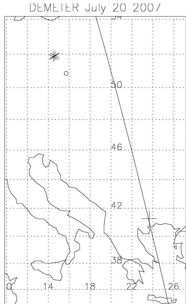
Fig. 2. Map showing the orbit of DEMETER (black line). The sign + indicates the position of DEMETER at the time of the optical observation performed at Śnieżka observatory (the sign o). The two stars give the position of the parent lightning strokes. The distance between the location of the event and the satellite position was around 1200 km.
