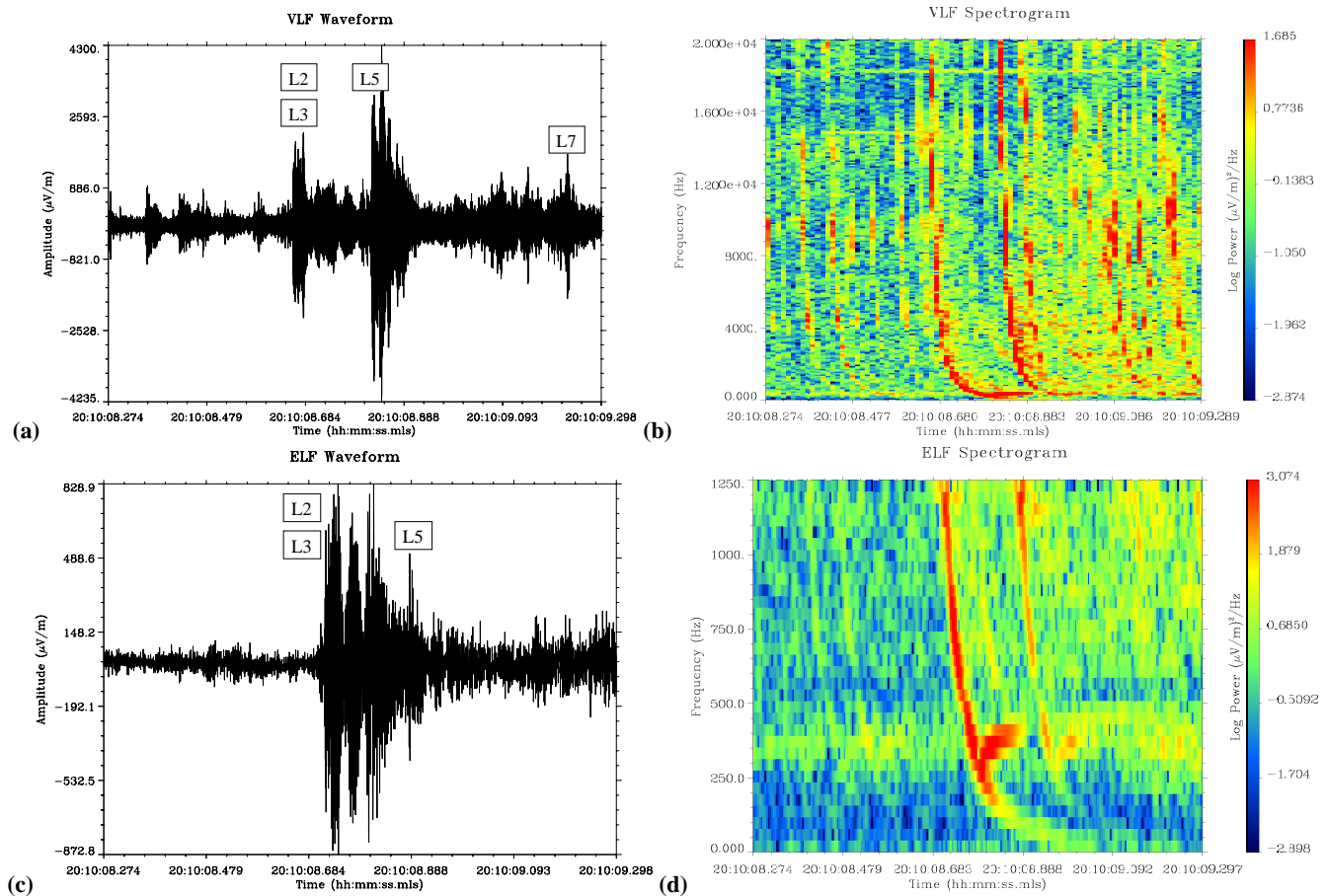
Fig. 3. ELF/VLF data from the electric field experiment onboard the DEMETER satellite gathered during the time of the sprite registration: (a) wave form of the VLF signal, horizontal axis – time (UT), vertical axis – value of the electric field in \mu\text{V/m} , (b) spectrogram of the signal shown in (a), horizontal axis – time, vertical axis – frequency, the intensity is color-coded according to the scale on the right, (c) wave form of the ELF signal, (d) Spectrogram of the ELF signal shown in (c). The discussion is given in the text.
