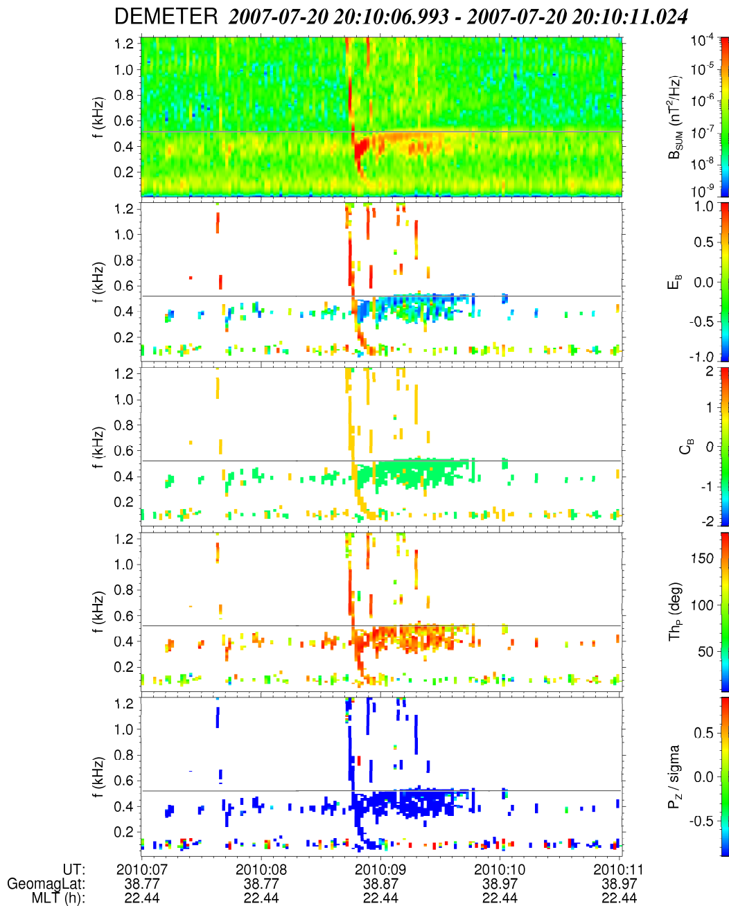
Fig. 4. Analysis of the propagation of the ELF signal during the event as function of the time. From the top to the bottom, the first panel shows the spectrum of the magnetic field variations (sum of the 3 components), the second panel displays the ellipticity of magnetic field polarization – value of 1 means right-hand circularly polarized waves, linear polarization gives 0, and –1 means left-hand circular polarization, the third panel is the sense of polarisation of the waves, the fourth panel indicates the angle between the wave vector and the Earth’s magnetic field calculated by the SVD technique (Santolik et al., 2003), and the bottom panel represents the Poynting vector. Empty areas in the four bottom panels correspond to magnetic power-spectral densities below 10^{-6} \text{ nT}^2 \text{ Hz}^{-1} . The geomagnetic latitude and the Magnetic Local Time (MLT) are displayed at the bottom of the figure. The discussion of the results is given in the text.
