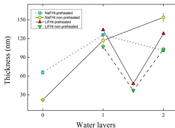
Figure 6. Clay particle thickness with error bars, obtained from the Scherrer equation and the Lorentzian width, as a function of the number of water layers for the Na- and LiFht non-preheated and preheated samples.
