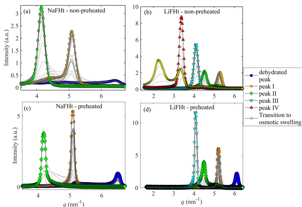
Figure 2. Diffraction peaks corresponding to the stable hydration states for (a, c) NaFht and (b, d) LiFht for samples subjected to different thermal treatments prior to the in situ hydration. Gray curves show intermediate states during the hydration transitions. The measurements marked with colored symbols are the stable peaks.
