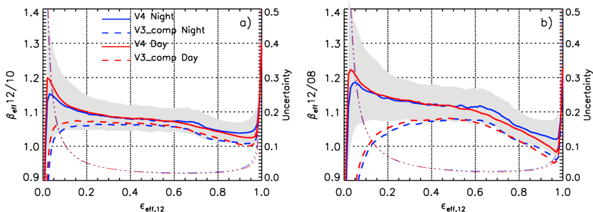
305 Figure 5: (a) \beta_{\text{eff}12/10} and (b) \beta_{\text{eff}12/08} microphysical indices vs. effective emissivity at 12.05 \mu\text{m} in single-layered ice clouds over oceans between 60°S and 60°N in January 2008 in V4 (solid lines) and in V3_comp (dashed lines). The blue and red curves are the median values for nighttime (blue) and daytime (red) and the shaded gray areas are between the nighttime 25 th and 75 th percentiles. The blue (night) and red (day) thin dotted dashed lines are the V4 random absolute uncertainty estimates with vertical axis on the right-hand side of each panel.
