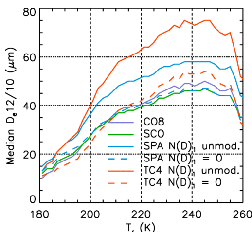
Figure 10: Median D_{e12/10} from the V4 CO8 (purple) and SCO (green) models, and from analytical functions derived by Mitchell et al. (2018) during the SPARTICUS (blue) and TC4 (red) field experiments using N(D)_1 unmodified (solid) or N(D)_1 = 0 (dashed). Same dataset as in Fig. 9.
