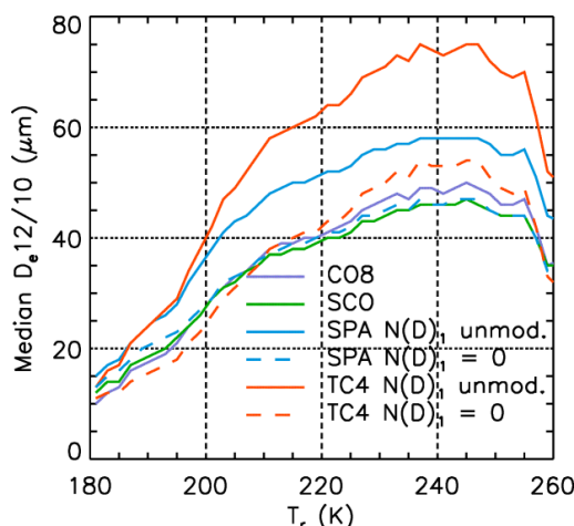
455 Figure 10: Median D_{e12/10} from the V4 CO8 (purple) and SCO (green) models, and from analytical functions derived by Mitchell et al. (2018) during the SPARTICUS (blue) and TC4 (red) field experiments using N(D)_1 unmodified (solid) or N(D)_1 = 0 (dashed). Same dataset as in Fig. 9.
