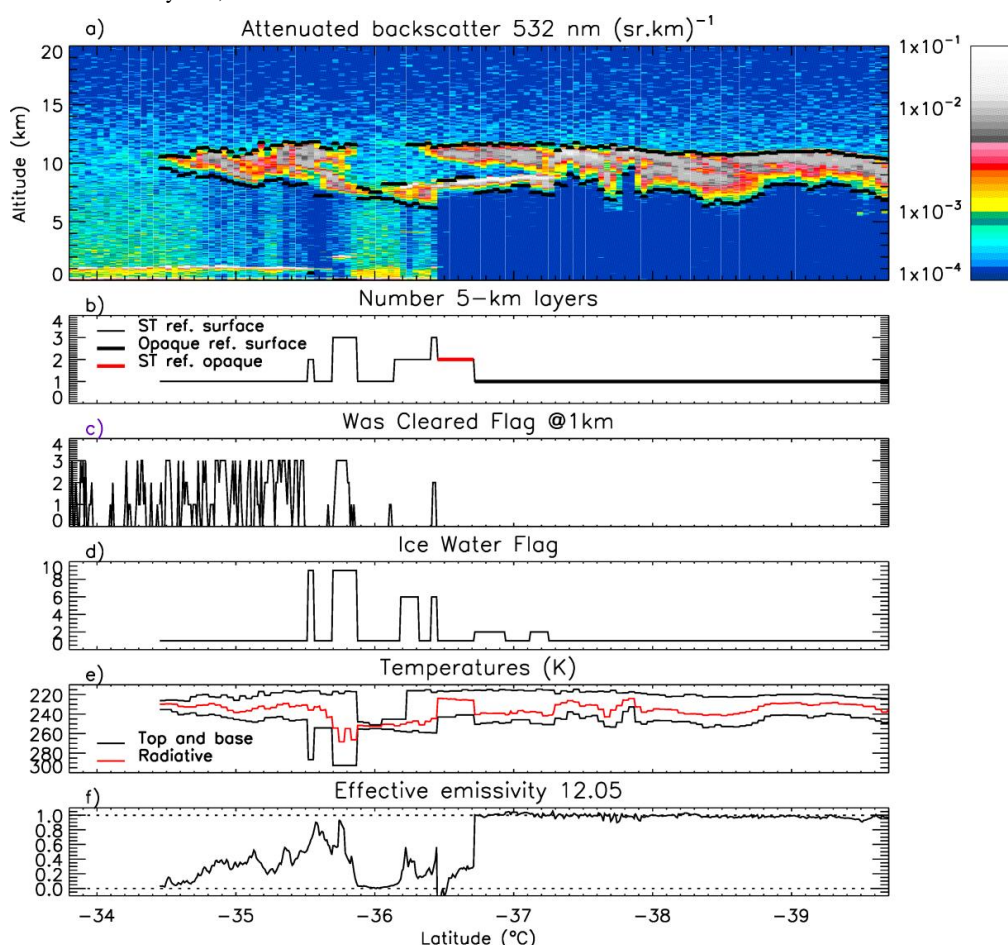
130 Figure 1: Example of the CALIOP scene classification information used for effective emissivity retrievals on January 30 th , 2008 (granule 2008-01-30T09-15-45Z). (a) CALIOP attenuated backscatter with top and base altitudes of the cloud-system highlighted in black; (b): number of cloud layers in the cloud-system; cases with Earth surface as a reference are denoted with black lines (thin: semi-transparent (ST) layers; thick: 1 opaque layer) and in red are the cases with the lowest opaque cloud as a reference; (c): CALIOP “Was Cleared Flag” at 1-km IIR pixel resolution; (d): Ice Water Flag of the cloud system (e): temperatures at cloud top and cloud base (black) and radiative temperature used by the IIR algorithm (red); (f): effective emissivity of the cloud-system at 12.05 \mu\text{m} . See text for details.
