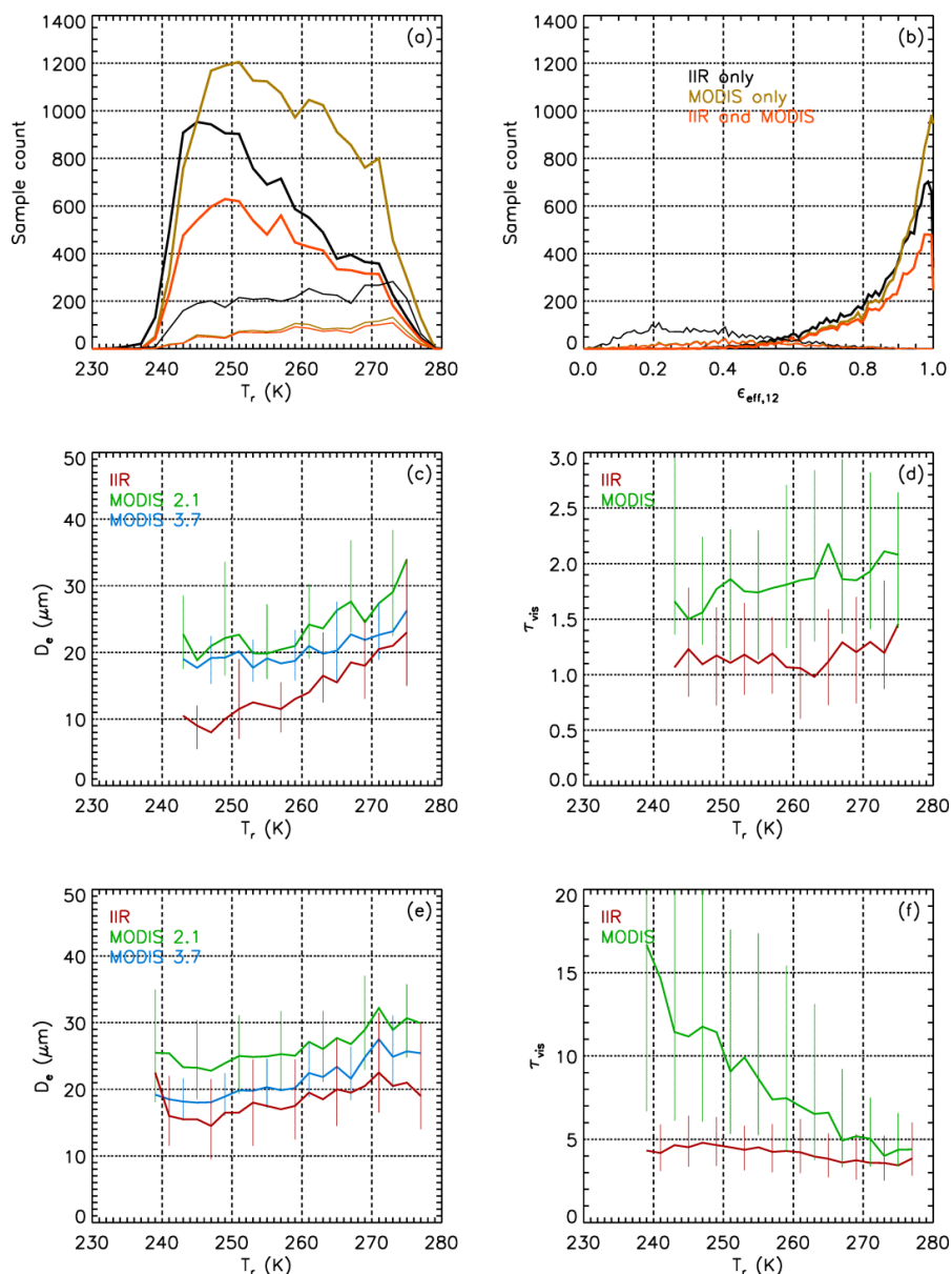
610 Figure 16: IIR and MODIS comparisons over oceans between 60° S and 60° N in January 2008 for single-layered high confidence liquid water clouds of centroid altitude > 4 km with MODIS water phase. Top: distributions of (a) IIR radiative temperature and (b) IIR effective emissivity at 12.05 \mu\text{m} in ST (thin lines) and opaque (thick lines) clouds where IIR has confident retrievals (black), MODIS has successful retrievals at 2.1 and 3.7 \mu\text{m} (brown), and both IIR and MODIS retrievals are successful and can be compared (orange). Median D_e vs. T_r from IIR (red), MODIS 2.1 (green) and MODIS 3.7 (blue) in ST (c) and opaque (e) clouds; Median \tau_{vis} from IIR (red) and MODIS (green) in ST (d) and opaque (f) clouds. The vertical bars in panels (c-f) are between the 25 th and 75 th percentiles.
