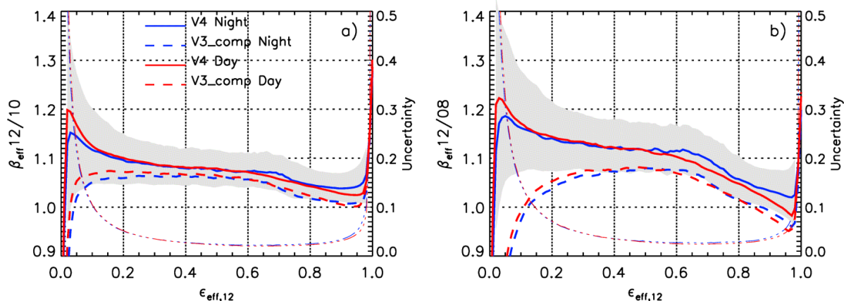
305 Figure 5: (a) \beta_{\text{eff}12/10} and (b) \beta_{\text{eff}12/08} microphysical indices vs. effective emissivity at 12.05 \mu\text{m} in single-layered ice clouds over oceans between 60°S and 60°N in January 2008 in V4 (solid lines) and in V3_comp (dashed lines). The blue and red curves are the median values for nighttime (blue) and daytime (red) and the shaded gray areas are between the nighttime 25 th and 75 th percentiles. The blue (night) and red (day) thin dotted dashed lines are the V4 random absolute uncertainty estimates with vertical axis on the right-hand side of each panel.
