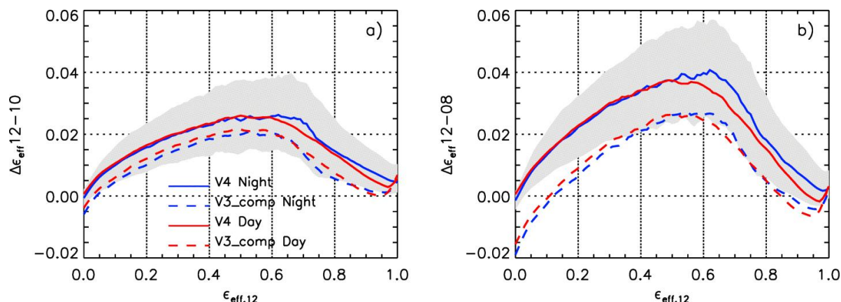
Figure 3: IIR inter-channel (a) \Delta\epsilon_{\text{eff},12-10} and (b) \Delta\epsilon_{\text{eff},12-08} effective emissivity differences vs. effective emissivity at 12.05\ \mu\text{m} in single-layered ice clouds over oceans between 60^\circ\text{S} and 60^\circ\text{N} in January 2008 in V4 (solid lines) and in V3_comp (dashed lines). The blue and red curves are median values for nighttime and daytime data, respectively. The shaded gray areas are between the V4 nighttime 25 th and 75 th percentiles.
