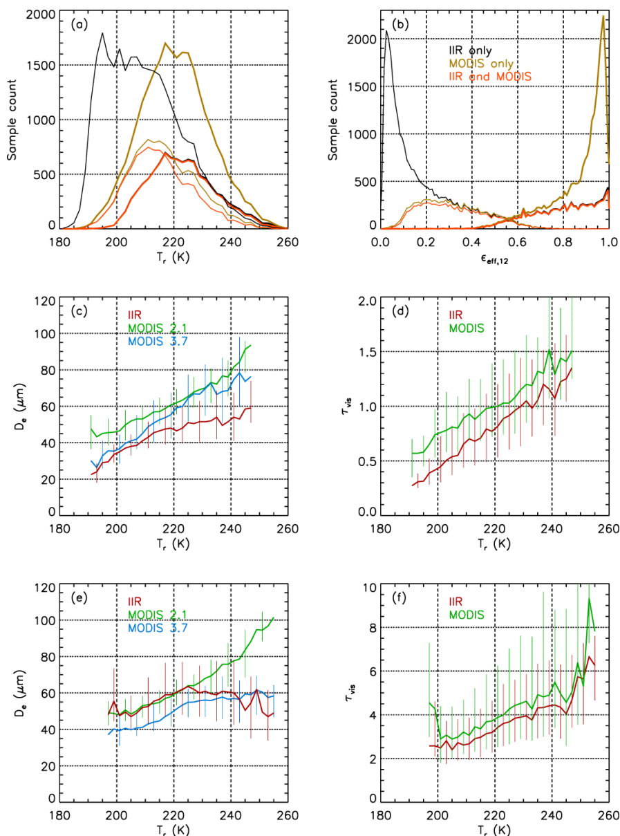
495 Figure 11: IIR and MODIS comparisons over oceans between 30° S and 30° N in January 2008 for single-layered high confidence ROI clouds with MODIS ice phase. Top: distributions of (a) IIR radiative temperature and (b) IIR effective emissivity at 12.05 \mu\text{m} in ST (thin lines) and opaque (thick lines) clouds where IIR has confident retrievals (black), MODIS has successful retrievals at 2.1 and 3.7 \mu\text{m} (brown), and both IIR and MODIS retrievals are successful and can be compared (orange). Median D_e vs. T_r from IIR (red), MODIS 2.1 (green) and MODIS 3.7 (blue) in ST (c) and opaque (e) clouds; Median \tau_{\text{vis}} from IIR (red) and MODIS (green) in ST (d) and opaque (f) clouds. The vertical bars in panels (c-f) are between the 25 th and 75 th percentiles.
