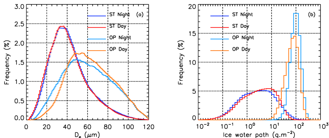
385 Figure 8: Histograms of V4 confident retrievals of (a) D_e and (b) Ice water path in single-layered semi-transparent (ST; Night: navy blue; Day: red) and opaque (OP; Night: light blue; Day: orange) ice clouds between 60^\circ S and 60^\circ N over oceans in January 2008.
