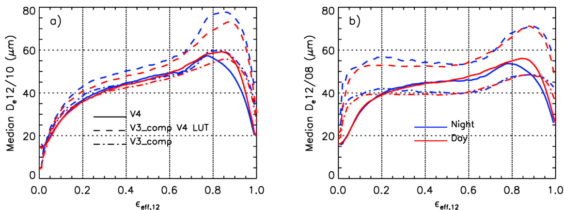
355 Figure 7: (a) Median D_{e12/10} and (b) median D_{e12/08} vs. effective emissivity at 12.05 \mu\text{m} for the cloud population used in Fig. 6, except that both \beta_{\text{eff}12/10} and \beta_{\text{eff}12/08} are in the range of possible retrievals, both in V3_comp and in V4. Solid line: V4 with SCO LUT; dashed lines: V3_comp with V4 SCO LUT; dashed dotted line: V3_comp with V3 solid column LUT. Blue: night; red: day.
