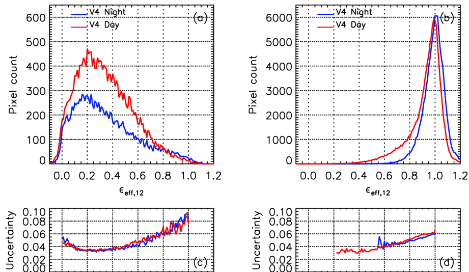
Figure 13. V4 effective emissivity distribution at 12.05\ \mu\text{m} in (a) ST and (b) opaque single-layered liquid water clouds of centroid altitude >4\ \text{km} over oceans between 60^\circ\ \text{S} and 60^\circ\ \text{N} in January 2008 for nighttime (blue) and daytime (red) data. Panels (c) and (d) are the V4 median random uncertainties corresponding to panels (a) and (b), respectively.
