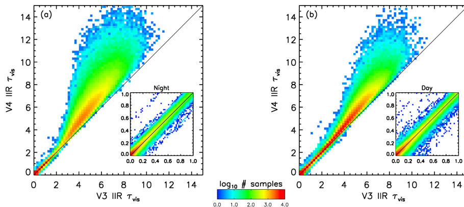
Figure 4. (a) Nighttime and (b) daytime comparisons of V3 and V4 IIR cloud optical depth ( \tau_{\text{vis}} ) in single-layered ice clouds over oceans between 60° S and 60° N in January 2008. The small embedded plots show details for \tau_{\text{vis}} between 0 and 1.
