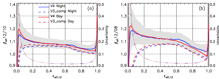
Figure 5. (a) \beta_{\text{eff}12/10} and (b) \beta_{\text{eff}12/08} microphysical indices vs. effective emissivity at 12.05\ \mu\text{m} in single-layered ice clouds over oceans between 60^\circ\ \text{S} and 60^\circ\ \text{N} in January 2008 in V4 (solid lines) and in V3_comp (dashed lines). The blue and red curves are the median values for nighttime (blue) and daytime (red), and the shaded gray areas are between the V4 nighttime 25th and 75th percentiles. The blue (night) and red (day) thin dashed–dotted lines are the V4 random absolute uncertainty estimates with the vertical axis on the right-hand side of each panel.
