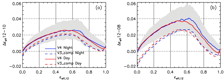
Figure 3. IIR inter-channel (a) \Delta\varepsilon_{\text{eff}12-10} and (b) \Delta\varepsilon_{\text{eff}12-08} effective emissivity differences vs. effective emissivity at 12.05 \mu\text{m} in single-layered ice clouds over oceans between 60° S and 60° N in January 2008 in V4 (solid lines) and in V3_comp (dashed lines). The blue and red curves are median values for nighttime and daytime data, respectively. The shaded gray areas are between the V4 nighttime 25th and 75th percentiles.
