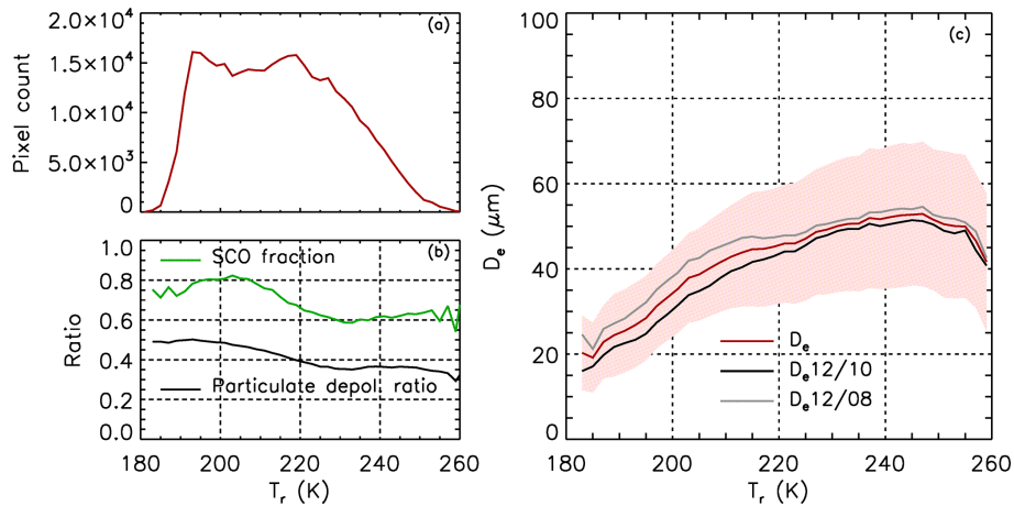
Figure 9. IIR V4 confident retrievals vs. radiative temperature in semi-transparent ice clouds over oceans between 60^{\circ} S and 60^{\circ} N in January 2008. (a) Pixel count; (b) fraction of retrievals using the SCO model (green) and mean CALIOP integrated particulate depolarization ratio (black); (c) mean D_e (red) \pm mean absolute deviation (shaded area), mean D_{e12/10} (black) and mean D_{e12/08} (gray).
