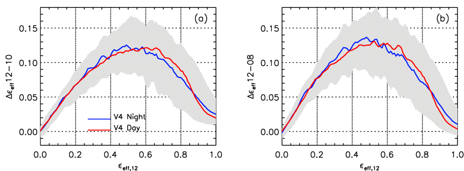
Figure 14. V4 IIR inter-channel (a) \Delta\epsilon_{\text{eff},12-10} and (b) \Delta\epsilon_{\text{eff},12-08} effective emissivity differences vs. effective emissivity at 12.05\ \mu\text{m} in single-layered liquid water clouds of centroid altitude >4\ \text{km} over oceans between 60^\circ\ \text{S} and 60^\circ\ \text{N} in January 2008. The blue and red curves are median values for nighttime and daytime data, respectively. The shaded gray areas are between the V4 nighttime 25th and 75th percentiles.
