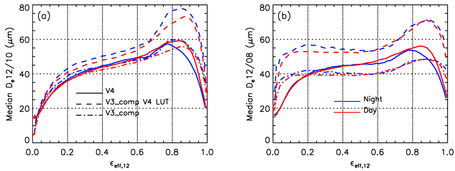
Figure 7. (a) Median D_e 12/10 and (b) median D_e 12/08 vs. effective emissivity at 12.05 \mu\text{m} for the cloud population used in Fig. 6, except that both \beta_{\text{eff}}12/10 and \beta_{\text{eff}}12/08 are in the range of possible retrievals, both in V3_comp and in V4. Solid line: V4 with SCO LUT; dashed lines: V3_comp with V4 SCO LUT; dashed–dotted line: V3_comp with V3 solid column LUT. Blue: night; red: day.
