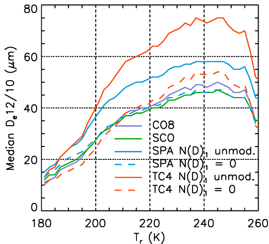
Figure 11. Median D_{e12/10} from the V4 CO8 (purple) and SCO (green) models, and from analytical functions derived by Mitchell et al. (2018) during the SPARTICUS (blue) and TC4 (red) field experiments using N(D)_1 unmodified (solid) or N(D)_1 = 0 (dashed). This is the same dataset as the one in Fig. 9.
