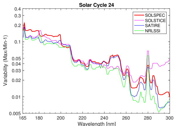
Fig. 5. Solar cycle 24 variability for observations (SOLAR/SOLSPEC and SORCE/SOLSTICE) and models (SATIRE and NRLSSI). The time range of solar cycle 24 is the time from the minimum of cycle 23/24 to the maximum of solar cycle 24 (late 2008 to early 2015).
