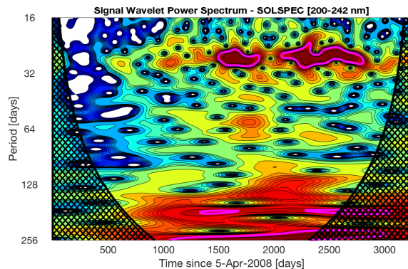
Fig. 7. Signal wavelet power spectrum from Morlet wavelet analysis of SOLAR/SOLSPEC time series (200–242 nm). The plot is jet-colored, where bright red indicates high wavelet power spectrum values. The regions with greater than 95% confidence are shown with thin pink contours. Anything below the cone of influence is dubious.
