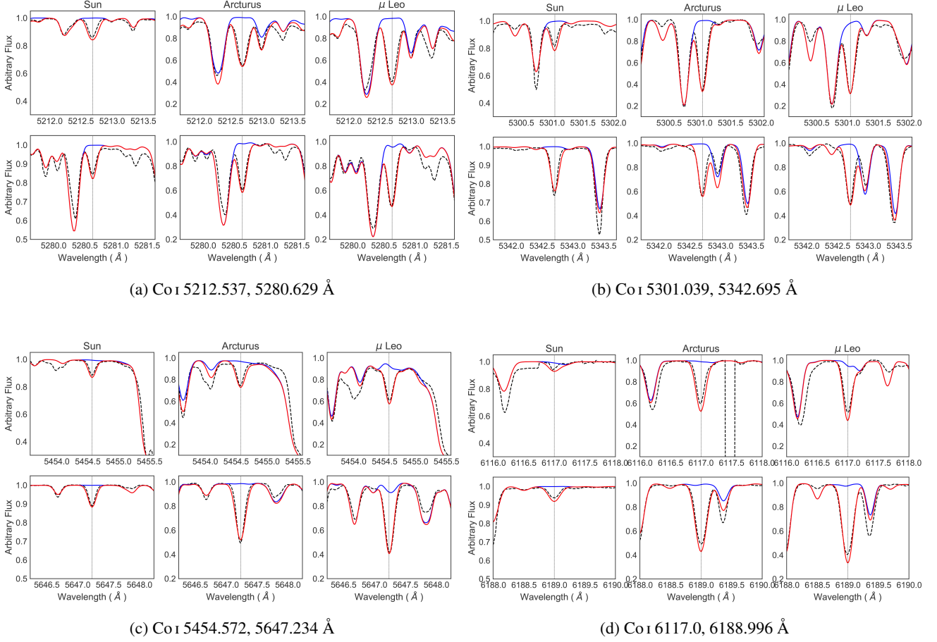
Fig. C.1. Cobalt lines as fitted to the Sun, Arcturus, and \mu Leo.
