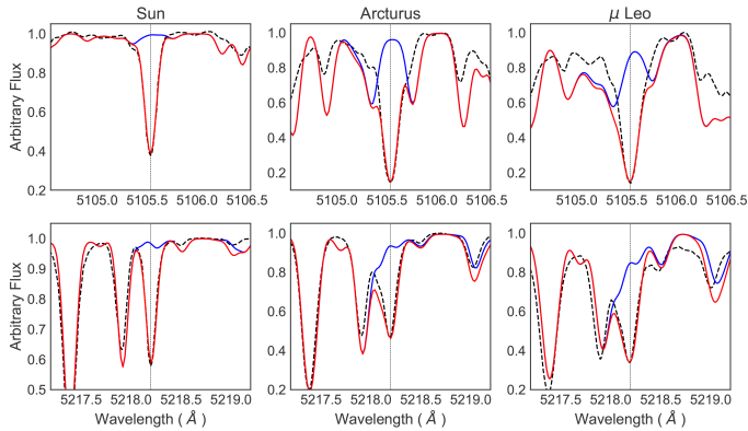
Fig. C.2. Copper lines Cu I 5105.537 and 5218.197 Å, as fitted to the Sun, Arcturus, and \mu Leo.
