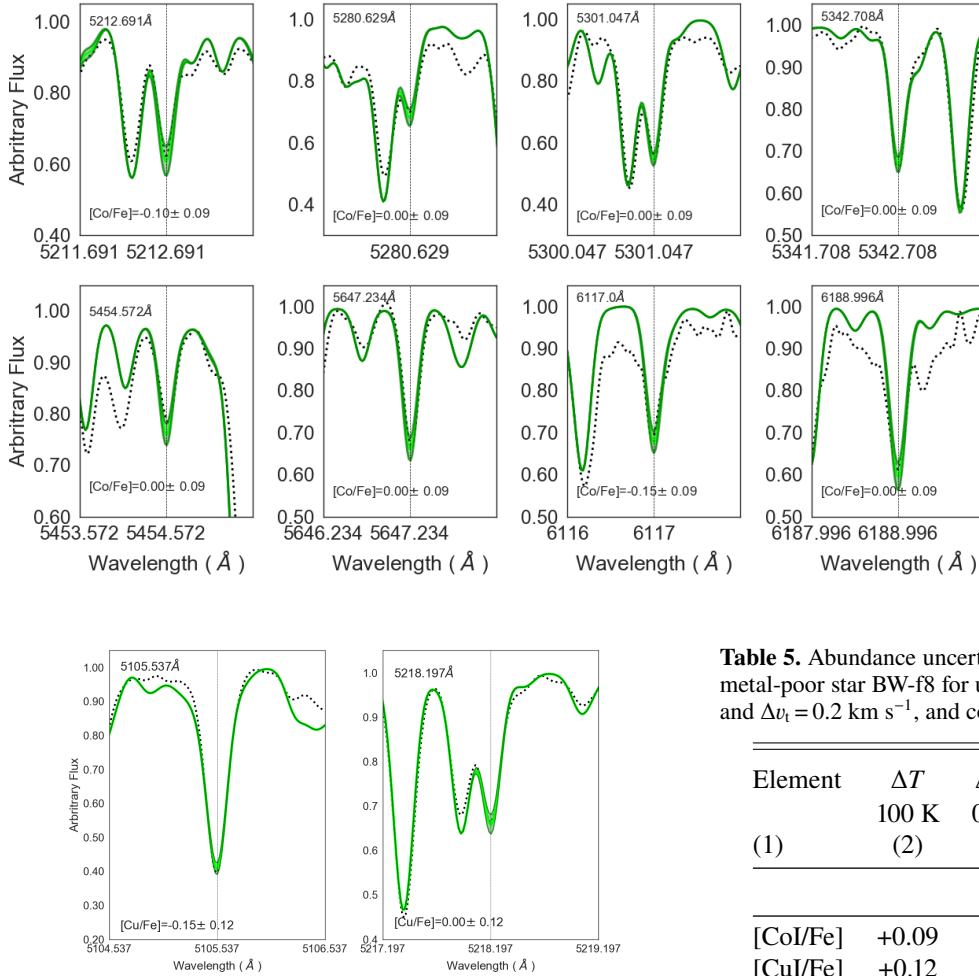
Fig. 2. Fits of synthetic spectra to the two observed lines of Cu I in star BL-7. The dotted line is the observed spectrum. The green lines correspond to the value adopted, and with [\text{Cu/Fe}] = +0.12 and -0.12 .
