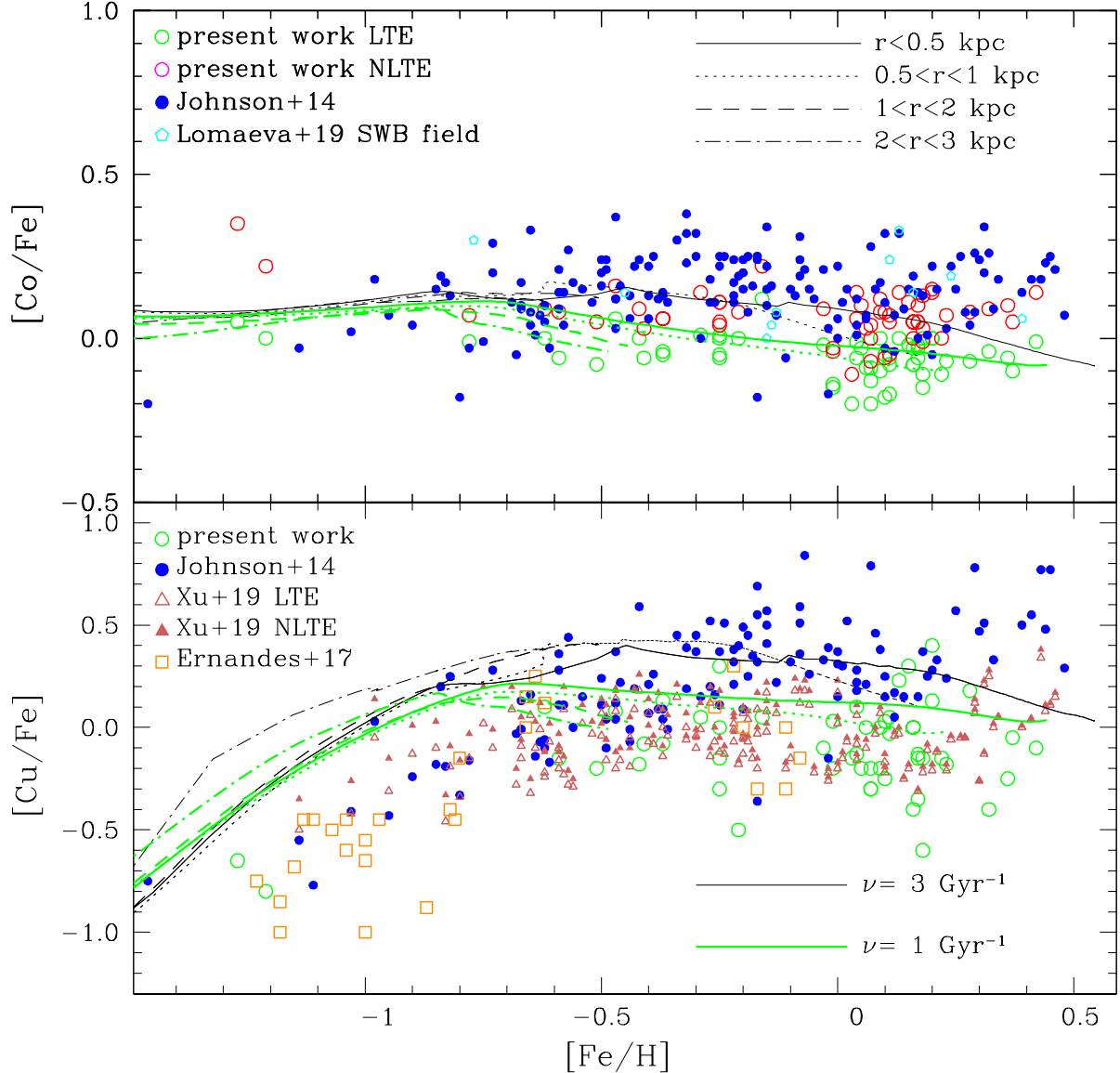
Fig. 3. Upper panel: [Co/Fe] vs. [Fe/H] with the present results in LTE and corrected for NLTE, together with literature data. Lower panel: [Cu/Fe] vs. [Fe/H] with the present results and literature data. Shown are: the present results in LTE (open green circles); present results in NLTE (open magenta circles); Johnson et al. (2014) (filled blue circles); Lomaeva et al. (2019) for the SW field (open cyan circles); Xu et al. (2019) in LTE (open Indian red triangles); Xu et al. (2019) in NLTE (filled Indian red triangles); Ernandes et al. (2018) for bulge globular clusters (open dark orange squares) and chemodynamical evolution models are overplotted; specific star formation rates of 3 \text{ Gyr}^{-1} , with SNII yields from WW95 (black lines); specific star formation rates of 1 \text{ Gyr}^{-1} , with SNII yields from WW95 and from Kobayashi et al. (2006) for [Fe/H] < -4.0 (green lines). Models are for distances to the Galactic center of: r < 0.5 \text{ kpc} (solid lines), 0.5 < r < 1 \text{ kpc} (dotted lines), 1 < r < 2 \text{ kpc} (dashed lines), and 2 < r < 3 \text{ kpc} (dash-dotted lines).
