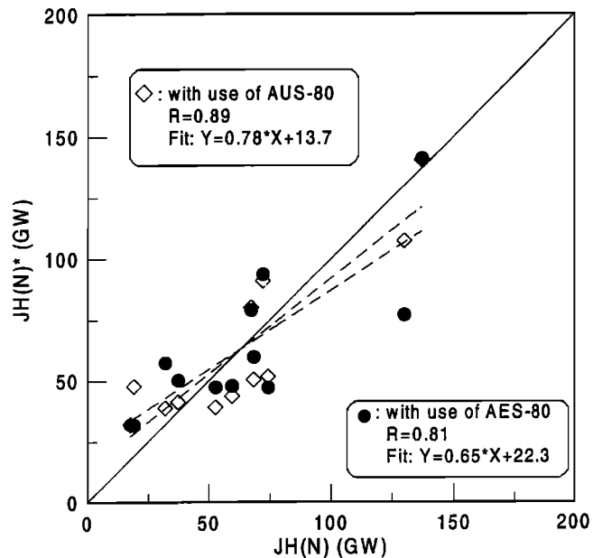
Figure 3. Scatterplot of data points (averaged over 12-hour intervals) of JH(N)* estimated using AES-80 and AUS-80 parameters versus JH(N) determined by the AMIE procedure. The dashed lines correspond to the best fits for the two groups of data. The correlation coefficients R and the equations of the fits are indicated. The solid line corresponds to the ideal case JH(N)*=JH(N).
