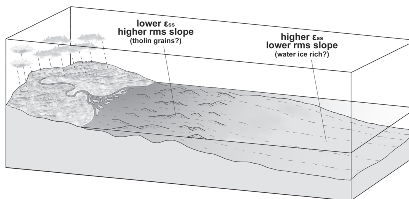
Figure 7. Model scenario of a river culminating in a liquid body. The flow deposits larger-dimension particulates close to the river terminus while more distant seafloor areas remain unaffected.
