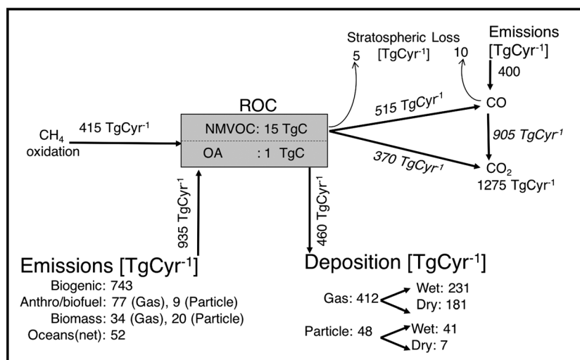
Figure 3. The global reactive organic carbon (ROC) 2010 tropospheric budget simulated with GEOS-Chem. Values in italics were derived assuming the total budget is in steady state.
