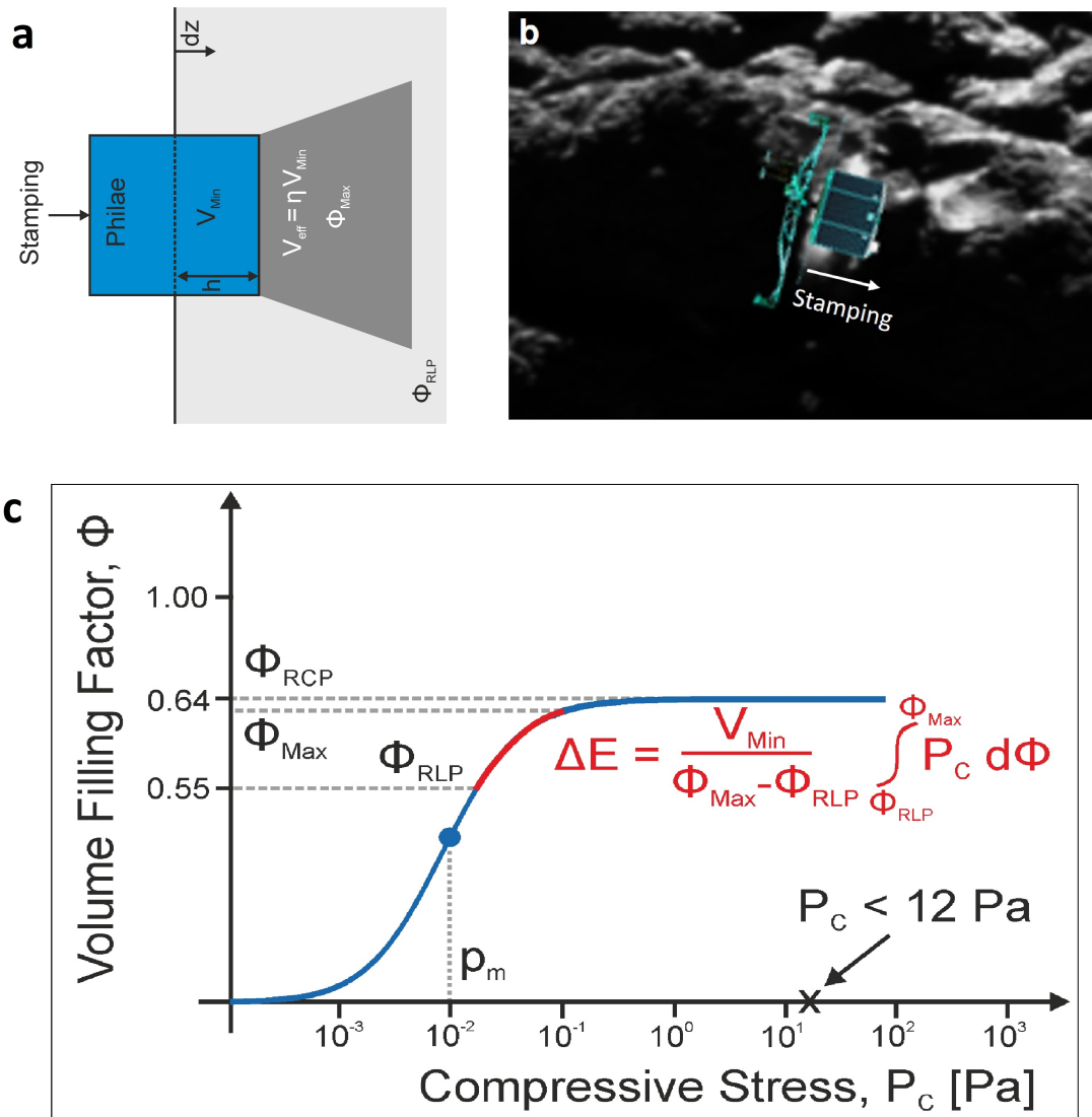
Extended Data Fig. 6 : Philae Interaction geometry and Boulder volume-filling factor. a Interaction geometry of Philae with the ice/dust at moment of deepest penetration in TD2c. b Philae superimposed on OSIRIS image (2 nd September 2016) showing equivalent interaction geometry as in a . c Compressive stress curves for a hierarchical makeup. Note the volume-filling factor \Phi denotes packing of porous pebbles only; these are then further packed to make up the whole boulder. See Methods for detailed explanation.
