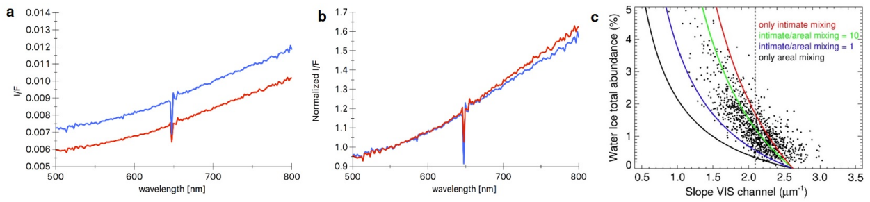
Extended Data Fig. 4 VIRTIS water ice analysis plots – Average I/F of skull-top boulder location (blue curve) and on the nearby dark terrain (red curve) before (plot a) and after (plot b) normalization at 550 nm. Plot c : theoretical abundance of water ice as a function of the spectral slope in the visible spectral channel 43 . Black dots and dashed lines indicate a water ice rich region observed by VIRTIS to calibrate the theoretical curves. The x-axis values correspond to slope values scaled to the dark terrain unit viewing conditions (Fig 3b. panel b1 red box) for observation V1_00424522185.QUB.
