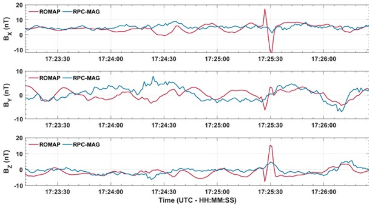
Extended Data Fig. 5 Combined ROMAP and RPC-MAG magnetic field and boom measurements. The three components of the magnetic field observations are shown starting before TD2 at 17:23:00 UTC and ending shortly after the boom movement was detected. This figure also shows the concurrent orbiter RPC-MAG observations as reference. See Methods and Supplementary Methods section 7 for detailed description.
