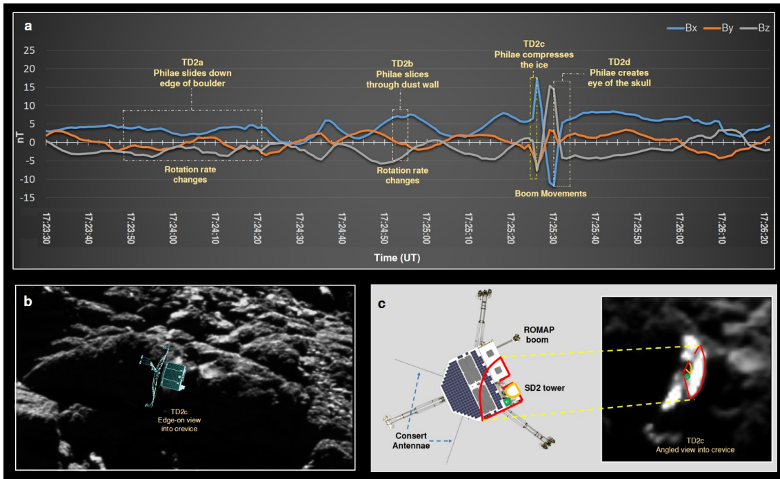
Fig. 2 A ROMAP guide and Philae impacts TD2c : Panel a shows the ROMAP magnetometer rotation/boom measurements matching Philae touchdown events versus time (see Methods and Supplementary Methods). OSIRIS Image b focusses on TD2c where the lander compressed the ice in the crevice (2 nd September 2016). Image c shows an overhead view of the Philae lander highlighting its instruments. The red, orange and green markings map to the impression in the ice (OSIRIS image 24 th August 2016). See Supplementary Video 2 showing a fly-over of the crevice and Supplementary Video 3 for an animation of this current figure.
