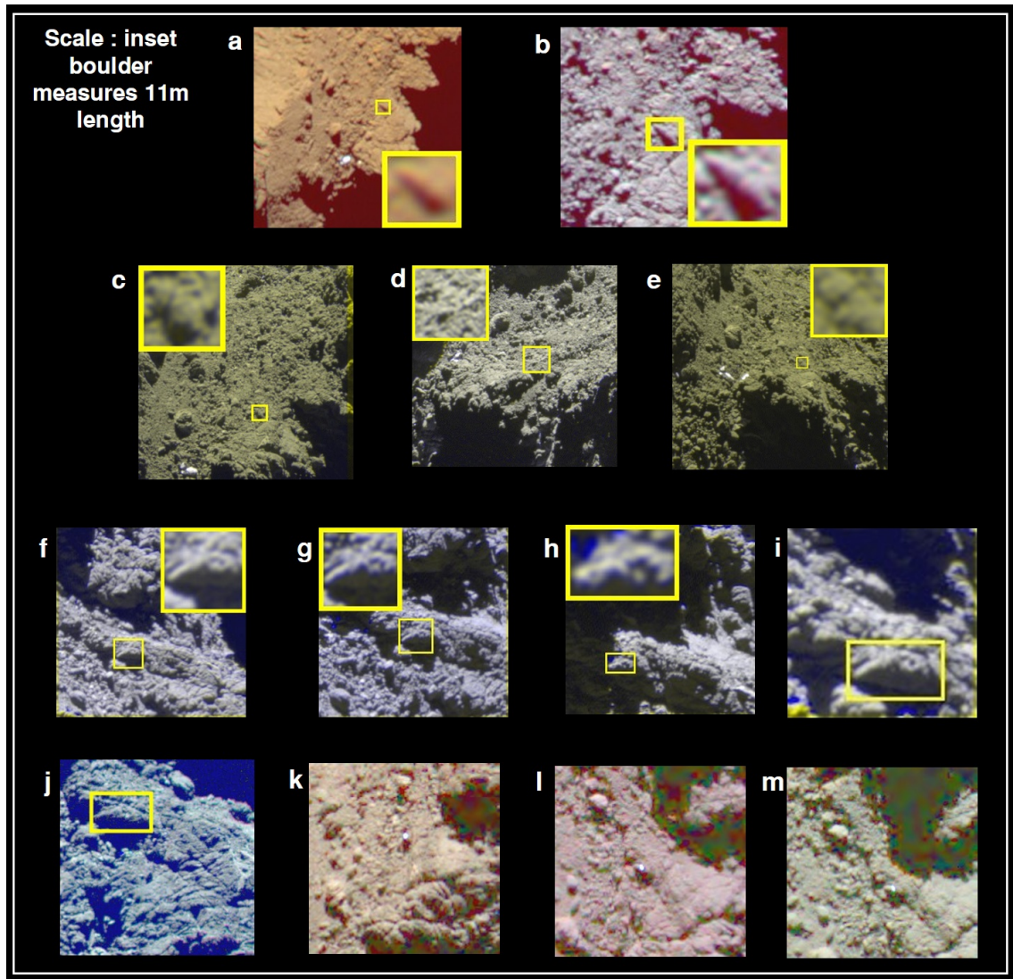
Extended Data Fig. 2 OSIRIS Colour composites of skull-top boulders Images a & b Pre-landing images of “skull-top” boulders (inset); RGB setting: “green”= F24 (480.7 nm), “red”= F22 (649.2 nm), “blue”= F16 (360.0 nm). Images c-e “skull-top” boulders observed December 2014; RGB setting: “green”= “red”= F22 (649.2 nm), “blue”= F24 (480.7 nm). Images f-i The “skull-top” boulders observed in March 2016; RGB setting: “green”= “red”= F22 (649.2 nm), “blue”= F24 (480.7 nm).. Images j-m Color composite of the “skull-top” boulders in early and mid-June 2016; RGB setting: “green”= F24 (480.7 nm), “red”= F22 (649.2 nm), “blue”= F16 (360.0 nm).
