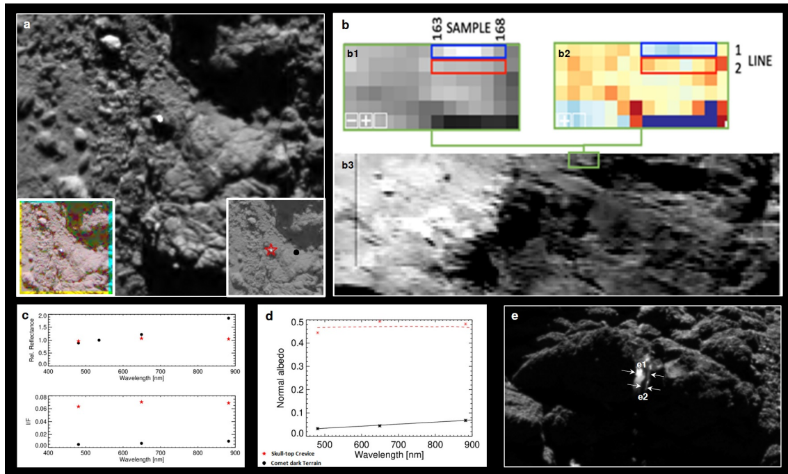
Fig. 3 Multi-instrument view of the water ice. a OSIRIS inset-images (left : multi-filter view, right : star and black dot position for plots c,d) within NAC image (14 th June 2014 10:29UT). b 0.55 μm VIRTIS-M Hyperspectral cube (V1_00424522185.QUB) of the Abydos region (14° June 2016 10:51-11:35 UT) with skull-top ridge located in the green box. The inset panels zoom on spectral slope (left) and I/F image (right). c plot of reflectance and I/F versus wavelength and d the measured albedo. OSIRIS Image e (2nd Sept 2016) shows the crevice edge-on with e1 (crevice width) 1.03 \pm 0.07 m and e2 (compression width) 0.246 \pm 0.049 m.
