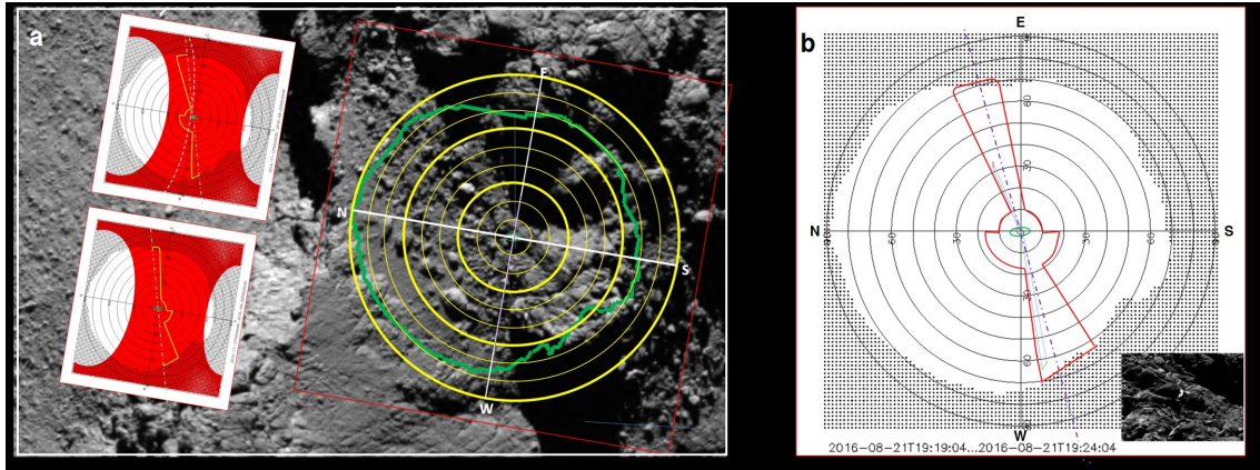
Extended Data Fig. 3 Skull-top crevice illumination geometry. a Transparent overlay of the azimuth plots from the insets on a 12 th June 2016 OSIRIS NAC image. The red highlight is the sun illumination from Philae landing to end of mission. Each concentric circle represents 30 degrees azimuth. The green line maps the edge of the sun illumination. The yellow line shows the crevice horizon mask. b 21 st August 19:19-19:24 azimuth plot with red-lined horizon mask of skull-top crevice. Inset OSIRIS image from that date/time shows crevice is illuminated. Red dot is sun angle and green dot is Rosetta viewing angle
