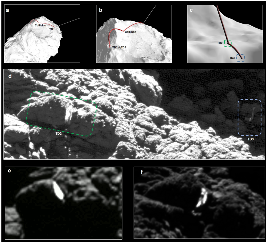
Fig. 1 – Philae landing trajectory, TD2 and Philae, Visible ice. Images a , b and c : three views showing the Philae landing trajectory as it crosses the surface of the comet (shape model) highlighting the locations of Touchdown 1 (TD1), Collision, Touchdown 2 (TD2) and Touchdown 3 (TD3). OSIRIS image d (2nd Sept 2016 19:59 UT; 0.049 m/pixel) is overexposed in order to show the skull-top crevice and the Philae lander hidden in the distant shadows. Images e and f show views of the ice in the crevice (6 th August 2016 and 24 th August 2016 respectively).
