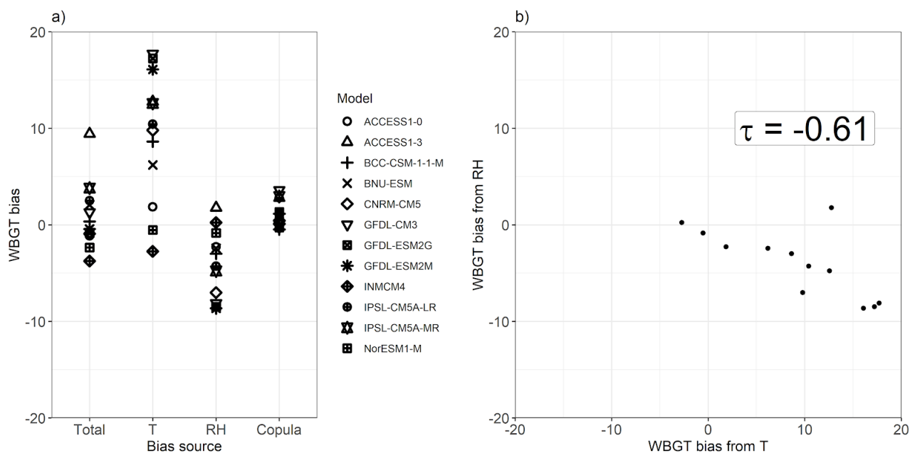
615 Figure 9: Spread of mean total bias in the 95th quantile (Q95) of WBGT and its contribution from T, RH and their copula for individual CMIP5 models (a), and a scatter plot of the T and RH contributions to Q95 WBGT bias, with their respective Kendall rank correlation coefficient (p-value < 0.001). Shown are results for a grid-point in Brazil (Amazonia, 5°S and 56.5°W). Bias was calculated as (CMIP5 or Transformation - ERA-Interim).
