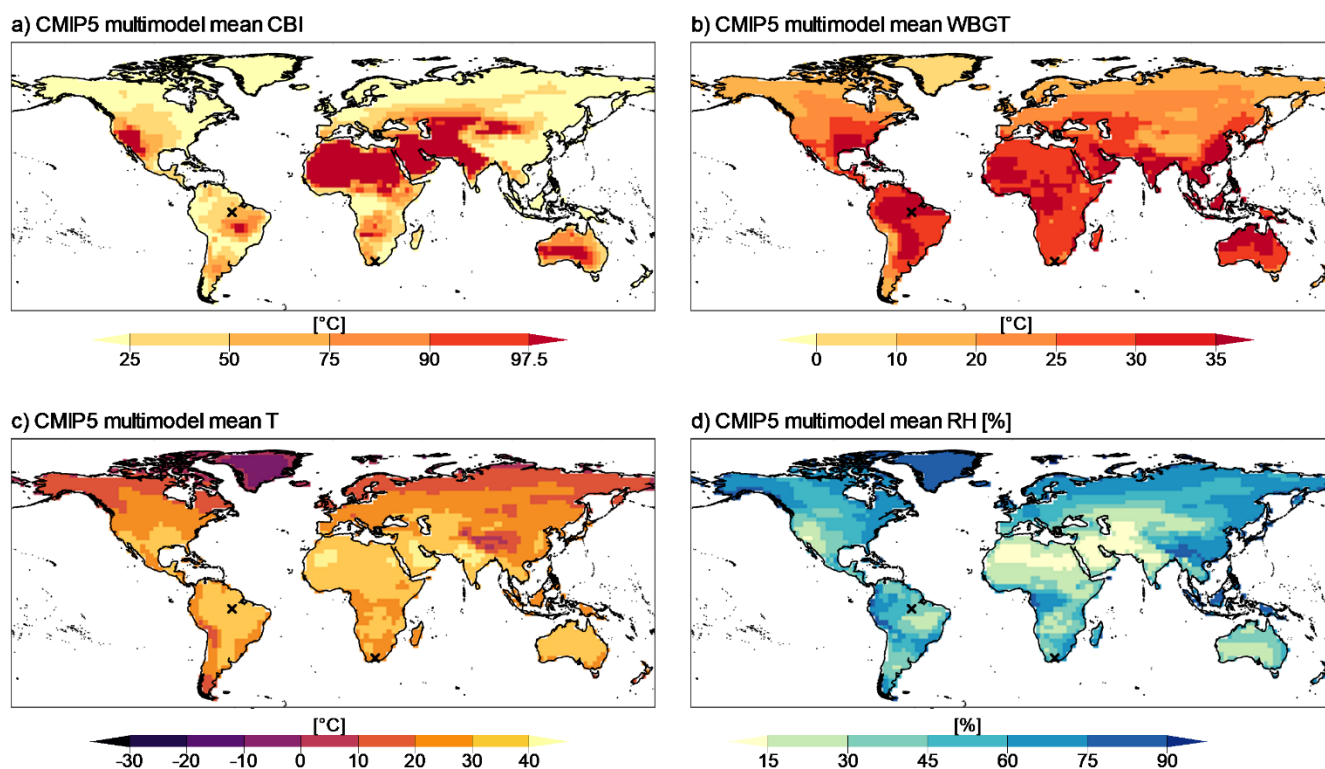
Figure A2: CMIP5 multimodel mean fire hazard index ( CBI ) value (a), heat stress index ( WBGT ) value f (b), temperature ( T ) value (c), and mean relative humidity ( RH ) (d).
