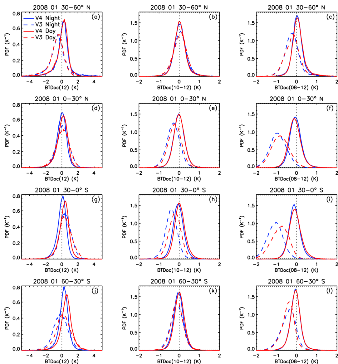
280 Figure 3: Probability density functions (PDF) of the differences between observed and computed brightness temperatures (BTDoc) over oceans in January 2008 in V4 pristine (no cleared clouds) nighttime (blue) and daytime (red) clear sky conditions in V4 (solid lines) and in V3 (dashed lines). Panels a, d, g, j: BTDoc at 12.05 \mu\text{m} . Panels b, e, h, k: 10-12 inter-channel BTDoc difference. Panels c, f, i, l: 08-12 inter-channel BTDoc difference. The PDFs are shown at 30-60° N (panels a, b, c), 0-30° N (panels d, e, f), 30-0° S (panels g, h, i), and 60-30° S (panels j, k, l).
