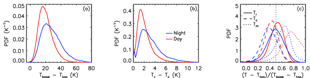
385 Figure 7: Nighttime (blue) and daytime (red) probability density functions in V4 opaque ice clouds of (a) apparent thermal thickness T_{base} - T_{top} , (b) T_r - T_c V4 correction, and (c) (T - T_{top})/(T_{base} - T_{top}) for T = T_r (solid lines), T = T_c (dashed lines) and T = T_m (dotted lines) over oceans between 60^\circ S and 60^\circ N in January 2008. Channel 12.05 \mu\text{m} .
