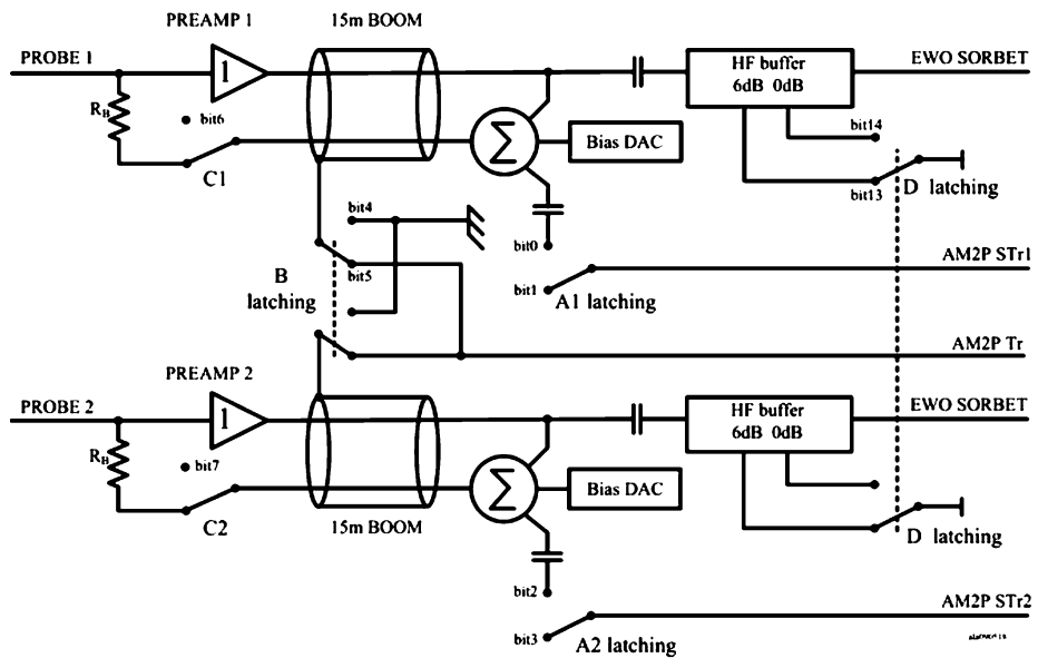
Fig. 9 Illustration of the simplified MEFISTO signal paths and controls
