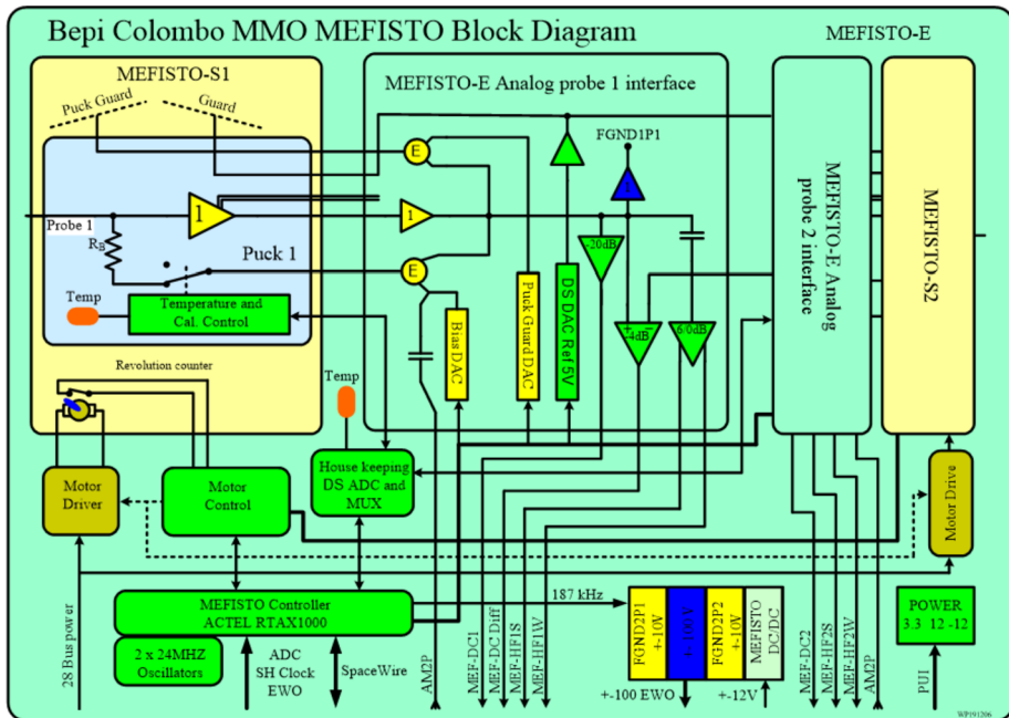
Fig. 7 MEFISTO block diagram
