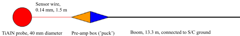
Fig. 4 MEFISTO sensor configuration. Adapted from Blomberg et al. (2006)
