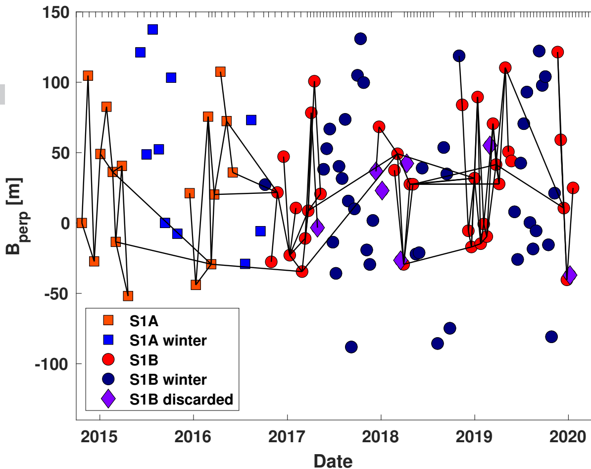
Figure 10: Perpendicular baseline ( B_{perp} ) plot for S1 SLCs from descending track 83. The time series for this track is in Figure 5g. Ticks on top of the figure show the date of the images, and clearly show the onset of 12 days acquisitions in February 2017 and several periods with data gaps. Blue squares and circles are SLCs acquired under winter conditions with snow on top of the volcano and purple circles are summer and early fall SLCs that result in interferograms with coherence loss either on top or on the vegetated flanks of the volcano. Black lines are interferograms used in the time series. The figure shows that despite the 12 day repeat period of the mission since February 2017, a significant amount of the small baseline interferograms are not useful due to their low coherence, even in the austral summer. Coherence loss was a severe problem during February 2017 - May 2018 but not as much during May 2018 - May 2019. Also, it is not straightforward to select summer to summer interferograms to ensure the connectivity of the InSAR network.
