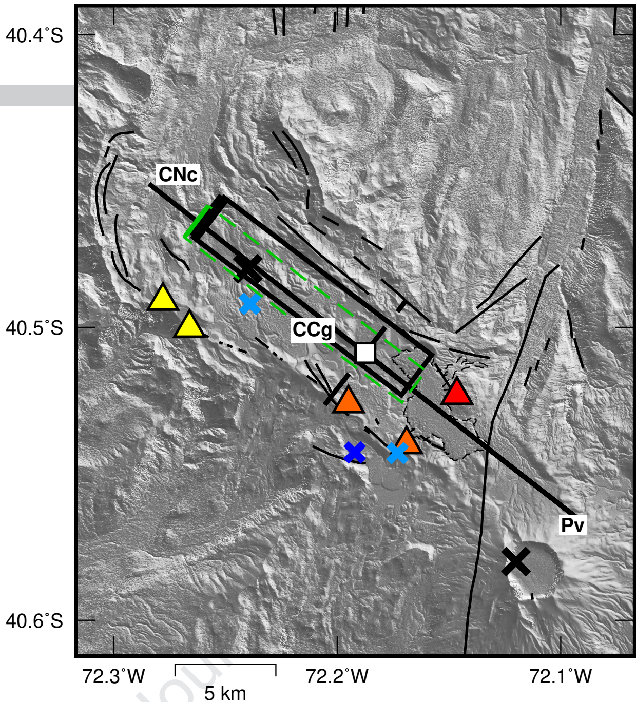
Figure 7: Compilation of deformation sources derived from InSAR inversions on top of TanDEM-X topography. The yellow, orange and red triangles are the 1921-1922, 1960 and 2011-2012 eruptive vents. The thin dashed outline is the 2011-2012 lava flow. The green rectangle is the 2003-2007 Okada source model (Figure 3, Figure S1), the light blue crosses are the 2007-2008 Mogi source model (Jay et al. , 2014), the blue cross is the 2008-2011 Mogi source model (Jay et al. , 2014), the black crosses are the Mogi sources for the first three days of the eruption (Jay et al. , 2014), the white square, thick black line and dashed black lines are the centroid, semi major- and semi-minor axes of the spheroid source model during the rest of the eruption (Figure 4, Delgado et al. , 2019), and the black square is the 2012-2017 Okada source model (Figure 5, Delgado et al. , 2018, 2016). The black lines are faults (Jay et al. , 2014)
