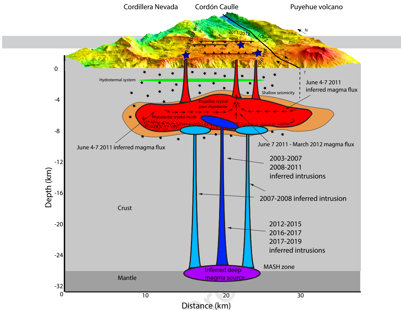
Figure 9: Cordón Caulle geological cross section (updated from Delgado et al., 2016, 2018 ) that summarizes the estimated deformation sources between 2003–2011, 2011–2012 and 2012–2019 derived from InSAR modeling and the inferred magma sources of the 1921–1922, 1960, and 2011–2012 eruptions from geobarometry ( Lara et al., 2006a ; Singer et al., 2008 ; Castro et al., 2013 ; Jay et al., 2014 ). The red region is the hypothetical mush zone, likely surrounded by a viscoelastic shell (orange region). The storage region could also be a collection of discrete, connected reservoirs instead of a large, interconnected zone. Black points in the red regions show crystals that might have settled at the bottom of the reservoir, thus reducing the magma viscosity ( Castro et al., 2013 ) and enhancing interstitial liquid extraction, a condition likely required to produce eruptible magma in a silicic magma chamber ( Bachmann and Bergantz, 2008 ; Cooper, 2017 ). The light blue regions show the inferred magma intrusion during 2007–2008, the blue region shows the inferred magma sources during 2003–2007, 2008–2011, 2012–2015, 2016–2017 and 2018–2019, and the green region is the hydrothermal system beneath the volcano ( Sepulveda et al., 2004 ; Sepulveda et al., 2007 ). Blue stars show the location of the historical eruptive vents, black stars are earthquakes beneath the volcano ( Delgado et al., 2016 ; Wendt et al., 2017 ), horizontal lines with open triangles show the graben bounding faults, and LOFZ is the Liquiñe-Ofqui regional fault zone that crosses the volcano ( Lara et al., 2006b ). MASH zone refers to a hypothetical zone of magma melting, assimilation, storage, and homogenization ( Hildreth and Moorbath, 1988 ) that I infer to be the source of magmas (see rationale in Jay et al., 2014 ). The sketch shows that the source of the 1921–1922, 1960, and 2011–2012 eruptions is the same reservoir located beneath Cordillera Nevada, Cordón Caulle, and Puyehue volcanoes and where magma intruded during 2003–2007, 2007–2008, 2008–2011, 2012–2015, 2016–2017 and 2017–2019. InSAR data are interpreted to show that magma flowed from the Cordillera Nevada and Puyehue volcanoes towards the 2011–2012 eruptive event during the first three eruption days and then flowed from the same area where magma injection occurred afterwards. Note that the shape of the crystal mush is hypothetical because no geophysical imaging is available for the volcano.
