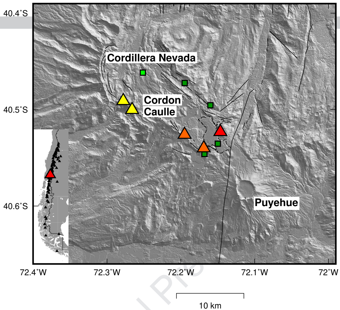
Figure 1: Cordón Caulle location map draped over the 12 m TanDEM-X shaded topography. The yellow, orange and red triangles are the 1921-1922, 1960 and 2011-2012 eruptive vents. The black dashed outline is the 2011-2012 lava flow and the black lines are faults ( Jay et al., 2014 ). Green squares are hot springs and fumaroles and the light green square is the Trahuilco geyser ( Sepulveda et al., 2004 ). All the eruptive vents are located in the NW-SE direction faults that bound the Cordón Caulle graben. The inset shows the location within South America, where the black and red triangles are Holocene volcanoes and Cordón Caulle.
