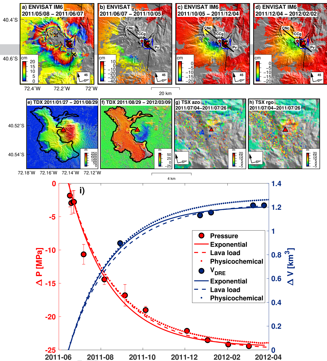
Figure 4: Summary of InSAR observations of subsidence during the 2011-2012 eruption. a-d) Ground subsidence recorded by four ENVISAT interferograms. The data span the first three days of the eruption (a) (modified from Jay et al., 2014 ), day three to 4 months (b) (modified from Jay et al., 2014 ), four to six months (c), six to eight months (d). Interferogram a) is presented wrapped with one fringe equivalent to 20 cm of ground deformation to highlight \sim 1.3 m and \sim 0.3 m of subsidence at Cordillera Nevada caldera (CNc) and Puyehue volcano (Pv). The best-fit Mogi sources for a) are the two black crosses circles and the best-fit Yang source for b-d) is the white square with the black thick lines that show the spheroid semi-major and minor axes. The circles in a) and the red circle in b-d) show the location of the time series in Figure 2 . The red triangle is the eruptive vent. The dashed blue square shows the area of e-h). TanDEM-X differential DEMs that span from the beginning of the eruption to August 2011 (e) and August 2011 to March 2012 (f). Azimuth (azo, g) and range offsets (rgo, h) that record more than 10 m of post-emplacment deformation in the area of the shallow laccolith. i) Time series of pressure drop (red circles) and intruded laccolith and extruded lava flow volume (blue circles) during the effusive phase of the eruption with fits for three different eruption models (modified from Figure 8 of Delgado et al., 2019 ). Here exponential refers to an analytic model of reservoir depressurization and lava effusion whose solution is an exponential function ( Equation 1-Equation 2 ). Lava load is a numerical model that incorporates the effects of the lava load onto the reservoir force balance ( Mastin et al., 2008 ). Physicochemical is a numerical model that incorporates both the lava load effect and the H 2 O and CO 2 exsolution in the reservoir ( Anderson and Segall, 2013 ; Delgado et al., 2019 ).
