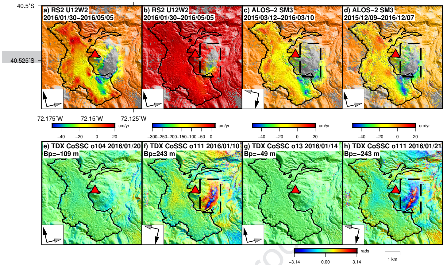
Figure 6: a-d) Mean ground velocity at the lava flow during a period with no deformation of magmatic origin. a-b) Mean ground velocity from a RADARSAT-2 Wide Ultra Fine 12 stack during February - May 2016. a) and b) show the same data but with different color scales to highlight deformation in the lava flow and in the laccolith respectively. The dashed black box shows the area of the laccolith. c-d) ALOS-2 SM3 interferograms that span one year showing mean ground velocity. e-h) TanDEM-X differential bistatic interferograms with the reference topographic phase removed with the 12m TanDEM-X DEM from 2011-2014. Here B_p is the perpendicular baseline. The dashed black box shows the area of the laccolith with a DEM error which propagates into subsidence with a high rate of 3 m/yr in the RS2 stack. The black and grey arrows show the satellite heading and LOS direction. The red triangle is the 2011 eruptive vent. The black thick line is the lava flow contour ( Bertin et al., 2015 ).
