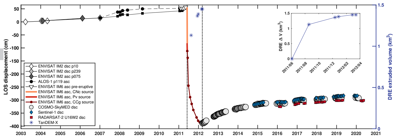
Figure 2: Compilation of line-of-sight (LOS) ground displacement from InSAR time series between 2003 and 2020 for selected pixels, including the 2011-2012 eruption (vertical dashed lines). The figure combines data from different orbits and viewing geometries because there is no single data that spans the whole sequence of unrest. The different data sets have been shifted by a constant so they lie approximately on top of each other for a better visual comparison. This also give the time series a qualitative continuity. Data location in Figure 3a-b and Figure S1 for ENVISAT IM2 (Image Mode 2) 2003-2007, Figure 3c,d for ALOS-1 2007-2011, Figure 3e for ENVISAT IM6 (Image Mode 6) pre-eruptive, Figure 4a,b for ENVISAT IM6 CNC (Cordillera Nevada caldera), Pv (Puyehue volcano) and CCg (Cordón Caulle graben) sources, Figure 6a,g,h for COSMO-SkyMED, Sentinel-1 and RADARSAT-2. Asc/dsc refers to ascending and descending data respectively. p10, p239, p075 and p119 refers to ENVISAT IM2 paths 10, 239 075 and ALOS-1 path 119. ENVISAT IM6 pre-eruptive time series by Reath et al., 2019 . COSMO-SkyMED, RADARSAT-2 and Sentinel-1 time series updated from Delgado et al., 2018 . Right axis and inset show dense rock equivalent (DRE) lava flow extruded and laccolith intruded volume from TanDEM-X differential DEMs ( Delgado et al., 2019 ). ENVISAT IM6 time series for CNC and Pv sources were calculated adding the maximum displacement produced by each one as recorded in Figure 4a. ENVISAT IM6 time series for CCg source was calculated for the point of maximum LOS predicted by the best-fit prolate spheroid model because there is no coherence on top of the volcano during more than half of the eruption ( Delgado et al., 2019 ).
