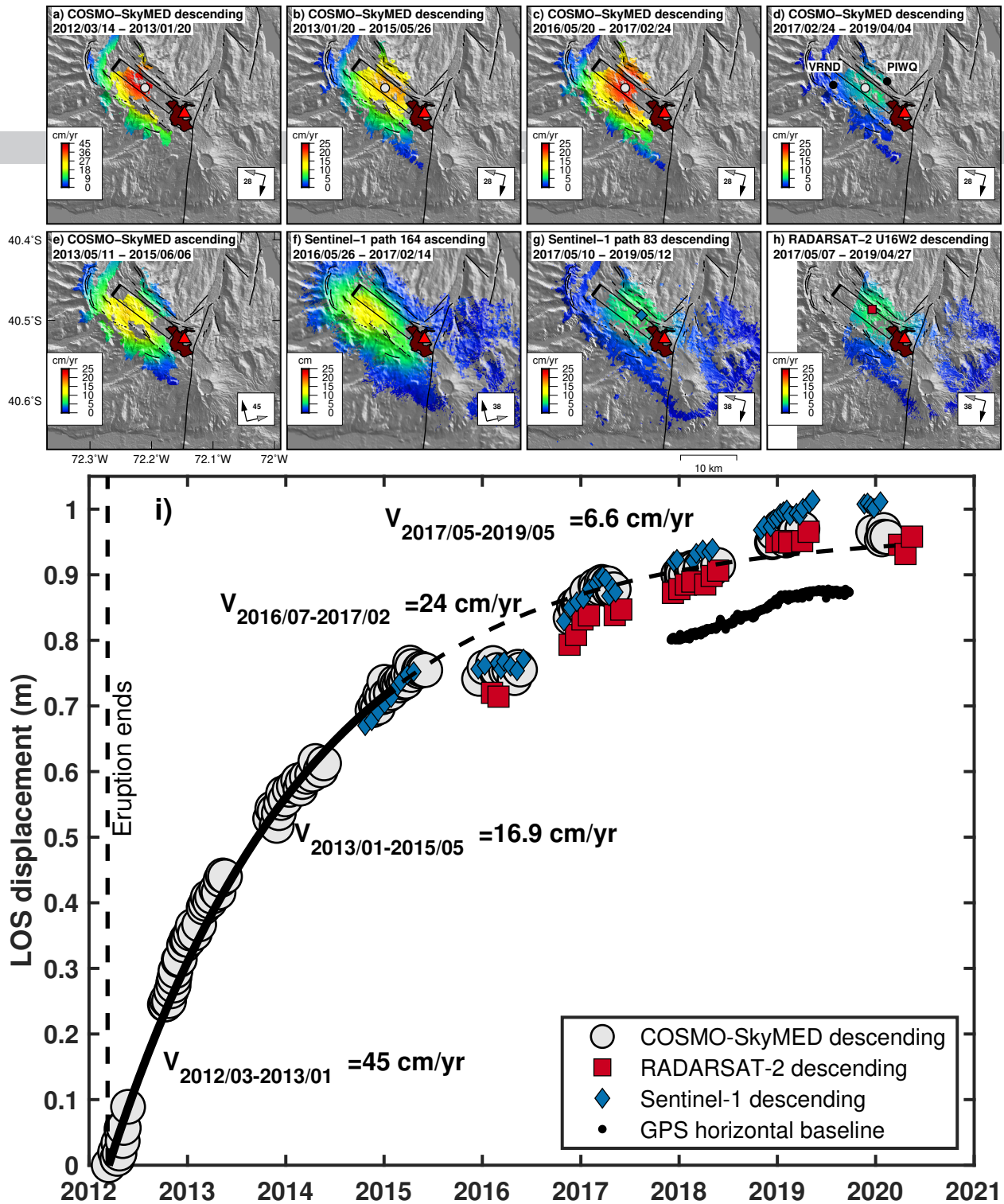
Figure 5: Summary of InSAR observations of post-eruptive LOS ground uplift between 2012 and 2020. Mean ground velocity recorded by a-d) CSK descending 2012-2019, e) CSK ascending 2013-2015, f) S1 ascending 2016-2017, g) S1 descending 2017-2019 and h) RS2 descending 2017-2019. Data in a,b,e) from Delgado et al., 2016 and data in c,f) modified from Delgado et al., 2018 . d,g,h) show new data. Note that c) and f) cover the same time span, but are plot with different color scales because c) is a mean velocity and f) shows the cumulative displacement during the 6 months of this uplift event. The black rectangle is the best-fit tensile dislocation with uniform opening during the 2012-2017 time span ( Delgado et al., 2016 ). The black circles in d) are the GPS stations installed in December 2017. The brown outline and the red triangle are the 2011-2012 lava flow and eruptive vent respectively. i) Descending time series of ground deformation for selected pixels for CSK (grey circles in a-d), S1 (blue diamond in g) and RS2 (red square in h). The data shows three pulses of uplift during March 2012 - May 2015, July 2016 - February 2017 and May 2017 - May 2020. The data sets have been shifted by an arbitrary constant so they approximately lie on top of each other to simplify the geologic interpretation. The GPS data are the horizontal baseline change between the two stations located on both sides of the volcano (d). The black thick line is an exponential fit to the 2012-2015 CSK data and is indicative of magma injection. The dashed black line is the exponential fit to the 2012-2015 CSK data extrapolated until 2020.
