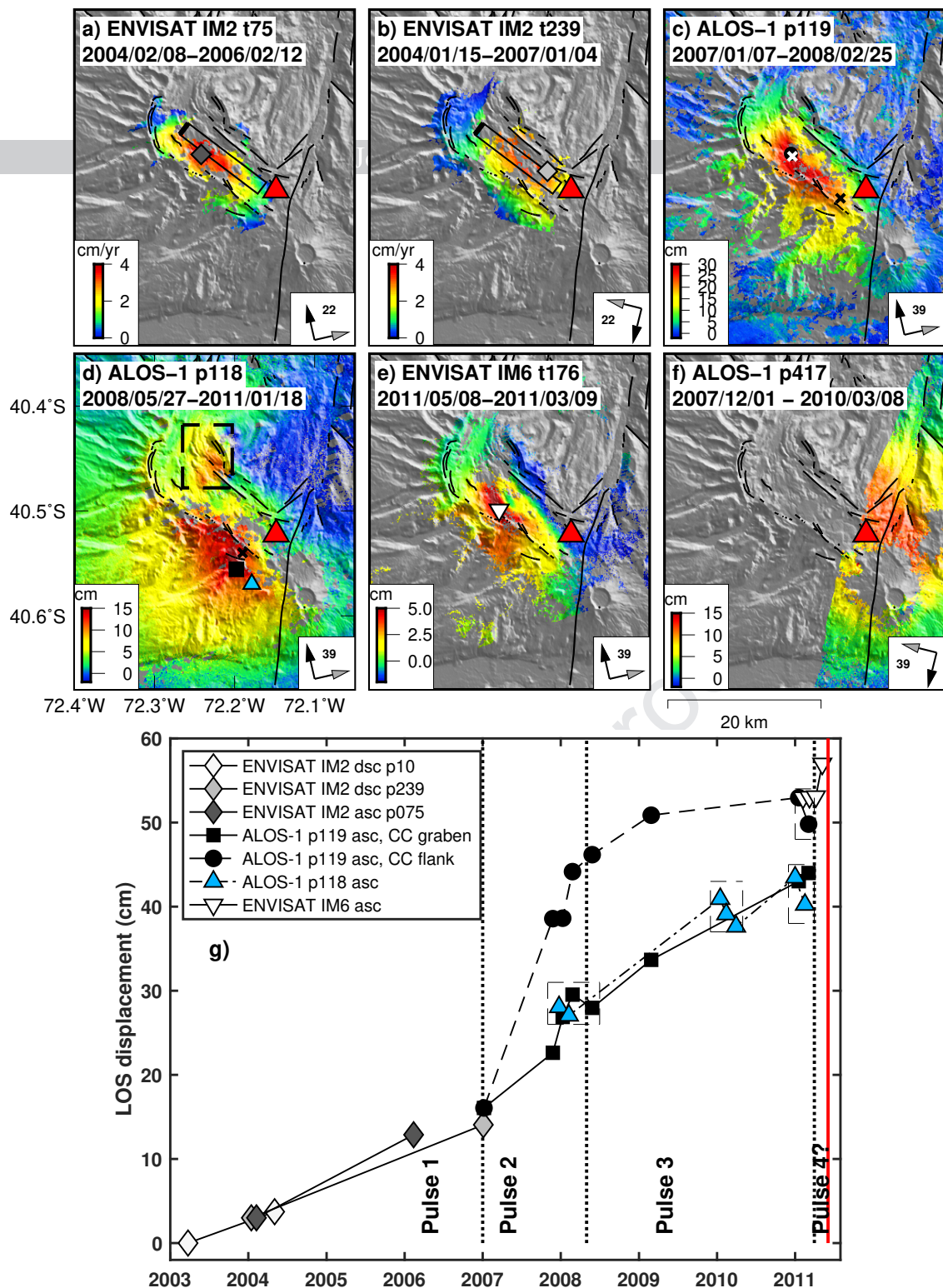
Figure 3: Summary of InSAR observations of pre-eruptive LOS uplift between 2003 and 2011. a-f). All panels show LOS ground deformation with the respective deformation sources and the 2011-2012 eruptive vent (red triangle). a-b) show interferograms converted to mean ground velocity while c-f) show the cumulative ground deformation. In each panel the black and grey arrows show the satellite heading and horizontal component of the LOS vector. The number next to the arrows is the look angle. a-b) First pulse of uplift during 2003-2007 with a rate of \sim 3\text{-}4 cm/yr. The black square is the contour of the best-fit sill model. c) Second pulse of uplift during 2007-2008 with a total displacement of \sim 30 cm. The crosses show the best-fit Mogi sources. d, f) Third pulse of uplift during 2008-2011 with a total displacement of \sim 15 cm. The dashed line is the area near the Trahuilco geyser in February - March 2010 that uplifted likely triggered by the 2010 Maule earthquake. The cross shows the best-fit pressurized Mogi source. e) Potential fourth pulse of uplift during early 2011 with a total displacement of \sim 5 cm. f) Descending ALOS-1 interferograms that shows the end of the second pulse of uplift and the third pulse of uplift. g). Time series of ground deformation calculated for the pixels of the same color and symbol in the upper panel and Figure 2. The time series were shifted by an arbitrary constant as in Figure 2. Rate map for ALOS-1 p118 asc is not shown in the figure. ENVISAT IM6 time series for early 2011 by Reath et al., 2019 . The dashed lines show localized atmospheric signals that are non-stationary across the scene, and therefore cannot be corrected with an empirical correction that correlates the phase and the topography across the interferogram.
