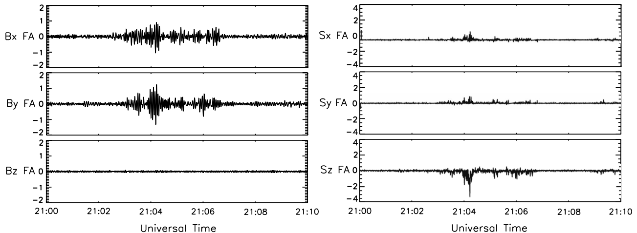
Figure 3. (a) Bandpass-filtered (0.1–0.4 Hz) plot of magnetic field data in nanoTeslas obtained by Cluster 4, in field-aligned coordinates, from 2100 to 2110 UT 30 September 2003. (b) Poynting vectors in field-aligned coordinates, in Watts/km 2 , for this same time interval.
