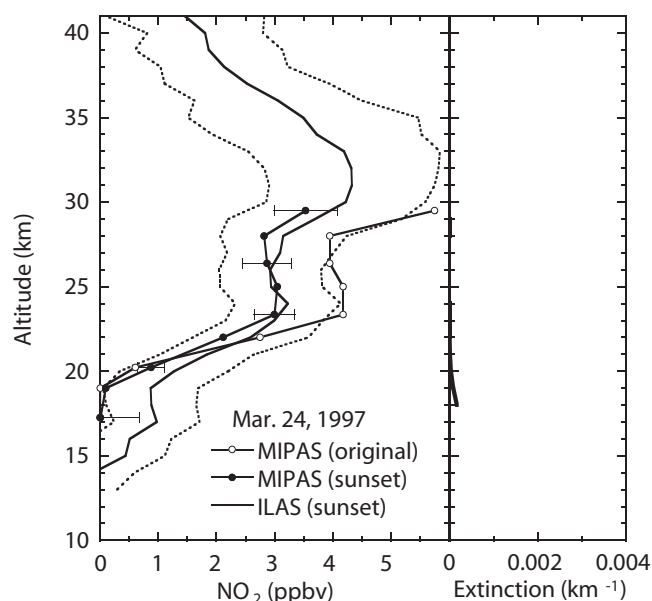
Figure 4. Same as Figure 1, but for the comparison with the MIPAS-B2 NO 2 measurements on 24 March 1997. The original balloon-borne NO 2 profile (SZA \sim 105^\circ ) is shown by the line with open symbols for reference.
