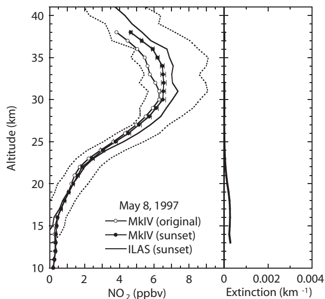
Figure 5. Same as Figure 1, but for the comparison with the MkIV NO 2 measurements on 8 May 1997. The original balloon-borne NO 2 profile (SZA \sim 90^\circ in the morning) is shown by the line with open symbols for reference.
