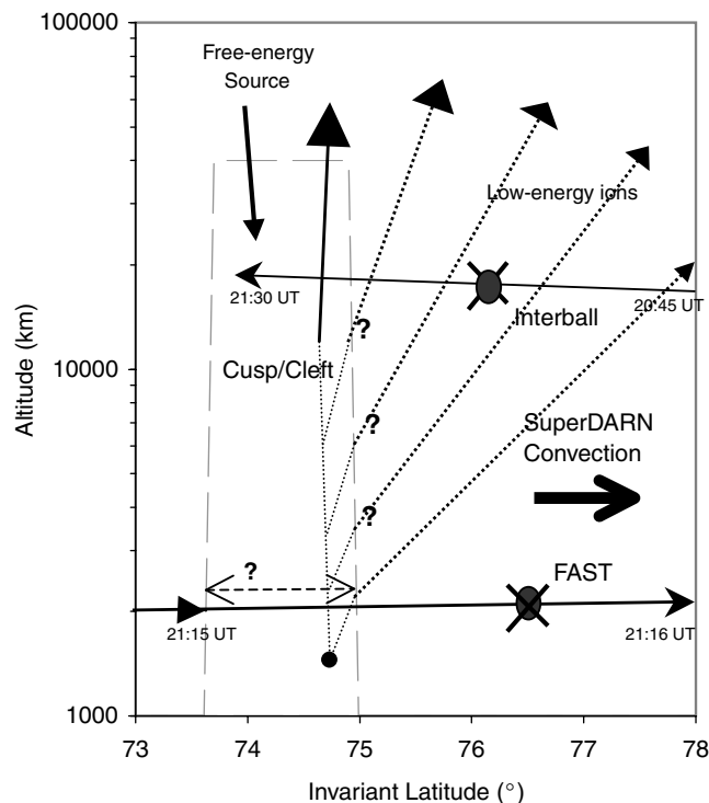
Figure 1. A sketch showing the coincidence between Interball 2, Fast Auroral Snapshot (FAST), and Super Dual Auroral Radar Network (SuperDARN) radar measurements. The trajectories are projected in the noon-midnight meridian plane and are given as functions of invariant latitude and altitude.
