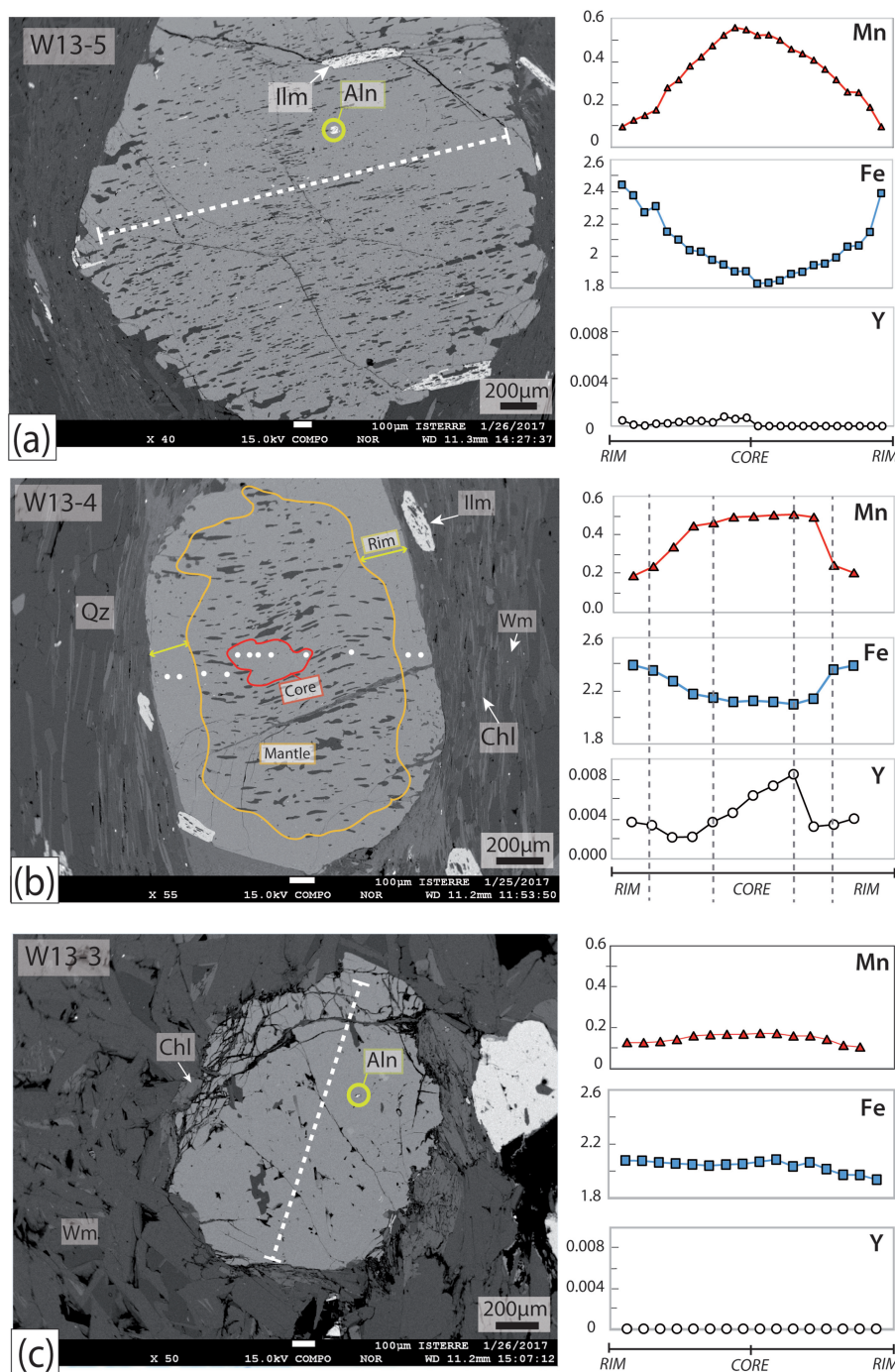
Fig. 4. Representative chemical analyses of garnet in samples w13-5 (a), w13-4 (b) and w13-3 (c). Left column: BSE images of analyzed garnet porphyroblasts. In sample w13-5 analyses were acquired along the profile (white dashed line) after each 110 \mu\text{m} , and in sample w13-4 after each 80 \mu\text{m} . The distance between point analyses in the garnet of sample w13-4 (white dots) varies to avoid Qz inclusions. Right column: Mn, Fe and Y (a.p.f.u.) contents measured along the profiles and points.
