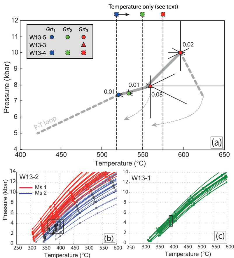
Fig. 6. Thermobarometric results. (a) P - T conditions of garnet growth in samples w13-5, w13-4 and w13-3 calculated using the GR T Mod fraction crystallization model. Grt 1 , garnet core; Grt 2 , garnet mantle; Grt 3 , garnet rims. Errors (continuous black lines) are estimated using the auto-refinement procedure provided in GR T Mod and a residual variation ( C_0 ) of \pm 1.5 corresponding to the uncertainty resulting from the EPMA chemical analyses. Continuous grey line is the P - T loop retrieved from garnet conditions used for the modeling of Fig. 7. Grey dashed line is the extrapolated portion of the P - T loop used following Airaghi et al. (2017b). (b, c) P - T lines for white mica in retrogressed samples w13-2 and w13-1 calculated with the multi-equilibrium approach. Black frames: P - T conditions of the greenschist assemblages. Black crosses in (b) represent the equilibrium conditions calculated simultaneously for pairs of white mica and chlorite analyses in sample w13-2.
