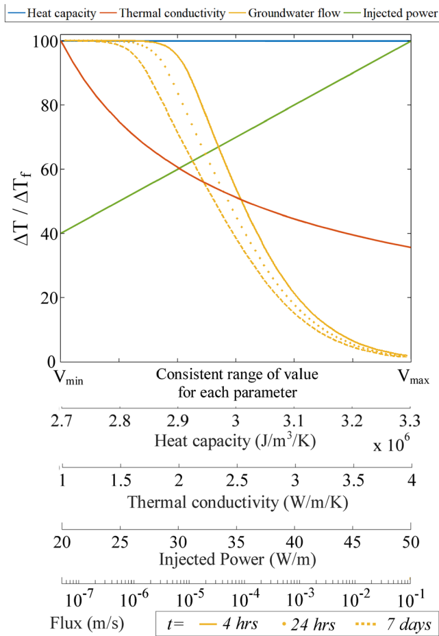
Figure 11. Sensitivity of the thermal response to the different parameters. For each parameter, the thermal response was calculated with the MILS model by fixing parameters to reference values ( Q = 35 W/m; \lambda = 1.4 W/m/K; C = 3 \times 10^6 J/m 3 /K; q = 2 \times 10^{-5} m/s, and t = 4 h) and by varying one of the parameters over a realistic range. The dotted and dashed yellow curves correspond respectively to heating periods of 24 h and 7 days. MILS, Moving Instantaneous Line Source.
