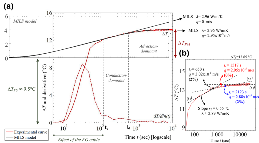
Figure 9. (a) Interpretation of the thermal response curve (red solid line) obtained during the second day of the experiment ( q = 2.95 \times 10^{-5} \text{ m/s} ). The dotted red line represents the log-time derivative of temperature. The temperature rise was matched with the MILS model (black lines) (Equation 7a) for q = 0 \text{ m/s} (for t < t_c ) and q = 2.95 \times 10^{-5} \text{ m/s} (for t > t_c ). In the MILS model (Equation 7a), the distance ( x, y ) between the heat source and the measurement point was fixed to x = 1.9 \times 10^{-3} \text{ m} and y = 0 \text{ m} , considering flow in the y direction, with x the effective radius of the FO cable used during the experiment and measured using an electronic caliper. (b) Application of the proposed graphical method based on the recognition of three characteristic times allowing the estimation of groundwater flux. The percentage of error of q estimates obtained from the three characteristic times compared to the experimental measurement of q is indicated. The graph highlights the last part of the temperature curve to better show characteristic times. MILS, Moving Instantaneous Line Source; FO, fiber optic.
