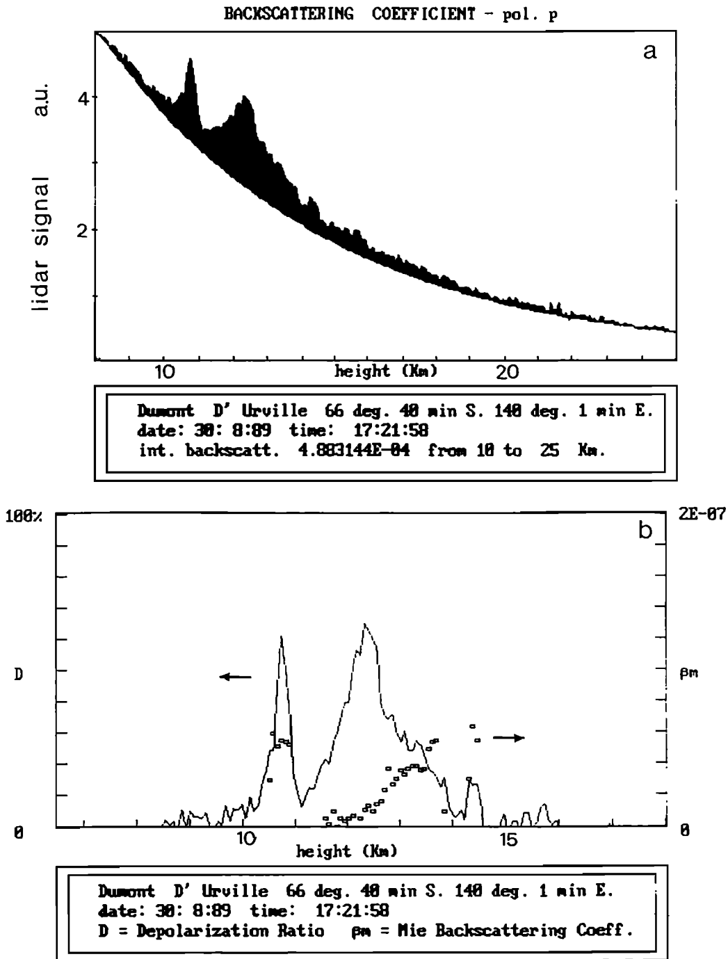
Fig. 11. (a) Backscattering coefficient in the p-polarization plane versus altitude as measured on August 30, 1989. (b) Depolarization ratio versus altitude.
