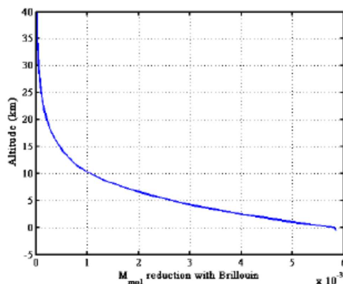
Fig. C1 Reduction of M_{mol} caused by the Brillouin effect
