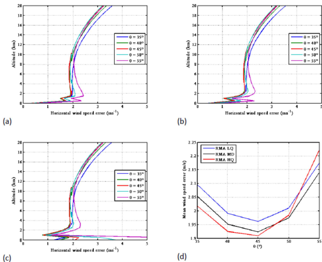
Fig. 7 (a, b, c) HLOS wind speed statistical error as a function of altitude for LOS angles between 35° and 55°, for Lower Quartile, Median, Higher Quartile RMA aerosols distribution respectively. (d) HLOS wind speed error averaged between 0.5 and 15 km in altitude as a function of LOS angle.
