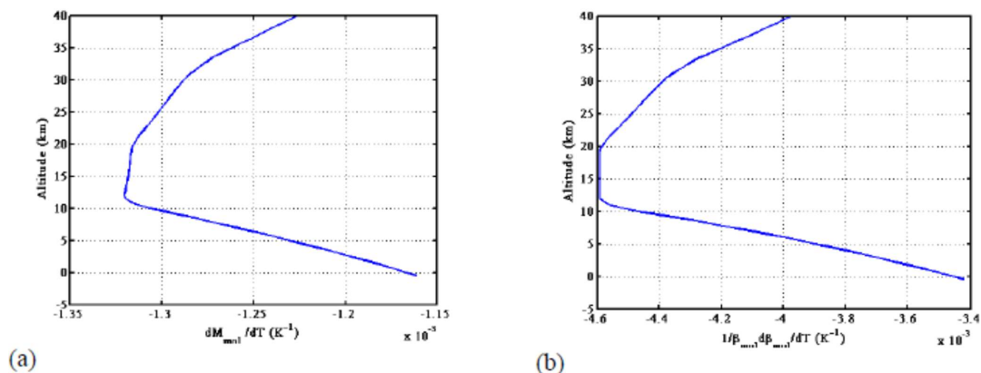
Fig C2 Temperature modeling sensitivity for (a) M_{mol} and (b) \beta_{mol}
