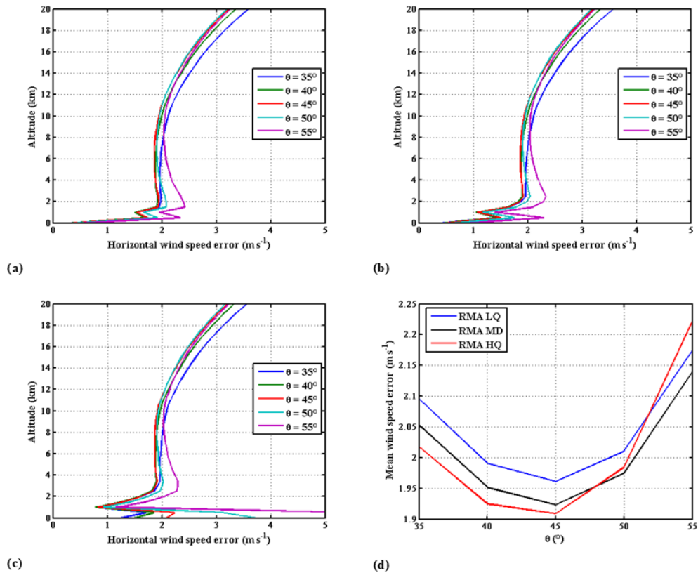
Figure 7. (a, b, c) HLOS wind speed statistical error as a function of altitude for LOS angles between 35 and 55°, for lower quartile, median, and higher quartile RMA aerosols distribution, respectively. (d) HLOS wind speed error averaged between 0.5 and 15 km in altitude as a function of LOS angle.
