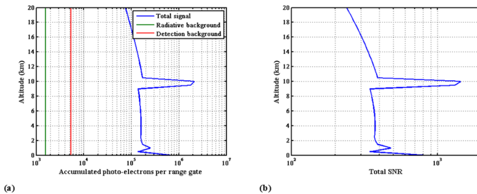
Figure 5. (a) Number of accumulated photo-electrons per range gate. (b) SNR for RMA MD backscatter profile plus cirrus at 45° LOS angle.
