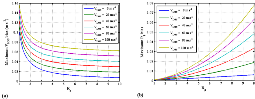
Figure 12. Maximum measurement bias for a 10^{-3} relative calibration error in the sensitivity a_i of one QMZ channel, as a function of the scattering ratio. (a) LOS velocity error. (b) Scattering ratio relative error for different LOS velocities ( V_{\text{LOS}} ).
