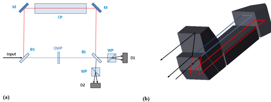
Figure 2. (a) QMZ schematics. BS – beam splitter; M – mirror; CP – field compensation plate; QWP – quarter-wave plate; WP – Wollaston polarizer; D1 and D2 – A-CCD detectors. (b) MZ actual prism arrangement (QWP, WP, and detectors are not shown here).
