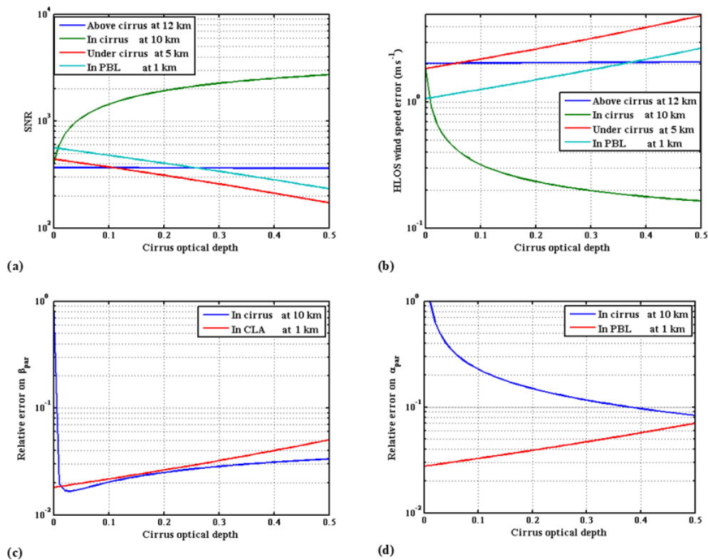
Figure 11. (a) SNR, (b) HLOS wind speed error, (c) \beta_{\text{par}} relative error, and (d) \alpha_{\text{par}} relative error as a function of the cirrus vertical optical depth for different measurement altitudes.
