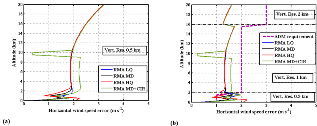
Figure 8. Vertical profile of the horizontal wind speed error (standard deviation) for different backscatter profiles, i.e., LQ, MD, HQ, and MD plus cirrus for the optimal parameters \Delta = 3.2 cm and \theta = 45^\circ . (a) Constant vertical resolution of 0.5 km. (b) Variable vertical resolution (0.5 to 2 km) and requirements, according to Aeolus.
