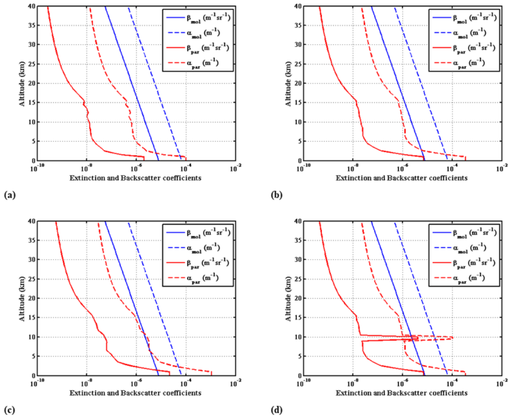
Figure 4. Backscatter and extinction coefficients vertical profiles at 355 nm used in the performance model. (a) RMA lower quartile, (b) RMA median, (c) higher quartile, and (d) median plus cirrus.
