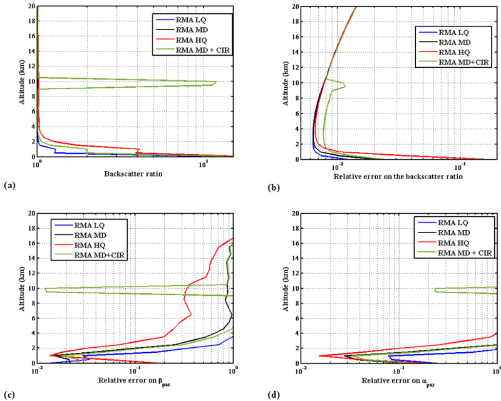
Figure 9. Actual scattering ratio. (a) Relative statistical error (standard deviation) on the scattering ratio measurement, (b) on the backscatter coefficient, (c) and on the extinction coefficient (d) for LQ, MD, HQ, and MD plus cirrus backscatter profiles.
