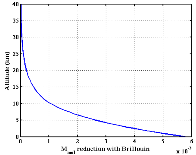
Figure D1. Reduction in M_{mol} caused by the Brillouin effect.
