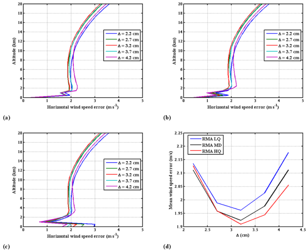
Figure 6. (a, b, c) Horizontal wind speed (HLOS) statistical error as a function of altitude for OPD for lower quartile, median, and higher quartile RMA aerosols distribution, respectively. (d) Wind speed error averaged between 0.5 and 15 km in altitude as a function of OPD.
