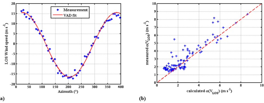
Figure C1. (a) LOS wind speed retrieved by HSRD-LNG over 100 shots at an altitude of 7.9 km. (b) Comparison of the measured and calculated LOS wind speed ( V_{LOS} ) errors.
