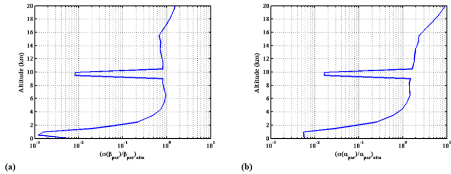
Figure 10. Relative standard deviation on \beta_{\text{par}} (a) and on \alpha_{\text{par}} (b) for the MD plus CIR backscatter coefficient distribution caused by uncertainties of 2 K in the atmospheric analysis as a function of altitude.
