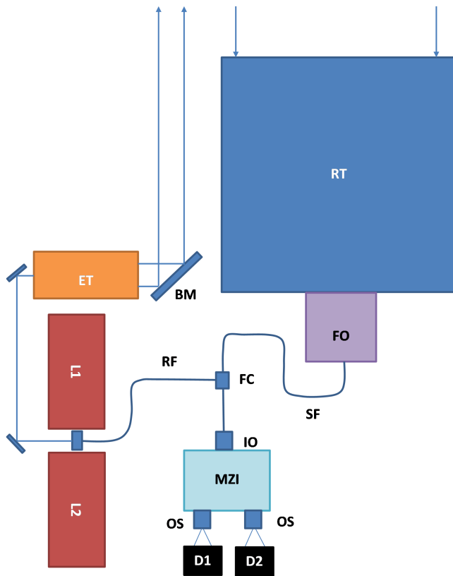
Figure 1. Diagram of the lidar system. L1 and L2 – lasers (nominal and redundant); ET – emission telescope; BM – boresight mirror; RT – receiver telescope; FO – front optic (including background filter); SF – signal fiber; RF – reference fiber; FC – fiber coupler and mode scrambler; IO – input optic; MZI – Mach-Zehnder interferometer; OS – output separation optic; D1 and D2 – A-CCD detectors.
