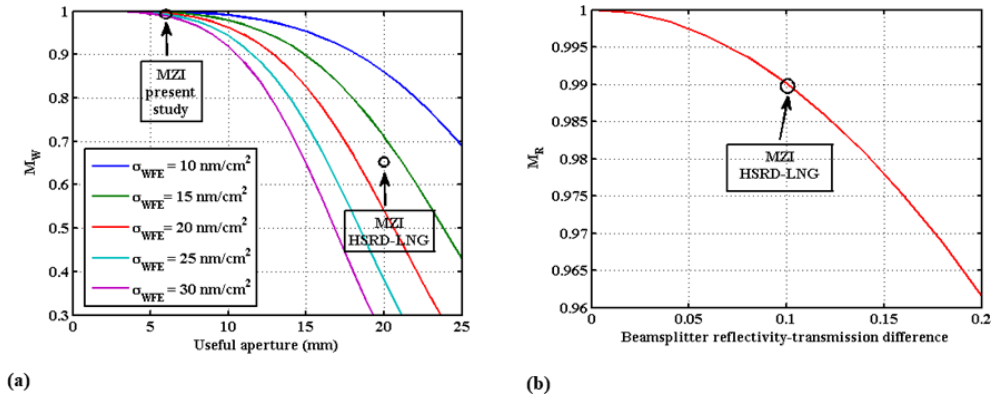
Figure 3. (a) Instrumental modulation factor M_W as a function of MZI useful aperture for different RMS WFE. The dots represent the MZI of the present study and the actual MZI of HSRD-LNG. (b) Instrumental modulation factor M_R as a function of the beam splitter R - T difference.
