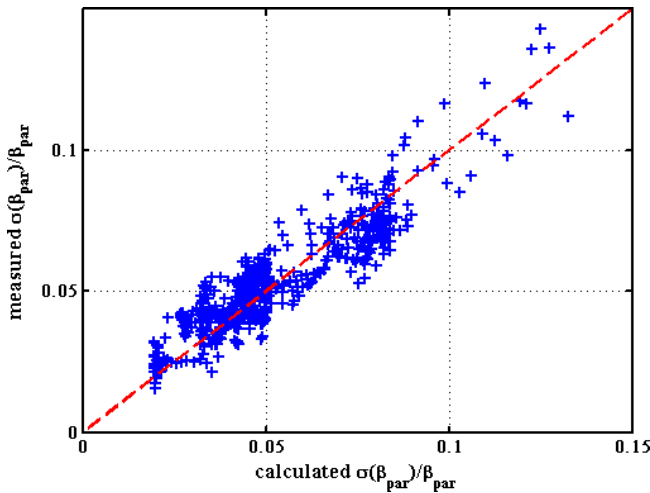
Figure C3. Comparison of the measured and calculated relative errors (standard deviation) on the particle backscatter coefficient.
