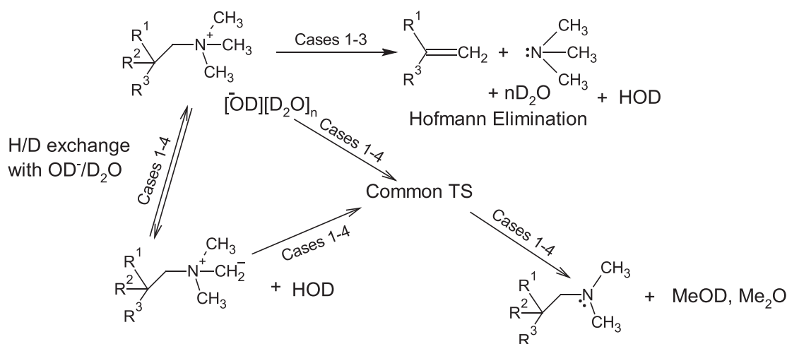
FIG. 1. Thermal decomposition of alkyltrimethylammonium deuteriooxide, adapted from Edson et al. (2012). Case 1: R^1 , R^2 , and R^3 = H ; Case 2: R^1 = CH_3 , R^2 , and R^3 = H ; Case 3: R^2 = H , R^1 , and R^3 = CH_3 ; Case 4: R^1 , R^2 , and R^3 = CH_3 . TS, transition state.
