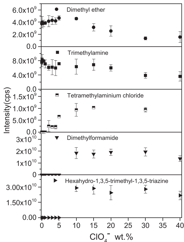
FIG. 9. The effect of \text{Ca}(\text{ClO}_4)_2 on the pyrolysis products of TMAH at a heating rate of 35^\circ\text{C}\cdot\text{min}^{-1} from 50^\circ\text{C} to 600^\circ\text{C} .
