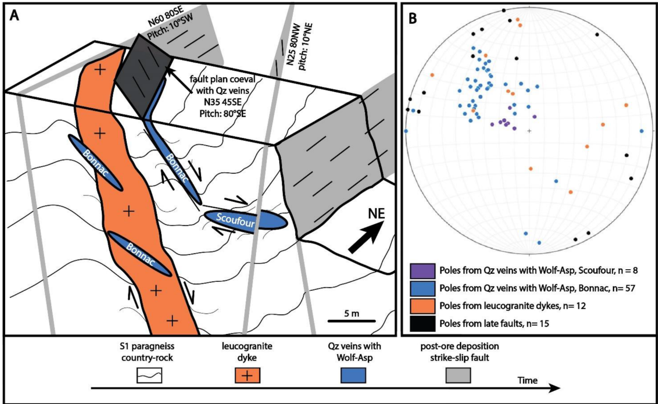
Fig. 7. (A) 3D block showing the main structural observations made on the mineralized quartz veins from Bonnac area. They allow us to propose a relative chronology of the structures developed in the paragneissic host-rock, the leucogranitic dykes and the quartz veins. (B) Stereogram (lower hemisphere projection) of the poles of the fault planes coeval with the emplacement of the mineralized veins, leucogranitic dykes, and late faults measured in the field.
