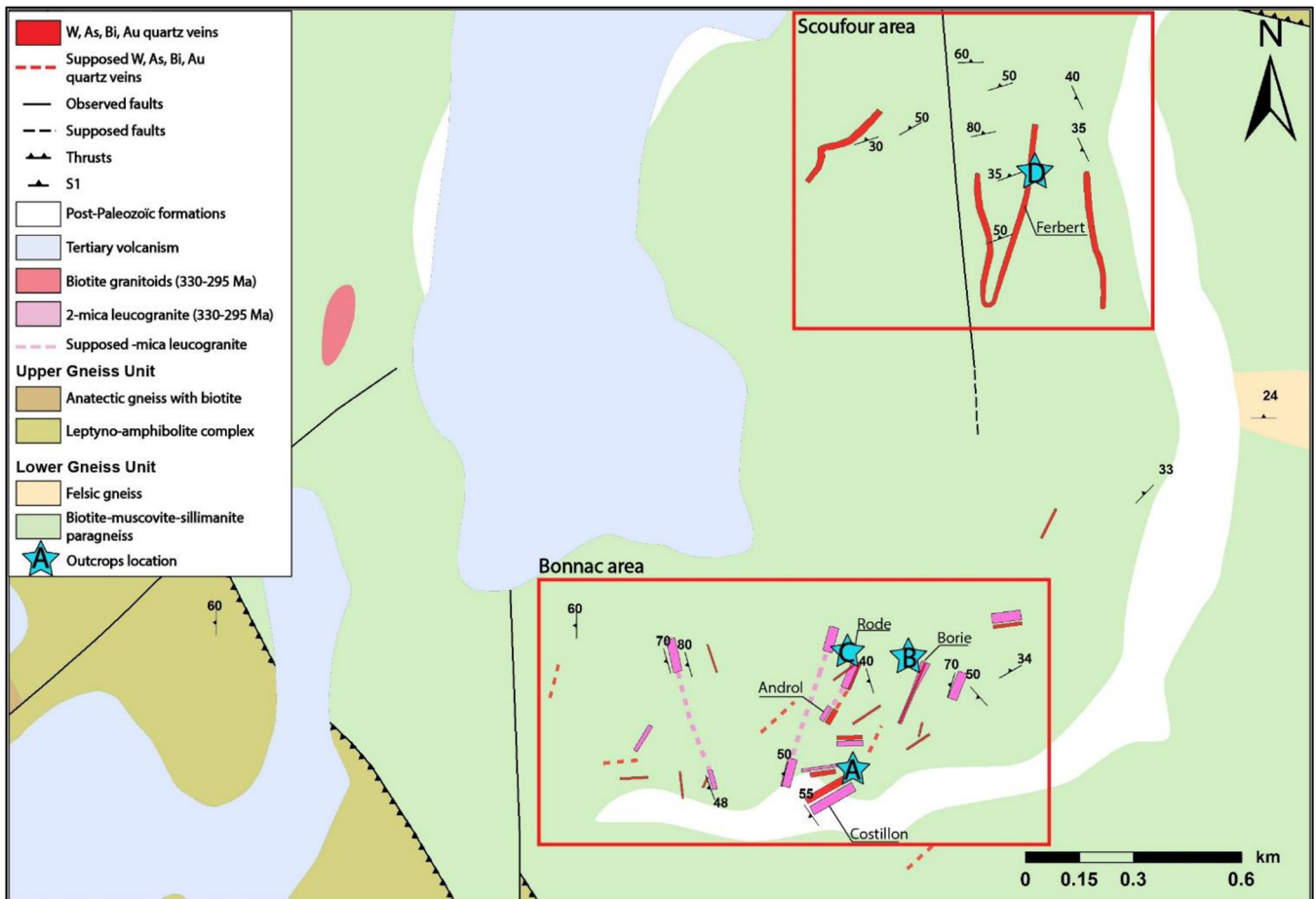
Fig. 3. Geological and structural map of the Bonnacc area with the location of most interesting outcrops.
