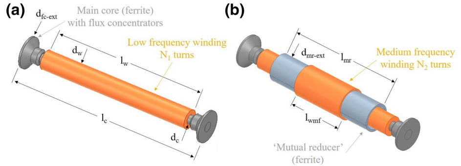
Figure 5. Characteristics of the (a) single band and (b) double band search-coil antennas.
