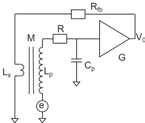
Figure 4. Equivalent circuit of the search-coil antenna and the preamplifier.
