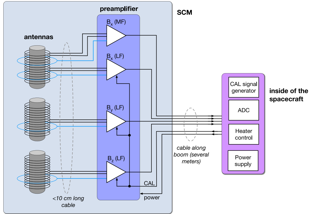
Figure 3. Block diagram of the SCM. The detailed processing of the preamplifier output somewhat differs for Solar Orbiter and for Parker Solar Probe.
