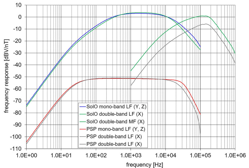
Figure 9. SCM transfer functions (gain) in dBV/nT for the instrument on Solar Orbiter and on Parker Solar Probe.
