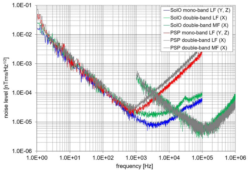
Figure 10. Noise level for the instrument on Solar Orbiter (blue) and on Parker Solar Probe (red).
