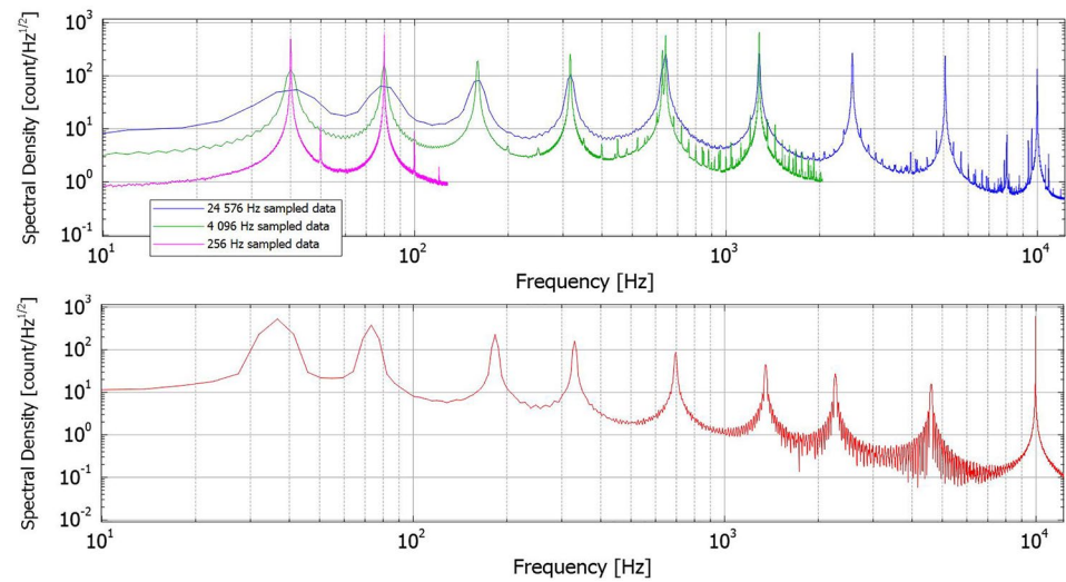
Figure 11. Response of the SCM to the on-board calibration stimulus sampled by the data analyzers LFR on Solar Orbiter (top) and DFB on Parker Solar Probe (bottom).
