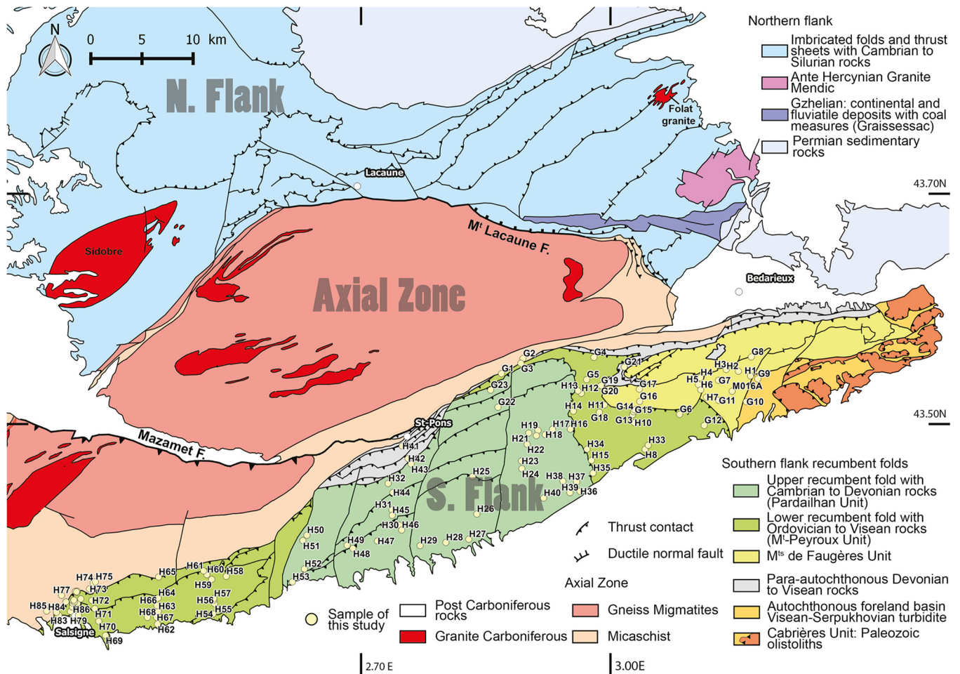
Fig. 2. Simplified structural map of the Montagne Noire showing the granite-migmatite dome of the Axial Zone, and the sedimentary northern and southern flanks (modified from Gèze, 1949; Arthaud, 1970; Faure et al. , 2010). The recumbent folding in the south area is coeval with the sedimentation in the Visean-Serpukhovian basin. The stratigraphy presents a reverse order in most part of these series. The figure was made from the vectorised map 250 000 of Montpellier by the BRGM (Berger et al. , 2001).
