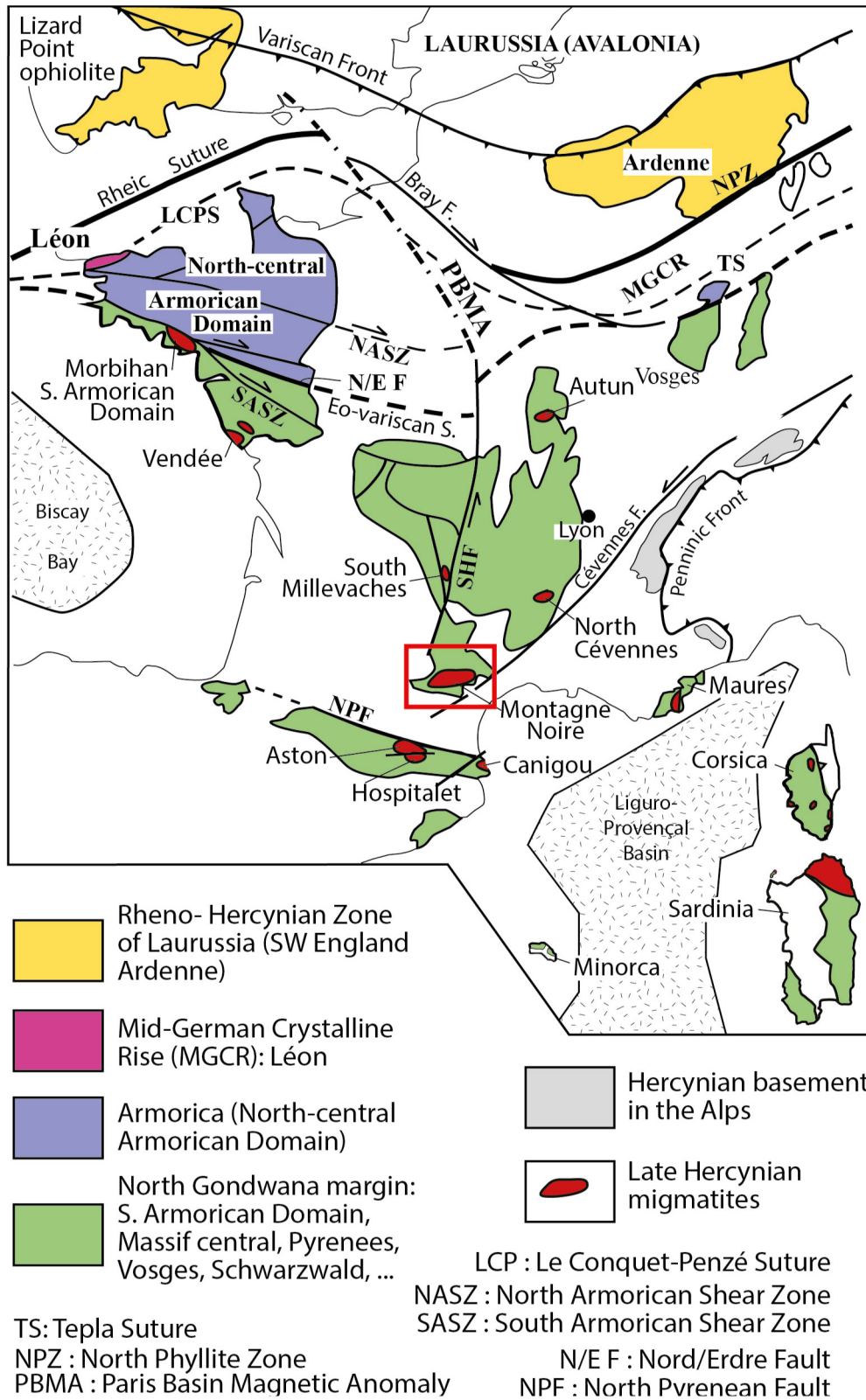
Fig. 1. Variscan massifs map with location of the Visean-Serpukhovian migmatites. The red rectangle represents the study area (modified from Faure et al. , 2010).
