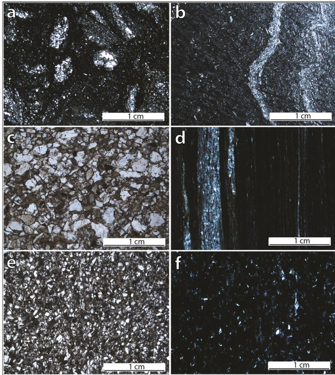
Fig. 6. Thin sections observed with optical microscope in polarized non-analysed light showing the lithology diversity, (a). Mudstone in the Visean Turbidite (sample G8), (b). Siltstone in the Early Ordovician rocks (sample G1), (c). Early Cambrian green sandstone (Marcory formation, sample H32), (d). Mudstone in the Early Ordovician rocks (sample G2), (e). Middle Cambrian fine-grained sandstone (sample H22), (f). Early Ordovician mudstone (sample G3).
