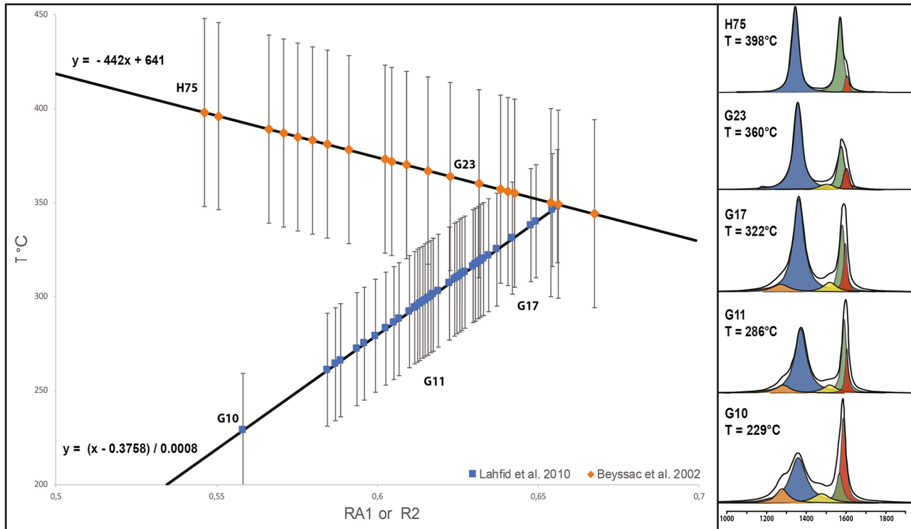
Fig. 7. Graph showing the repartition of our data with respect to the two methods used. The right column shows the evolution of the spectra aspect and the deconvolution chosen with D1 band (blue), D2 band (red), D3 band (yellow), D4 band (orange) and G band (green).
