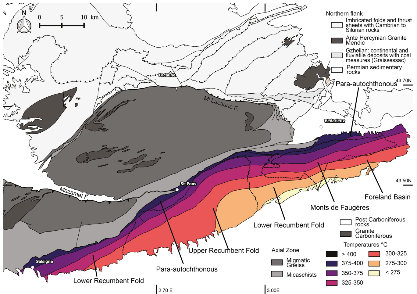
Fig. 10. Temperature map determined by the RSCM Tmax results of this study. The isotherms crosscut the tectonic units of the southern flank. Roughly, the temperature decreases from the NW to the SE away from the Axial Zone dome. The isotherms cut the micaschists between Salsigne and St-Pons because of a lack of data.
