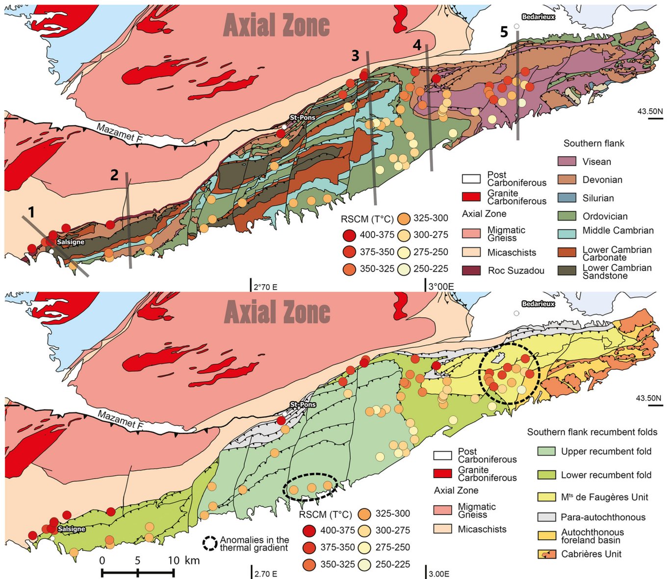
Fig. 8. Geological map of the Montagne Noire with the Tmax measured in the southern flank. Totally, 72 samples from the recumbent folds and turbiditic basin have been analysed by the RSCM method in the present study.
