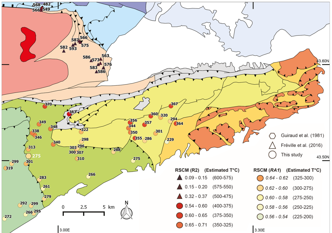
Fig. 11. Comparison of temperatures in °C acquired via RSCM method in this study and Fréville et al. (2016) and Guiraud et al. (1981) temperature from fluid inclusion.
