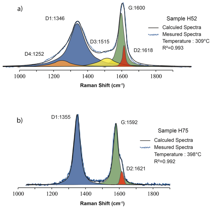
Fig. 5. Peakfitting of samples H52 (a), and H75 (b) by low temperature (Lahfid et al. , 2010) and high temperature method (Beysac et al. , 2002), respectively.
