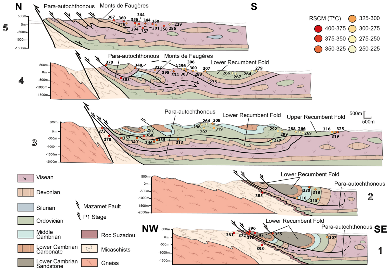
Fig. 9. Projections of the analyzed samples on five cross sections (located in Fig. 8) of the southern flank of the Montagne Noire. Temperatures are globally increasing toward the Axial Zone dome.
