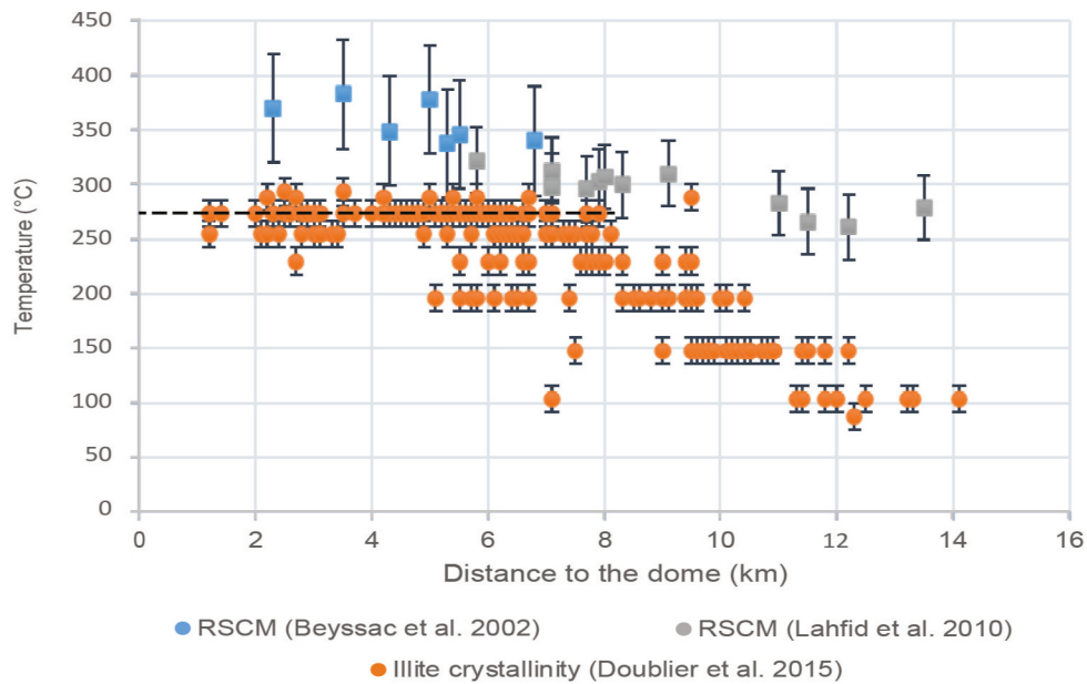
Fig. 14. Plot of the variation of measured temperatures using different methods with respect to the distance to the dome.
