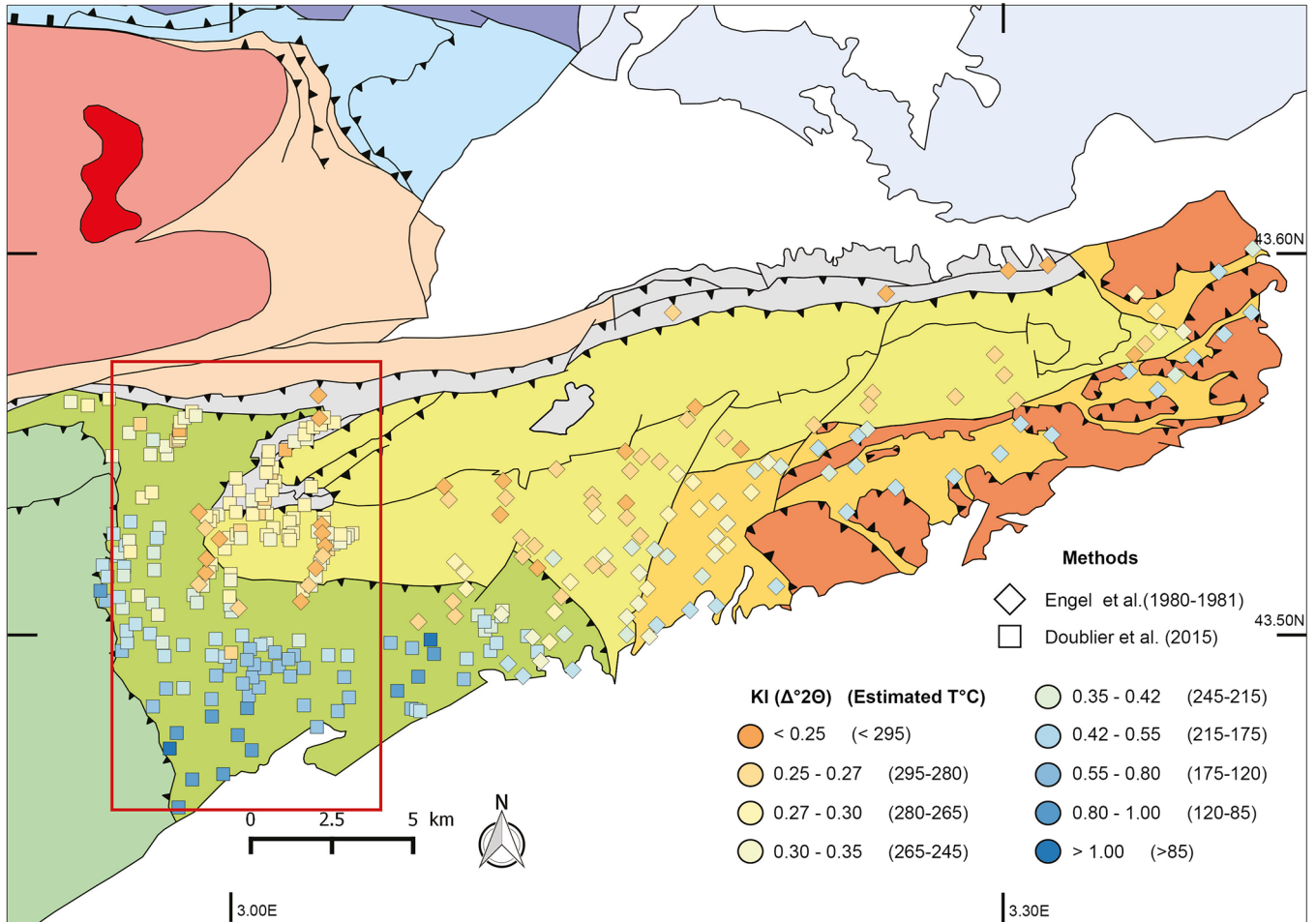
Fig. 12. Illite crystallinity data from previous studies (Engel et al. , 1981; Doublier et al. , 2015) based on the crystalline organization of illite analysed via X-ray diffraction converted from the Kübler index into °C (Merriman and Frey, 1999; Zhu et al. , 2016). The Figure 14 is based on the data from the red rectangle.
