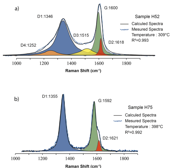
Fig. 5. Peakfitting of samples H52 (a), and H75 (b) by low temperature (Lahfid et al. , 2010) and high temperature method (Beyssac et al. , 2002), respectively.
