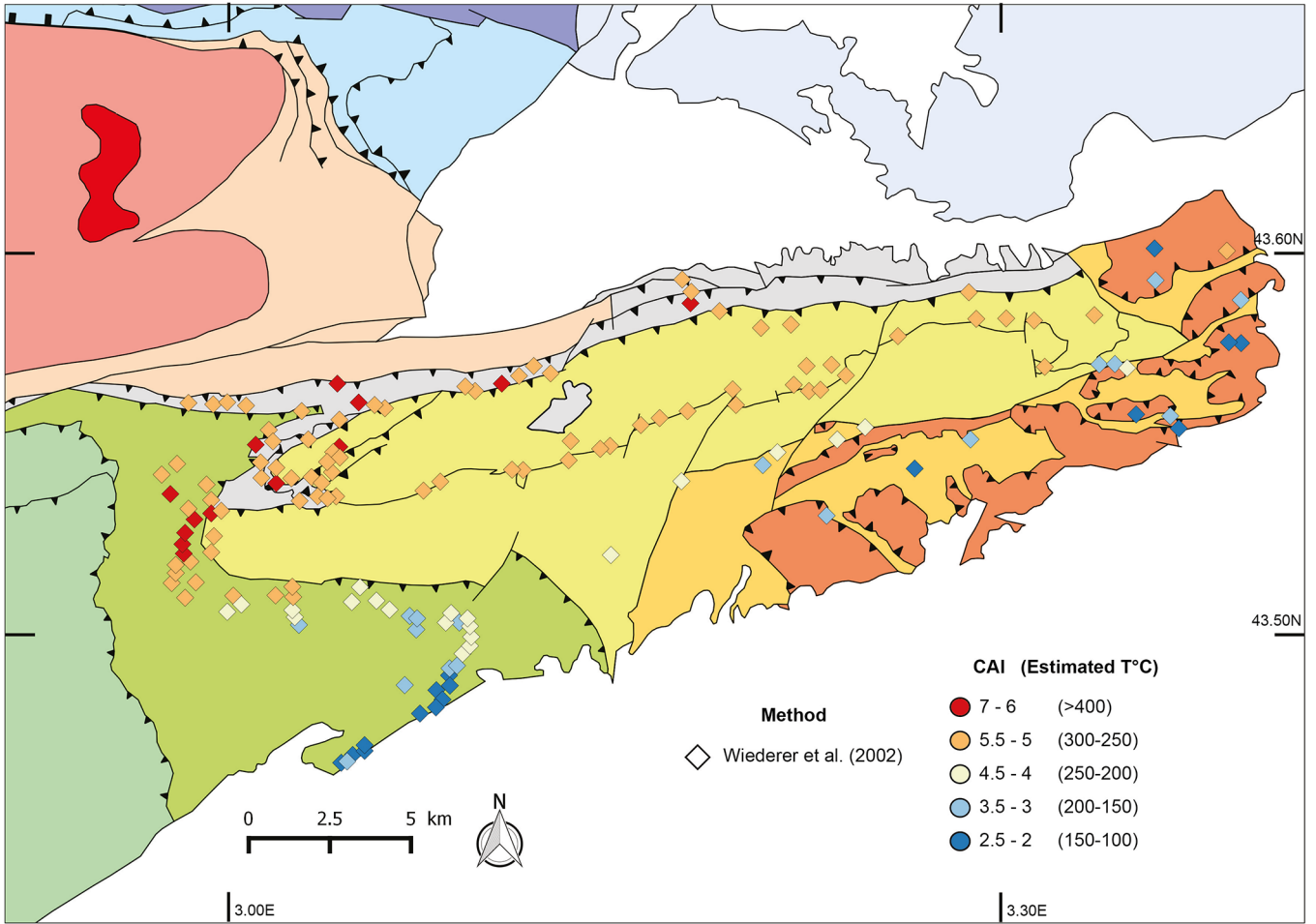
Fig. 13. Conodont alteration index method from previous study (Wiederer et al. , 2002). The colour of apatite crystals indicates its metamorphic degree. Wiederer et al. (2002) have studied more than three hundred conodonts.
