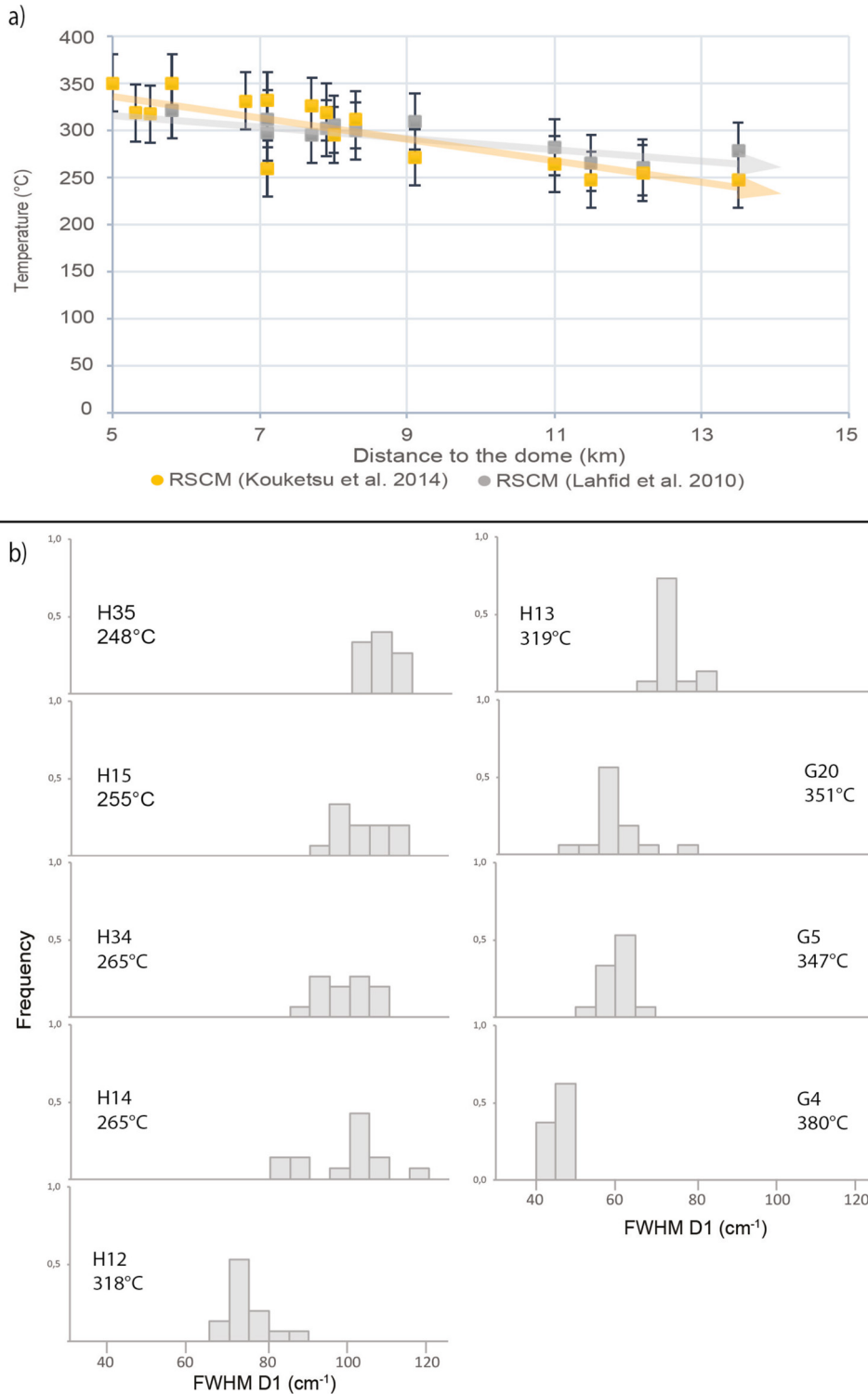
Fig. 15. (a) Comparison of Lahfid et al. (2010) and Kouketsu et al. (2014) thermometers, arrows represent the major linear trends. (b) Histograms of frequencies of the full width at half maximum of the band D1 (FWHM) acquired using the Kouketsu et al. (2014) method.
