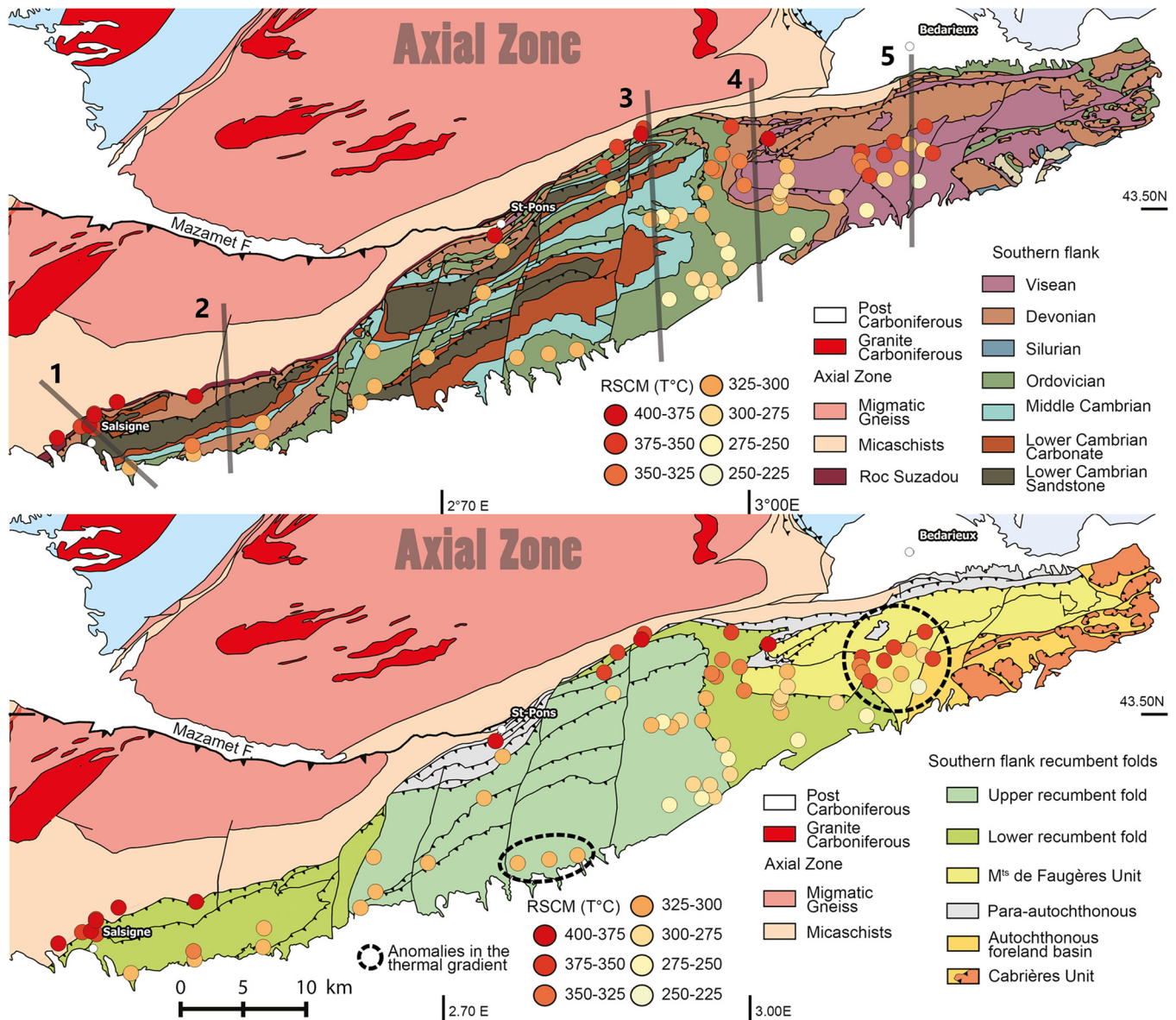
Fig. 8. Geological map of the Montagne Noire with the T_{max} measured in the southern flank. Totally, 72 samples from the recumbent folds and turbiditic basin have been analysed by the RSCM method in the present study.
