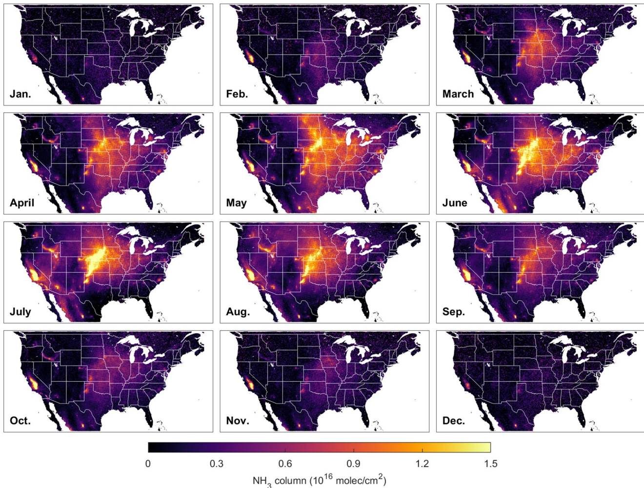
Figure 2. IASI 2008–2017 oversampled \text{NH}_3 column concentration over CONUS from January to December.
