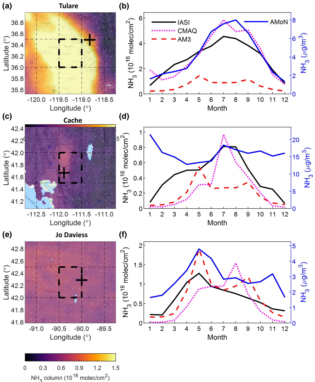
Figure 4. Comparison of \text{NH}_3 seasonality in hotspots regions. Panels (a), (c), and (e) are the annual averaged IASI oversampled \text{NH}_3 column concentrations. The bold black dashed box indicates the selected hotspot regions. The black cross shows the nearby AMoN site. Black dashed lines represent AM3 grid boxes, and white dots represent the center of CMAQ grids. (b), (d), and (f) are the \text{NH}_3 seasonality derived from the IASI oversampling \text{NH}_3 column, CMAQ, and AM3 modeled \text{NH}_3 columns (left axis), and AMoN \text{NH}_3 concentration (right axis). Map data from Google Earth.
