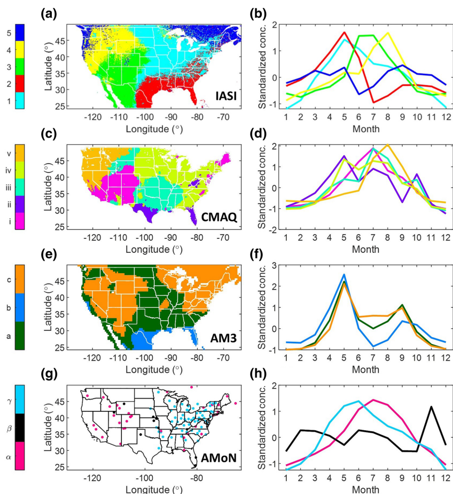
Figure 3. IASI, CMAQ, AM3, and AMoN \text{NH}_3 seasonality clusters map (a), (c), (e), and (g) and standardized \text{NH}_3 concentrations for each cluster (b), (d), (f), and (h).
