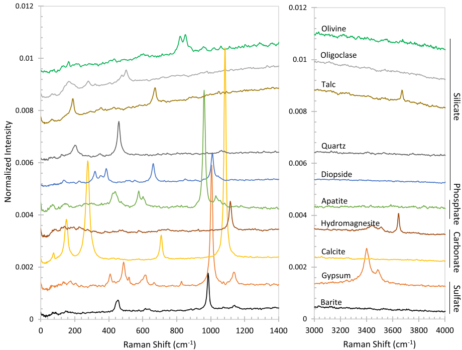
Fig. 46 Raman spectra of pure minerals taken using the FM BU and EQM MU. Spectra are averages from 100 laser pulses taken with a delay of 650 ns, a gate width of 100 ns, and a gain of 3200. Laser energy was measured at \sim 8 mJ. The distance was 2.77 m. The talc is from an unknown locality while the apatite is from Durango, Mexico, the diopside from Tanzania, the oligoclase from Ontario, Canada, the gypsum from Durango, Mexico, the quartz from Minas Gerais, Brazil, the calcite from Mato Grosso do Sul, Brazil, the barite from Cumbria, UK, the hydromagnesite from Iran, and the olivine from San Carlos, AZ, USA. Spectra of the oligoclase, olivine, and talc have been multiplied by 4 to enlarge the peaks
