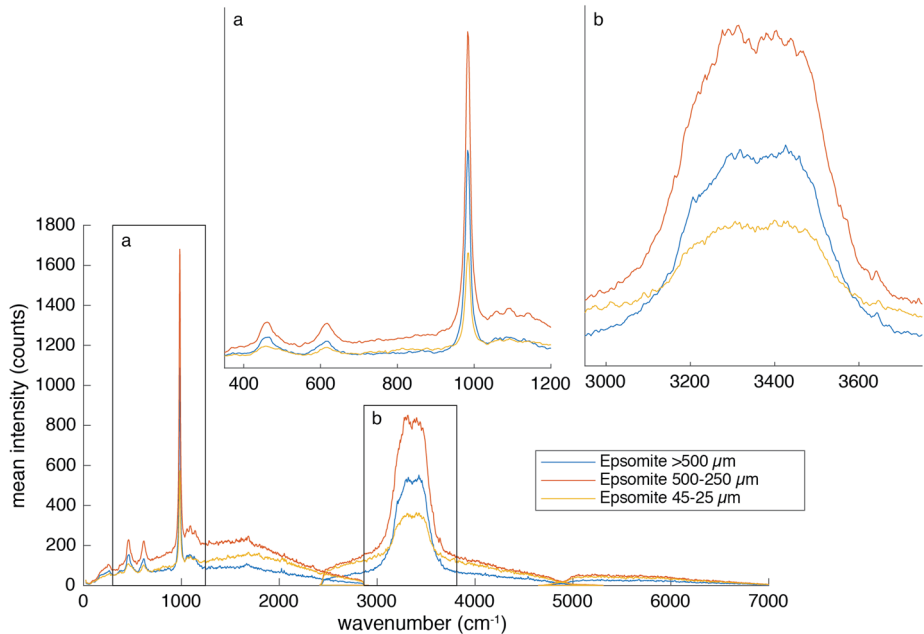
Fig. 48 SuperCam Raman spectra of pressed-powder pellets of different grain sizes of epsomite, observed with the EQM at 2.25 m distance integrating 100 laser pulses. Wavenumbers are approximate. Insets show closer detail of the fingerprint (a) and water regions (b) of the spectrum
