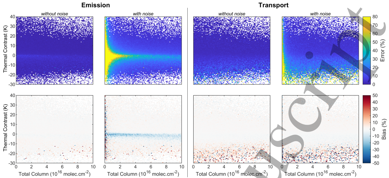
Figure A3. Performance evaluation (top: error, bottom: bias, both in %) of the emission network (left four panels) and transport network (right four panels), with and without adding noise. Note that compared to the evaluation plots in [53], the median value is shown in each grid box, which removes the effect of outliers and allows us to better assess the real performance of the network.
