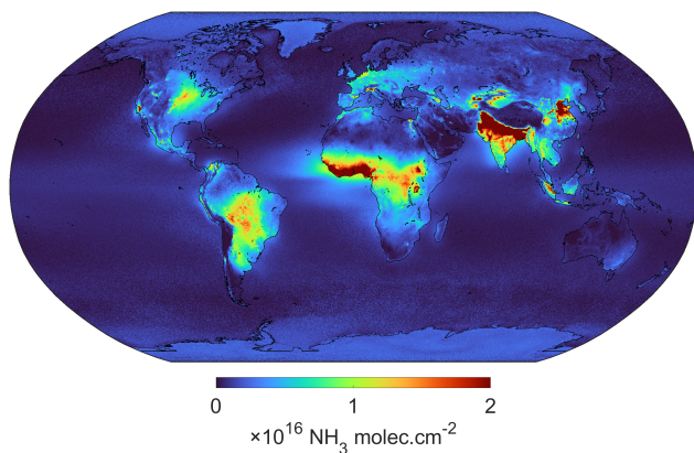
Figure 1. IASI-NH 3 total columns distribution (molec.cm -2 ) averaged from 11 years of IASI/Metop-A measurements (1 September 2008 to 31 December 2018, morning overpasses, ANNI-NH 3 -v3R-ERA5 dataset) on a 0.5° × 0.5° grid.
