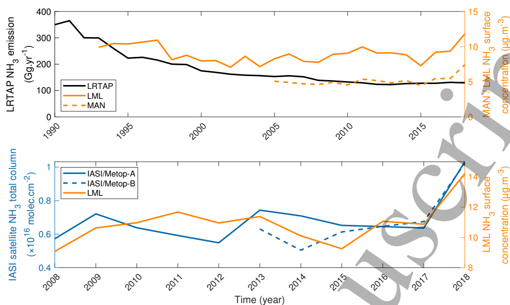
Figure 4. (top) Yearly timeseries of NH 3 emissions reported for the Netherlands in the framework of the Gothenburg Protocol (1990–2018, Gg.yr -1 , black), NH 3 surface concentrations from the LML (1993–2018, μg.m -3 , orange) and from the MAN network (2005–2018, μg.m -3 , dashed orange). 27 MAN stations (6, 8, 9, 11, 12, 20, 21, 23, 32, 35, 39, 45, 46, 54, 58, 61, 63, 65, 68, 84, 87, 88, 121, 122, 130, 131, 990) and 8 LML stations (131, 235, 444, 538, 633, 722, 738, 929) have been considered. (Bottom) Yearly NH 3 time-series for the Netherlands measured by IASI (molec.cm -2 , blue) and at the surface by ground-based instruments from the Dutch National Air Quality Monitoring Network (LML) (μg.m -3 , orange). Only the LML stations with data coverage over the entire 2008–2018 period have been used (stations 131, 444, 538, 633, 738).
