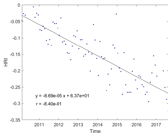
Figure A2. HRI (no unit) monthly time series over a remote location in the Pacific Ocean. The linear regression is indicated in black.
