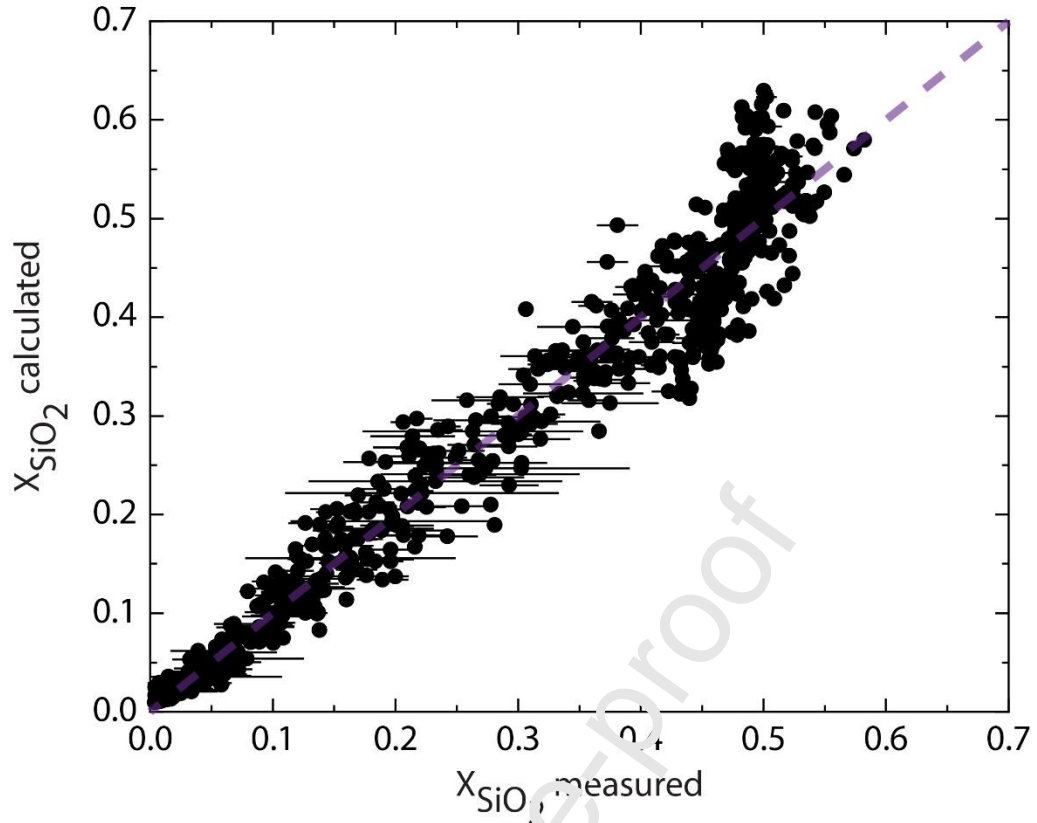
Fig. 3. Comparison of the molar fraction of \text{SiO}_2 in melt calculated with MAGLAB to that from the experimental database. The relative deviation of MAGLAB calculations, taken as \frac{|x_{\text{SiO}_2}^{\text{Melt, calculated}} - x_{\text{SiO}_2}^{\text{Melt, measured}}|}{x_{\text{SiO}_2}^{\text{Melt, measured}}} , is \sim 15\% on average.
