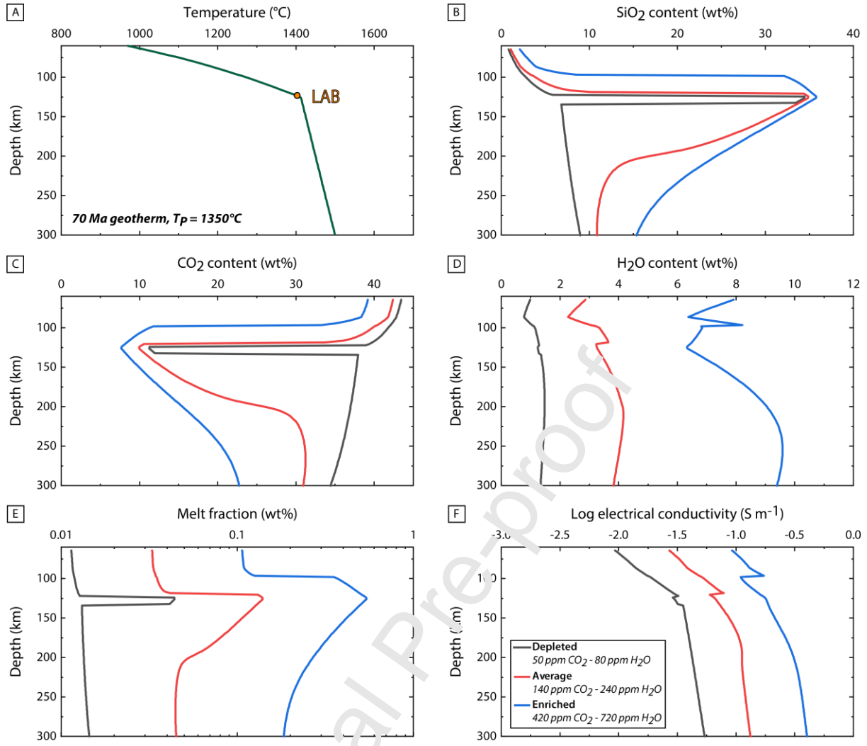
Fig. 7: MAGLAB equilibrium melt composition, melt fraction and electrical conductivity for oceanic upper mantle at 70 Ma with various volatile contents (50 wt ppm \text{CO}_2 – 80 wt ppm \text{H}_2\text{O} , 140 wt ppm \text{CO}_2 – 240 wt ppm \text{H}_2\text{O} , and 420 wt ppm \text{CO}_2 – 720 wt ppm \text{H}_2\text{O} ) as a function of depth. (A) Mantle thermal structure with potential temperature T_P = 1350^\circ\text{C} from Grose and Afonso (2013) (G13R1350 model). (B) \text{SiO}_2 , (C) \text{CO}_2 , and (D) \text{H}_2\text{O} contents of melts. (E) Melt fraction. (F) Bulk mantle electrical conductivity. The orange circle in panel (A) provide an estimation of the LAB depth.
