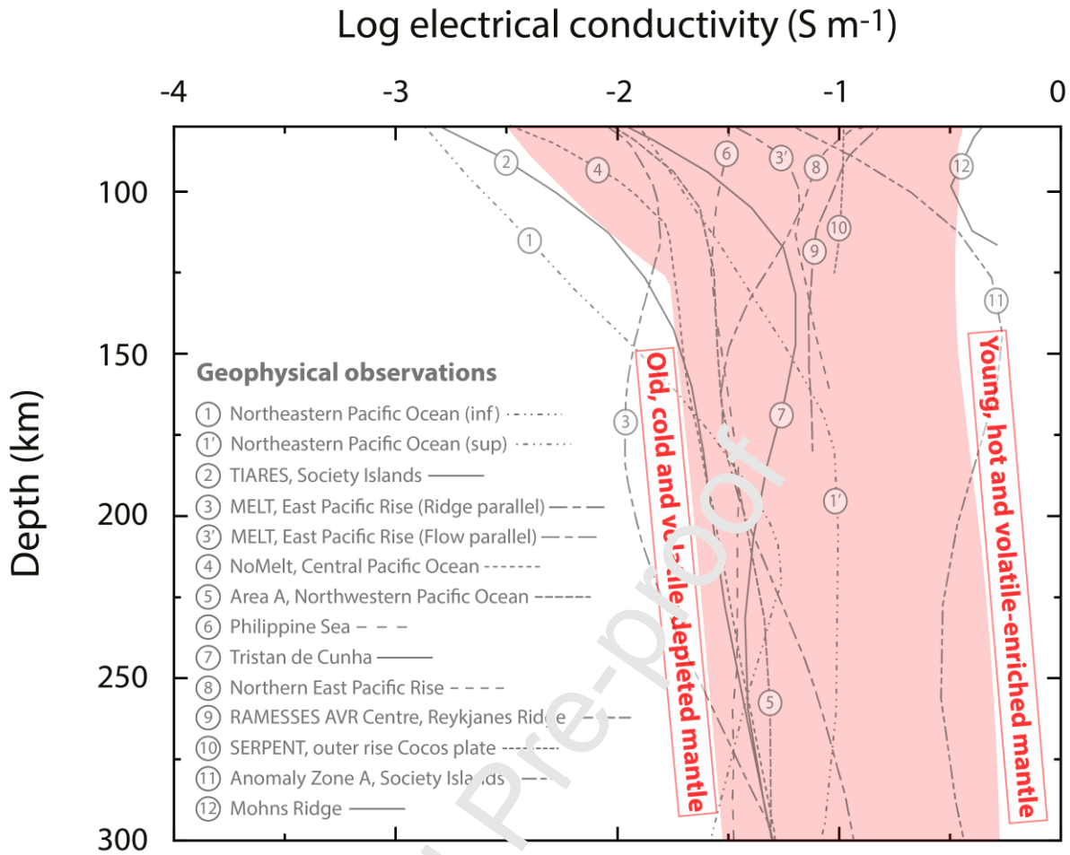
Fig. 11: Comparison between electrical profiles observed beneath various ocean floors and MAGLAB simulations. MAGLAB conductivities for partially molten peridotite rocks (light red area) range from (i) old, cold and highly depleted mantle (130 Ma, with T_P = 1300^\circ\text{C} and 20 wt ppm \text{CO}_2 – 50 wt ppm \text{H}_2\text{O} ) to (ii) young, hot and highly enriched mantle (0 Ma, with T_P = 1450^\circ\text{C} and 100 wt ppm \text{CO}_2 – 720 wt ppm \text{H}_2\text{O} ). The mantle thermal structures are G13R1300 and G13R1450 models from Grose and Afonso (2013) , with T_P = 1300^\circ\text{C} and 1450^\circ\text{C} , respectively. Electrical conductivity profiles of the oceanic upper mantle in dark grey are from various magnetotelluric studies. 1 and 1', conductivity profile in the northeastern Pacific Ocean between Hawaii and California ( Lizarralde et al., 1995 ). 2, Tomographic Investigation by seafloor ARray Experiment for the Society hotspot (TIARES) profile representing the ‘background’ mantle beneath the Society hotspot in the Pacific Ocean ( Tada et al., 2016 ). 3 and 3', Mantle Electromagnetic and Tomography (MELT) profile in the region of the East Pacific Rise ( Evans et al., 2005; Baba et al., 2006 ). 4, conductivity profile in the central Pacific Ocean (“NoMelt” experiment in Sarafian et al., 2015 ). 5, conductivity profile in the northwestern Pacific Ocean (“Area A” in Baba et al., 2013, 2017b ). 6, conductivity profile beneath the Philippine Sea ( Baba et al., 2010 ). 7, conductivity profile beneath the Tristan da Cunha hotspot in the southern Atlantic Ocean ( Baba et al., 2017a ). 8, conductivity profile in the northern East Pacific Rise ( Key et al., 2013 ). 9, Reykjanes Axial Melt Experiment: Structural Synthesis from Electromagnetics and Seismics (RAMESSES) profile in the northern section of the Mid-Atlantic Ridge, i.e. the Reykjanes Ridge (“AVR Centre” in Heinson et al., 2000 ). 10, Serpentinite, Extension, and Regional Porosity Experiment across the Nicaragua Trench (SERPENT) profile beneath the outer rise of 22-24 Ma Cocos plate seafloor in the Pacific Ocean ( Naif et al., 2013; Naif, 2018 ). 11, conductivity
