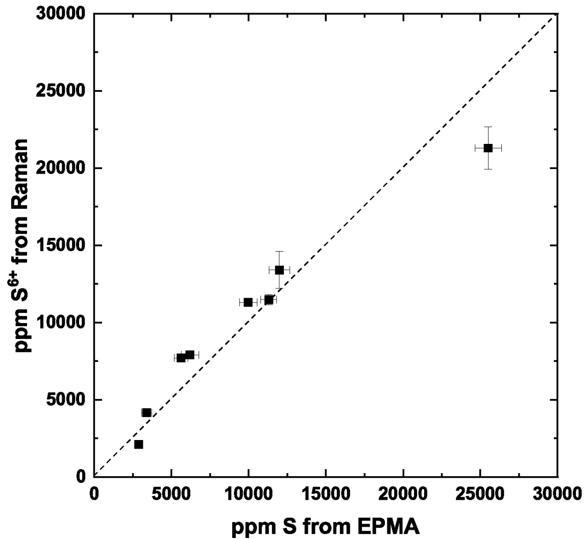
Fig. 2 S content determined by Raman spectroscopy (ppm S^{6+} ) and the calibration of Morizet et al. (2017b) from the Raman spectrum simulations (see Fig. 2) as a function of S content determined by EPMA. The reported errors are the ones in Table 1 and obtained from standard deviation of the replicated analyses.
