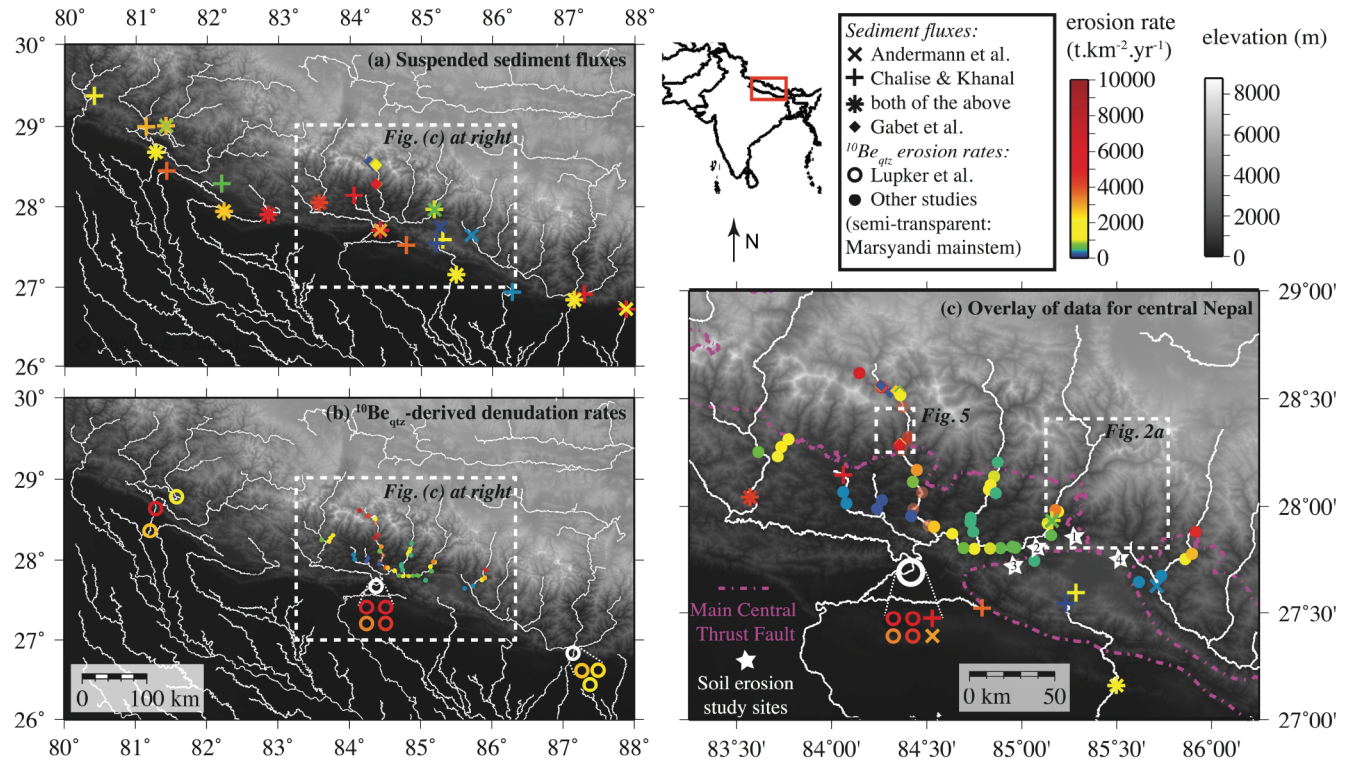
Figure 1. Map of Nepal showing erosion rate data collected in previous studies. Grayscale background shows elevation from SRTM digital elevation map at \sim 90 m resolution. Data points are color-coded by erosion rate. (a) Sediment fluxes from Chalise and Khamal (1997) and Andermann et al. (2012), with overlain symbols representing sites with data from both studies. (b) Denudation rates determined from ^{10}\text{Be}_{\text{qtz}} from Godard et al. (2012), Godard et al. (2014), Lupker et al. (2012), and Wobus et al. (2005). White circles are expanded to show data collected from multiple times or grain sizes by Lupker et al. (2012). (c) Magnified scale of central Nepal region showing data from (a) and (b) along with location of several previous studies of agricultural soil erosion identified from published literature: (1) Likhu Khola (Gardner and Jenkins, 1995; location of this study), (2) Kulekhani (Upadhaya et al., 1991), (3) Pokhare Khola (Tiwari et al., 2008), and (4) Jhiku Khola and Kavre catchments (e.g., Merz, 2004).
