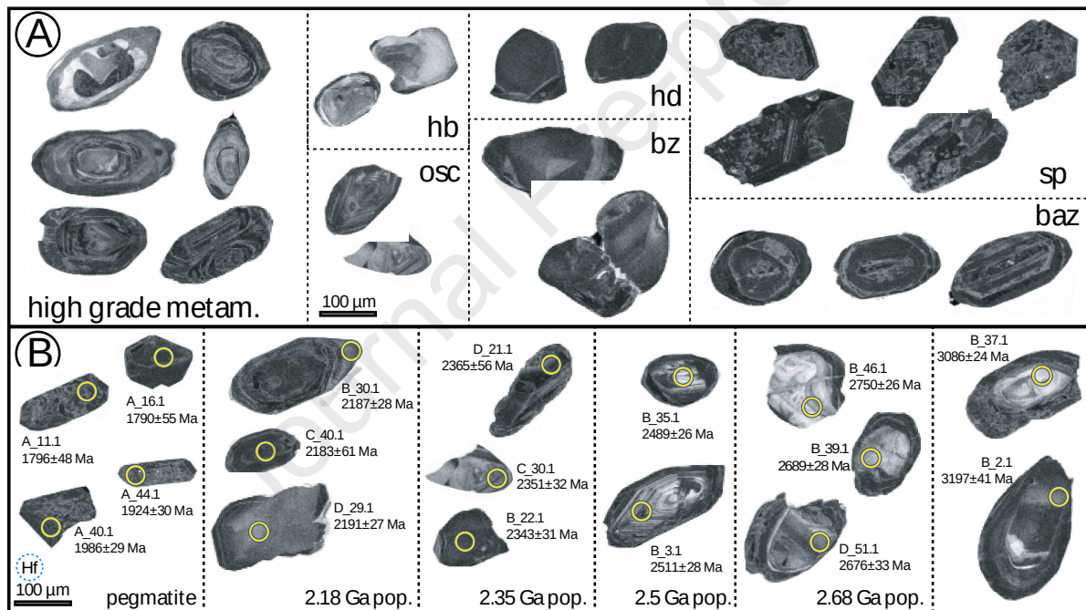
Figure 5: CL images of zircon grains from all samples, scaling is the same in A and B. (A) shows examples of the variety of different textures present in the samples. The grains in the left panel show very complex, often chaotic textures typical for high grade metamorphism and cores overprinted by zones of recrystallization or new growth, the others show examples of each classification (hb: homogeneous bright, hd: homogeneous dark, osc: oscillatory zoning, bz: broad zoning, sp: spongy/porous, baz: broad altered zoning). (B) shows highly concordant (intercept with Concordia) grains and ages of each age population. The circles show the 32 \mu\text{m} sized LA spots for the U-Pb analyses. Hf analyses were performed with 47 \mu\text{m} sized LA spots (dashed circle next to scale bar) in the same locations. The corresponding analytical data can be found in the electronic supplementary material.
