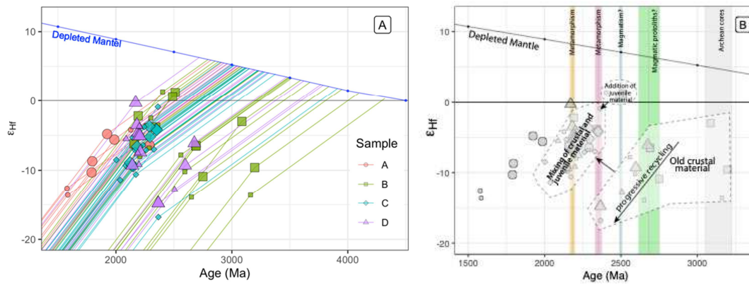
Figure 10: Representations of the Hafnium data of samples TRX – 04 A-D. (A): \epsilon_{\text{Hf}}(t_1) values as a function of time for the four samples (TRX-04A: red circles, TRX-04B: green squares, TRX-04C: blue diamond, TRX-04D: purple triangles). Big symbols correspond to concordant analyses with U-Pb ages intercepting the Concordia curve, small symbols correspond to analyses up to 10% discordant. \epsilon_{\text{Hf}}(t_1) is calculated from the measured ^{176}/^{177}\text{Hf} isotope ratio and the corresponding U-Pb age. The paths indicate the evolution of \epsilon_{\text{Hf}} as a function of time. The intercepts of these paths with the \epsilon_{\text{Hf}} composition of the depleted mantle (blue line and dots) indicate the Depleted Mantle model age T_{\text{DM}} . (B) shows the same data as A emphasizing the main zircon populations (vertical colored bars, colors and ages are as in Figure 9) and the proposed differentiation and mixing processes interpreted for the dataset. Symbols and sizes are as in (A).
