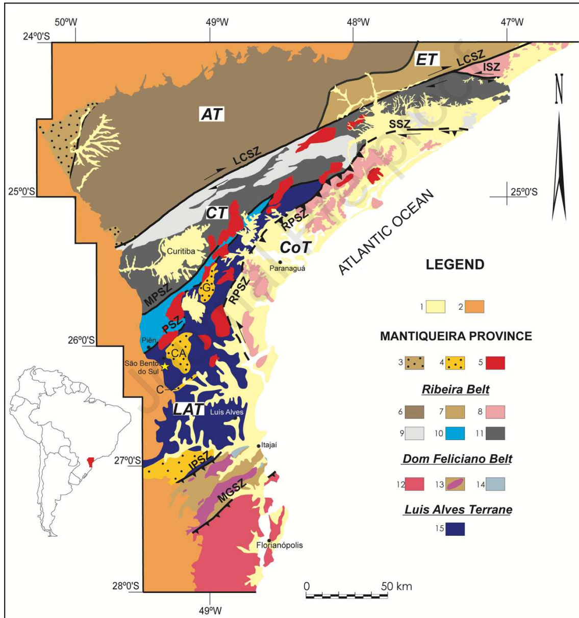
Fig. 1 –Tectonic and geological sketch of the south-southeast Brazilian Precambrian terranes with sampling location of sample TRX-04 (star). 1. Quaternary and Tertiary sediments; 2. Paraná Basin; 3. Eopaleozoic basins; 4. Neoproterozoic basins (CA: Campo Alegre; C: Corupá; G: Guaratubinha); 5. Graciosa/Serra do Mar Suite alkaline granites. Ribeira Belt : Apiaí Terrane (AT) : 6. Supracrustal and granitic rocks undifferentiated. Embu Terrane (ET) : 7. Orthogneisses, supracrustal and granitic rocks undifferentiated. Coastal Terrane (CoT) : 8. Metasedimentary Sequences and gneiss-granitic rocks of Paranaguá/Mongaguá Domains undifferentiated. Curituba Terrane (CT) : 9. Supracrustal rocks; 10. Piên Domain: calc-alkaline granitoids and mafic ultramafic suite; 11. Atuba-Registro Itatins Complexes. Dom Feliciano Belt : 12. Granitoid belt (Florianópolis Batholith); 13.
