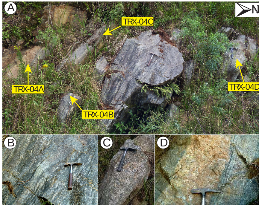
Fig. 2 – Field pictures of the sampled rocks. (A) Entire outcrop representative of the metamorphic units; the yellow arrows indicate the location of the collected samples. (B) orthogneiss in the center of the outcrop. Samples TRX-04B and TRX-04B are homogeneous, slightly broader felsic (TRX-04B) and mafic (TRX-04C) bands of this gneiss. (C) amphibolite lens, sample TRX-04D. (D) detail picture of the pegmatite, sample TRX-04A.
