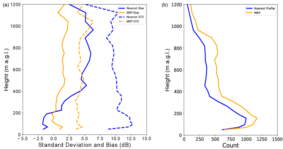
Figure 10. (a) The bias and standard deviation of observation–simulated radar reflectivity at SIRT A for the period 1 November 2018–19 February 2019. The statistics were calculated for instances when reflectivity was both observed and simulated at a given range gate at a given time. (b) The count of cells for which reflectivity was observed and simulated.
