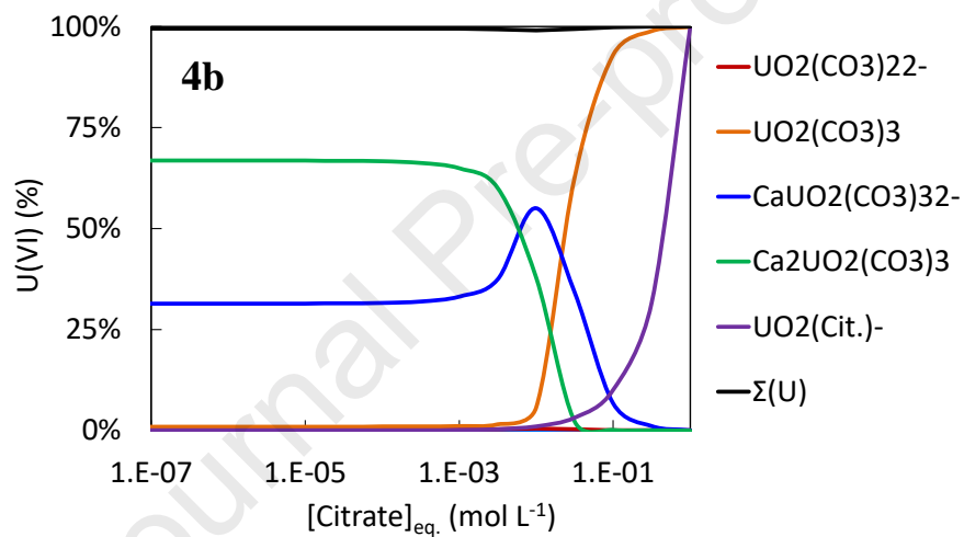
Fig. 4. Speciation of calcium (4a) and U(VI) (4b) in COx pore water
