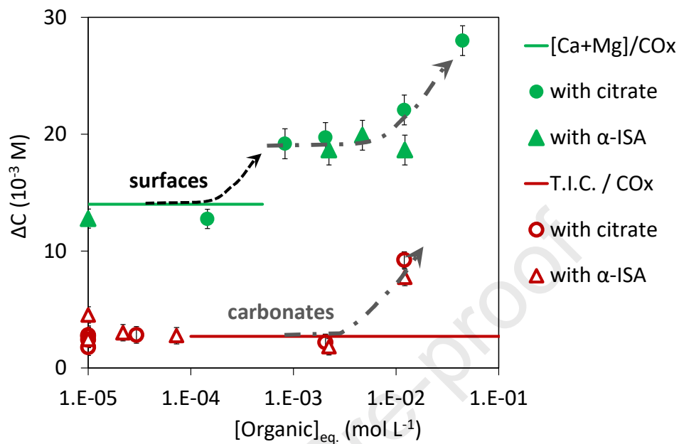
Fig. 5. Disturbance of carbonates chemistry in aqueous solution.
