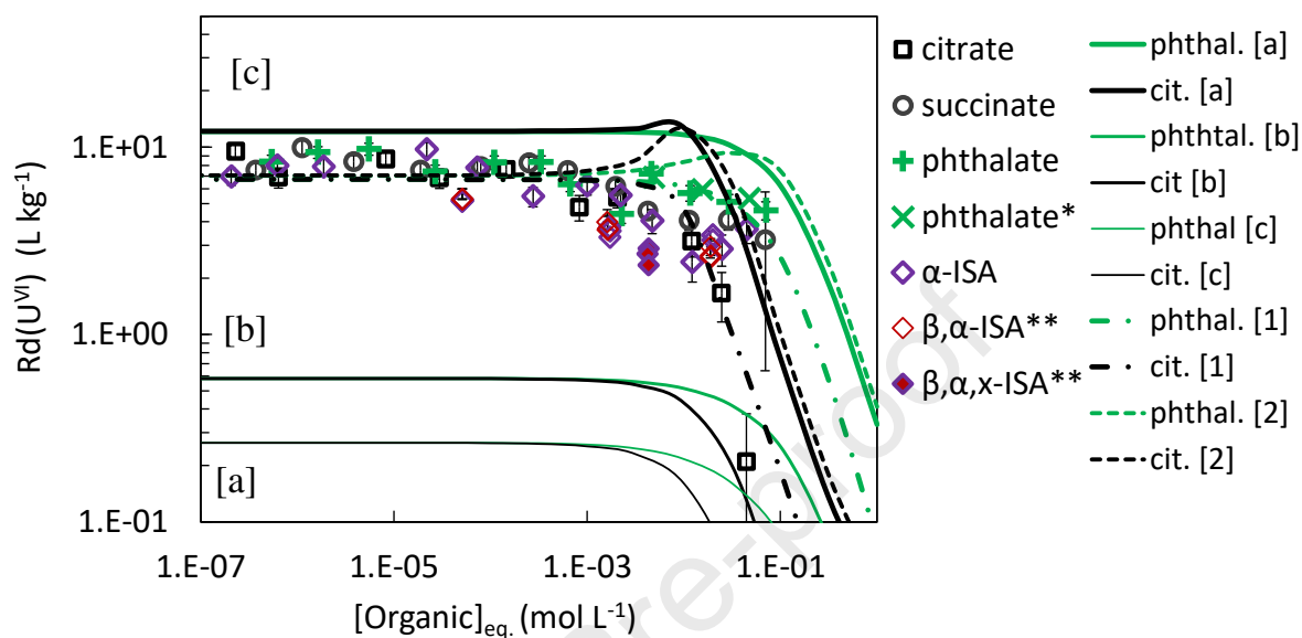
Fig. 3. Adsorption of U(VI) on COx clay rock as a function of concentration of various organic compounds at equilibrium with calcite.
