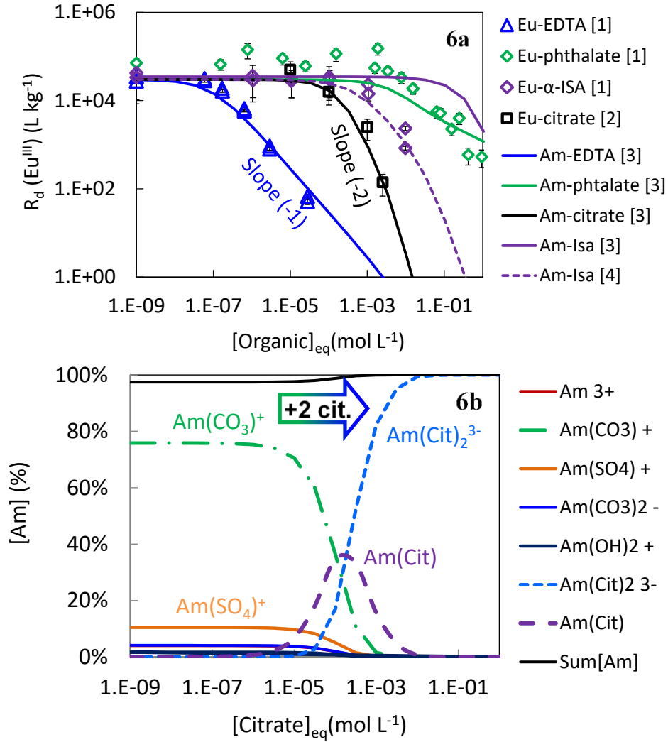
Fig. 6. (6a) Experimental Eu(III) sorption data (signs) compared to predictive model on Am(III) (solid lines). (6b) Speciation of americium in COx pore water as a function of citrate concentration. [1] This study [2] Schott et al., (2012) on Opalinus clay [3] Predictive model using Am(III) sorption data and ThermoChimie TDB. [4] Model with Am-ISA complexation constant adjusted by analogy with Eu-ISA (this work).
