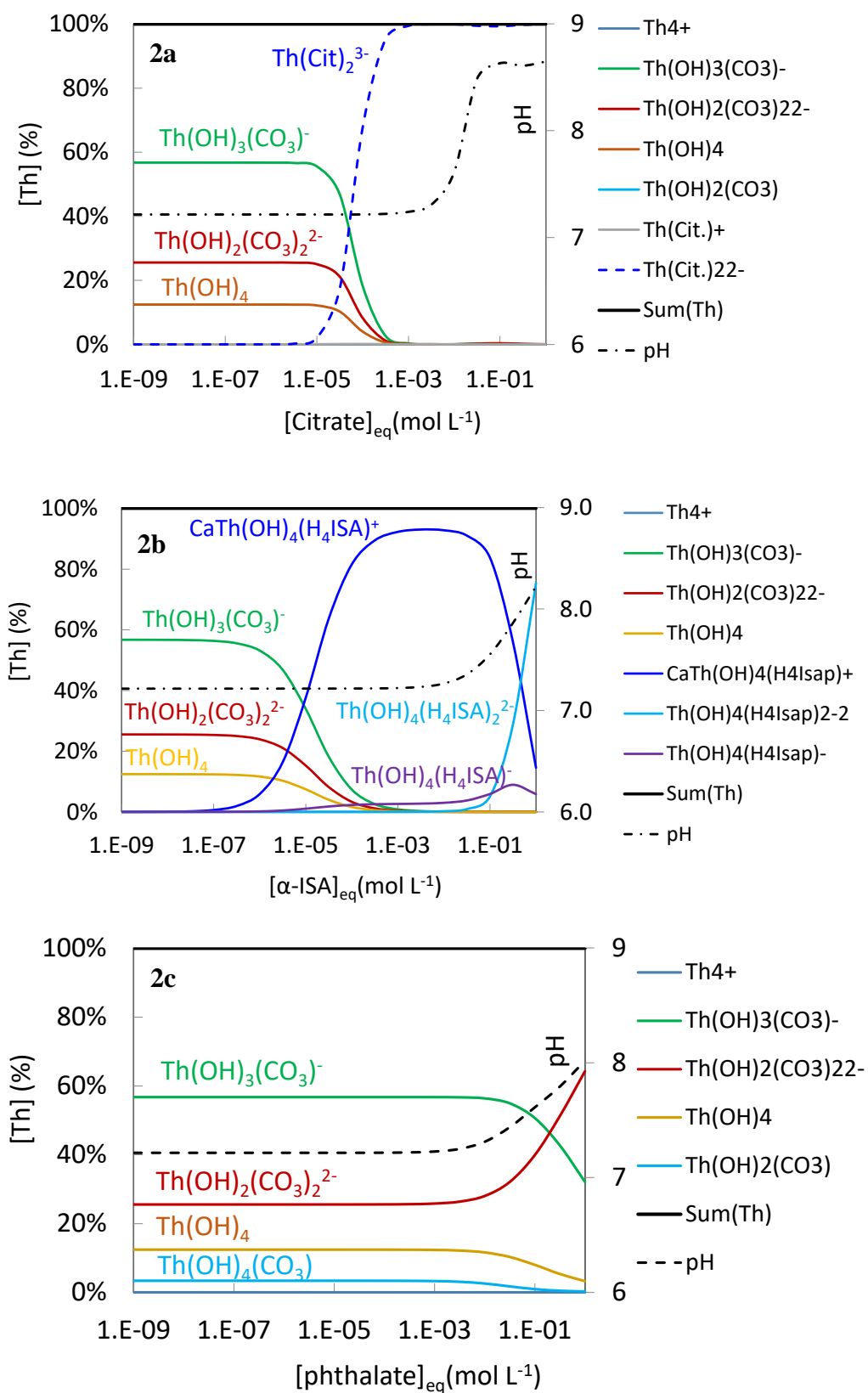
Fig. S2: Speciation of Th(IV) in COx clay rock at equilibrium with citrate (2a), \alpha -ISA (2b) or o-phthalate (2c). \text{pH}_0 \sim 7.2 , at equilibrium with calcite.
