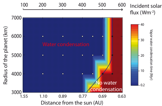
Fig. 1. Diagram showing condition for condensation of water vapor as a function of radius of the planet and solar flux. Color scale shows times at which condensation occurs. Time increases from blue to red.
